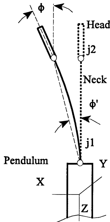
Figure 6. Head/Neck Pendulum Test Model
