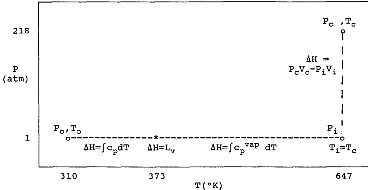
Fig. A1. Evaluation of enthalpy changes, \Delta H , in determination of q=\Delta E=\Delta H-\Delta(PV) . In addition to \Delta H , there is the overall \Delta(PV)=P_c V_c-P_o V_o . An expression for c_p^{\text{vap}} is given in Eq. (A2).
