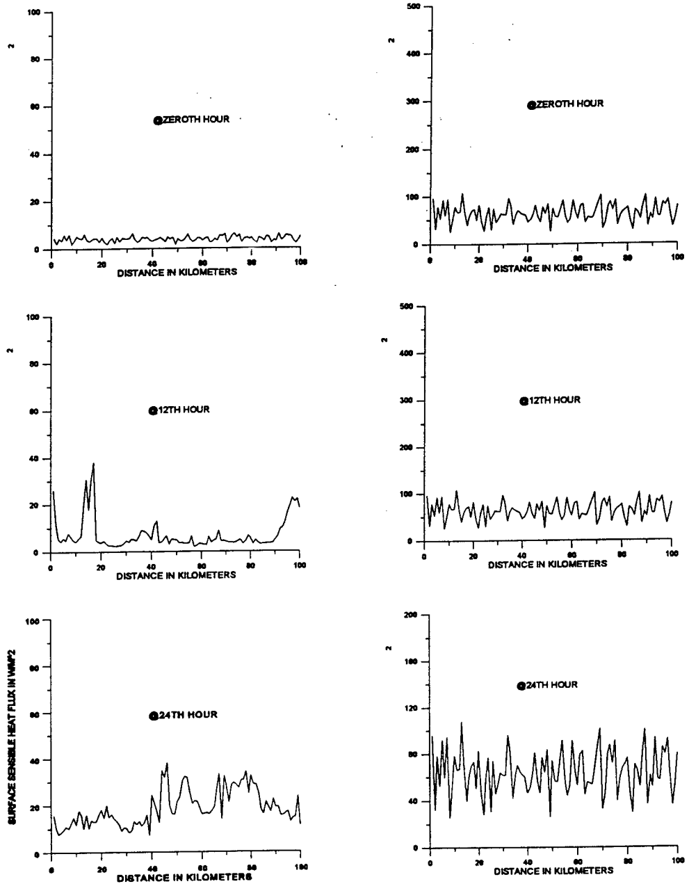
Fig. 13: Sea surface sensible and latent heat flux values
