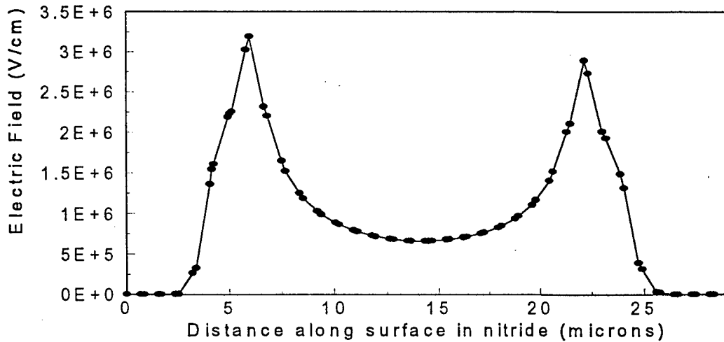
Fig.32 Electric Field in nitride for a RESURF dose of 7 \times 10^{12} /cm 2
