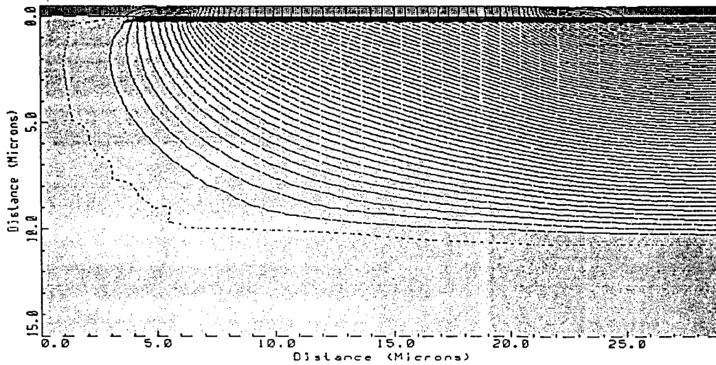
Fig 10 Potential Contours at breakdown for RESURF dose of 7 \times 10^{12} / \text{cm}^2
