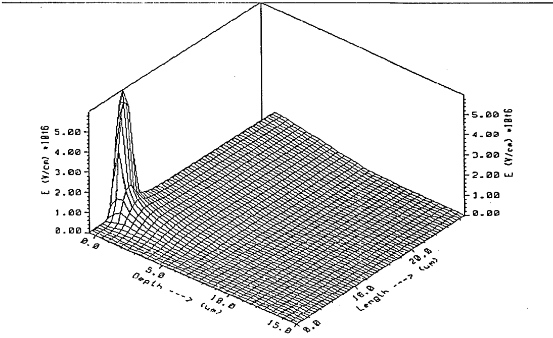
Fig 20 3-D Plot of the Electric field in the diode for a dose of 3 \times 10^{13} / \text{cm}^2
