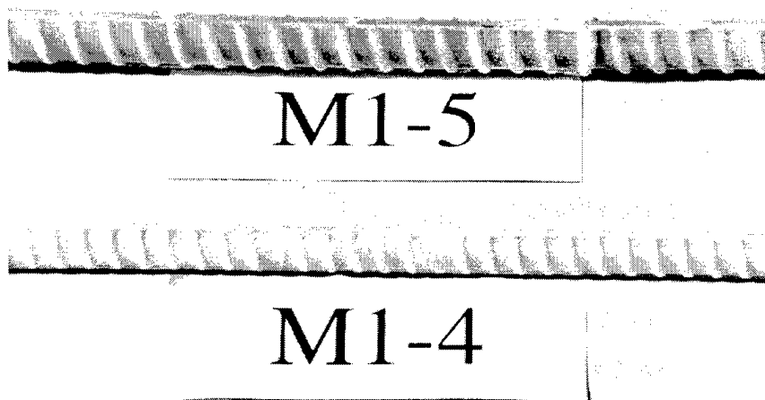
Figure 2.5 M1 GFRP Rebar
