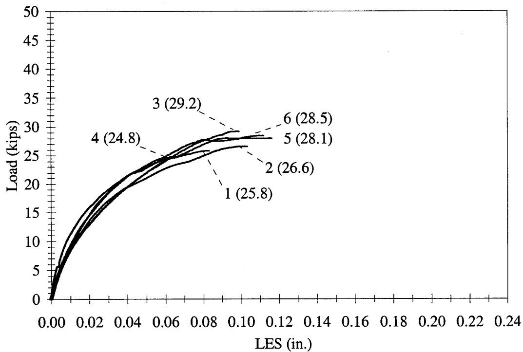
Figure 3.24 LES vs. Load, M2-6-2-15.0
