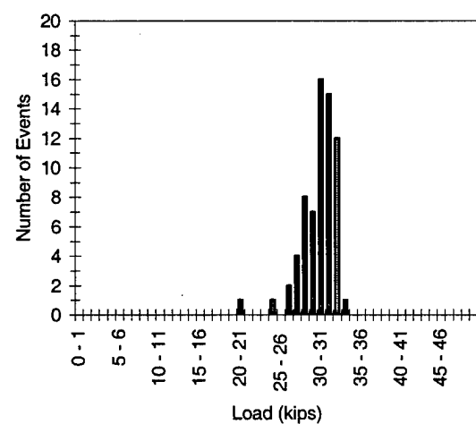
Figure F.54 2M2-6-2-47.0-3
