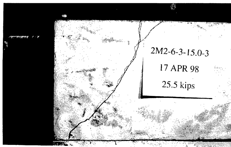
Figure 3.50 2M2-6-3-15.0-3 Side Photograph
