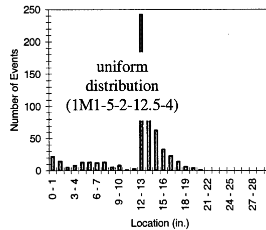
Figure 3.31 M1, C2 (concrete sensors) Distribution Patterns
