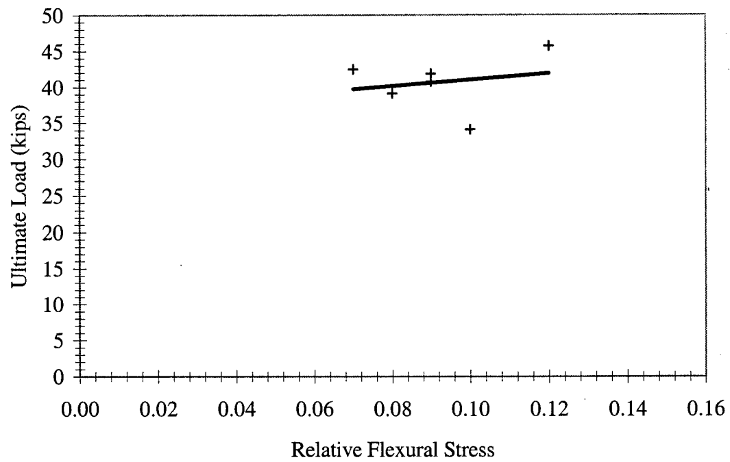
Figure 3.58 M2, Bond Test Relative Induced Flexural Stress
