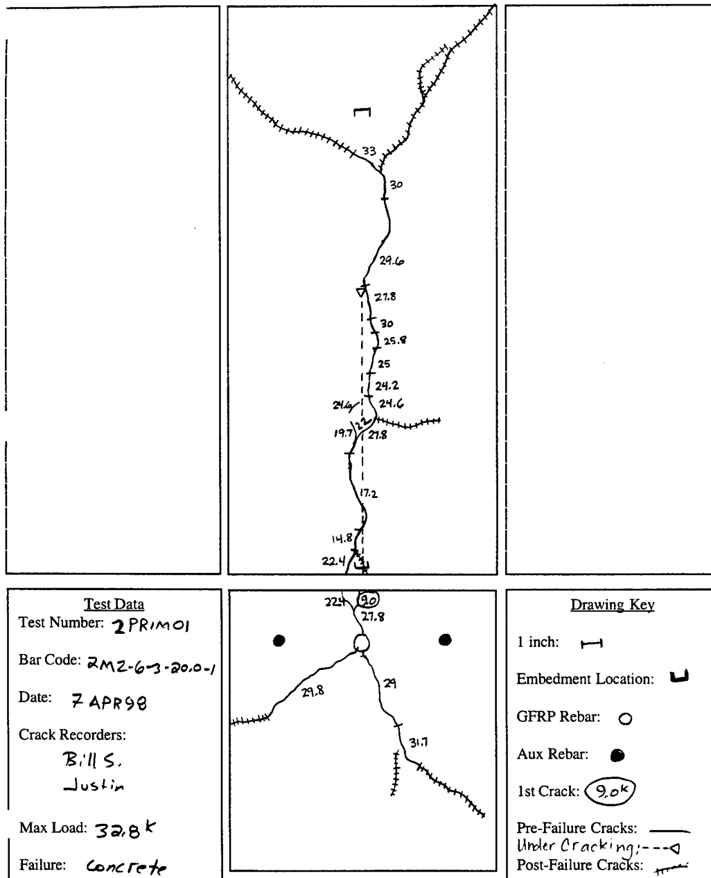
Figure E.40 2M2-6-3-20.0-1
