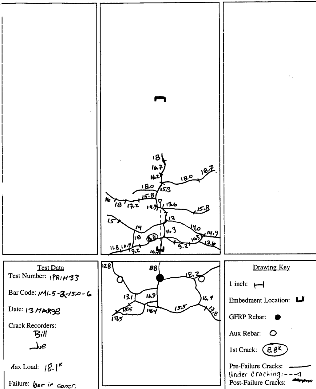
Figure E.30 1M1-5-2-15.0-6
