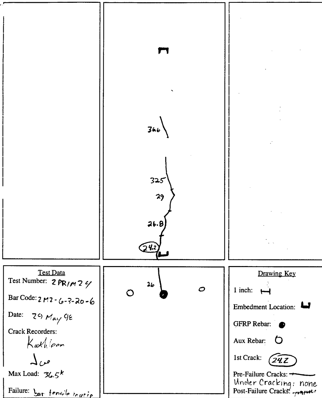
Figure E.45 2M2-6-3-20.0-6
