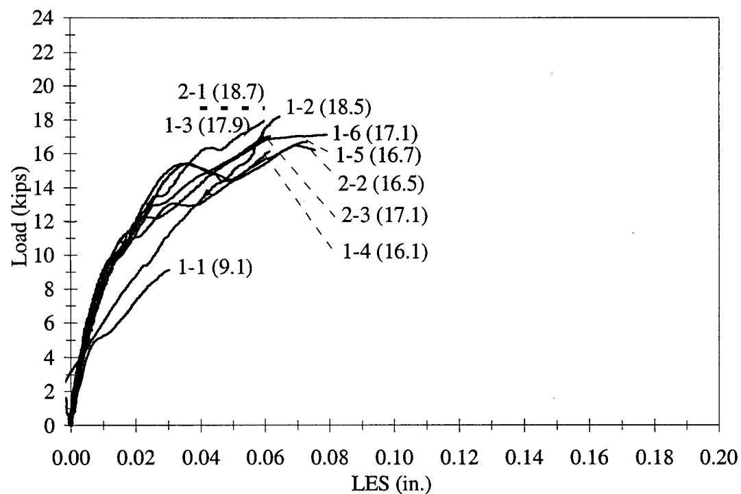
Figure 3.12 LES vs. Load, M1-5-2-12.5
