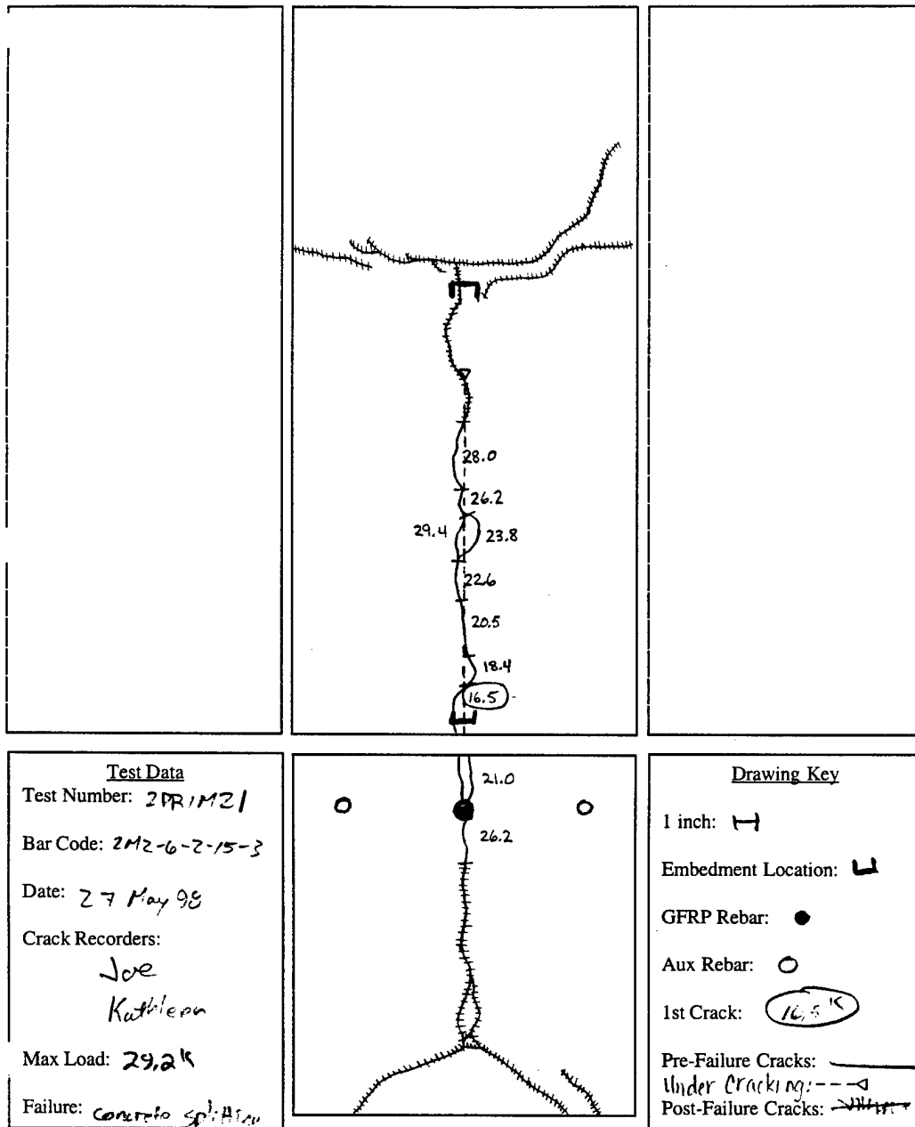
Figure E.69 2M2-6-2-15.0-3
