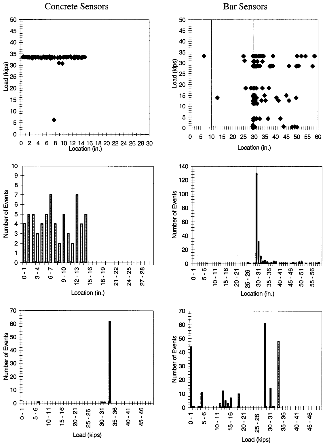
Figure F.43 2M2-6-3-20.0-4
