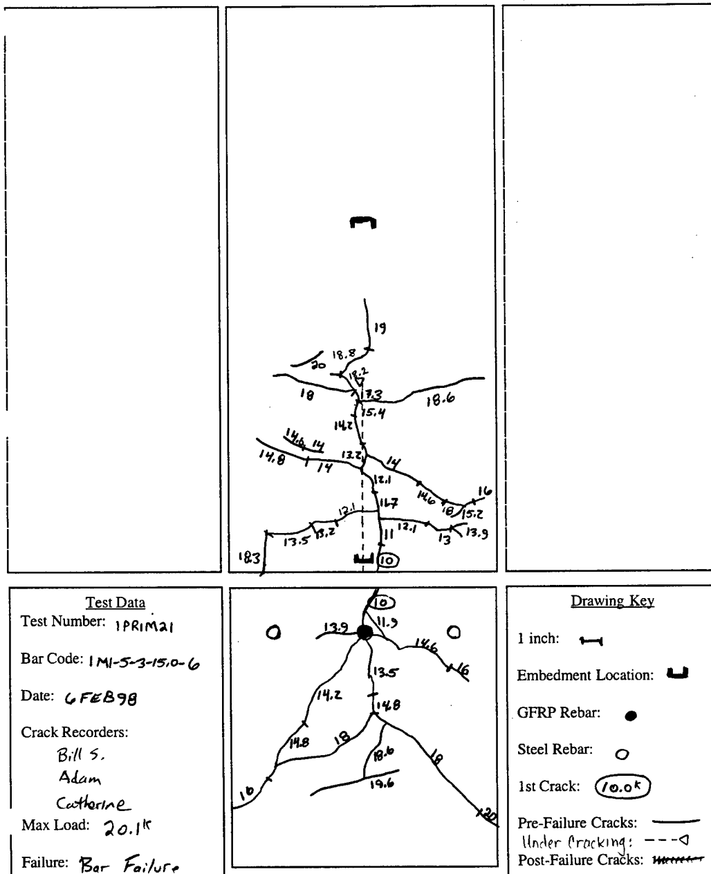
Figure E.6 1M1-5-3-15.0-6
