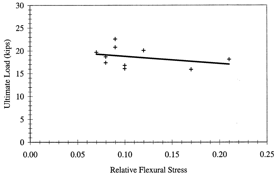
Figure 3.53 M1, Bond Test Relative Induced Flexural Stress
