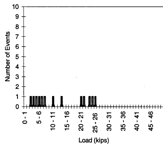
Figure F.69 2M2-6-2-15.0-3
