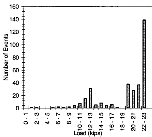
Figure F.27 1M1-5-2-15.0-3
