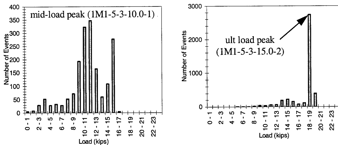
Figure 3.35 M1, C3 (concrete sensors) AE Peaks
