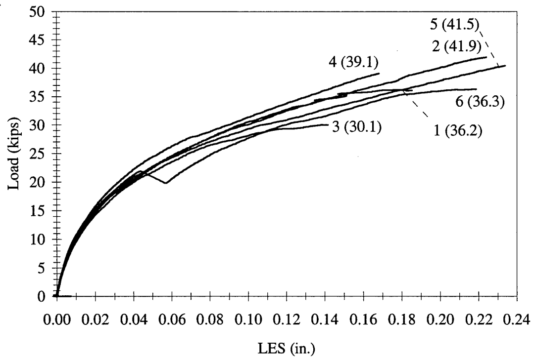
Figure 3.20 LES vs. Load, M2-6-2-25.0
