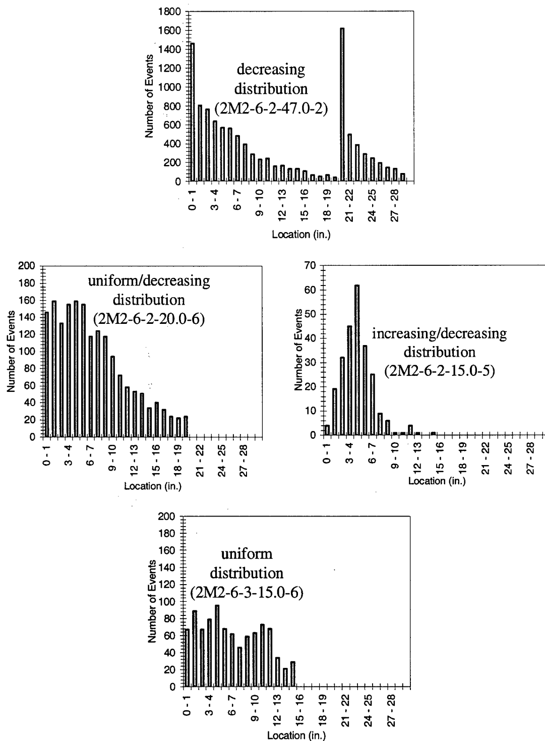
Figure 3.32 M2, C2 (concrete sensors) Distribution Patterns
