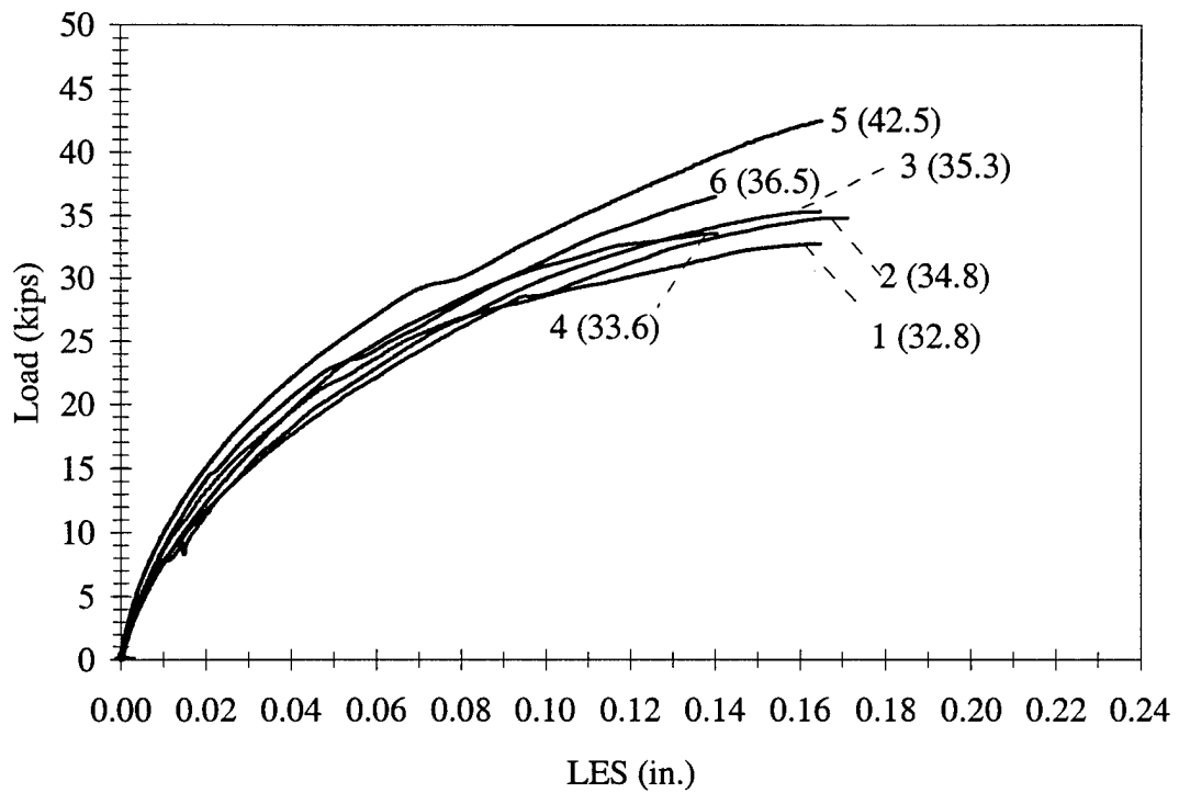
Figure 3.14 LES vs. Load, M2-6-3-20.0
