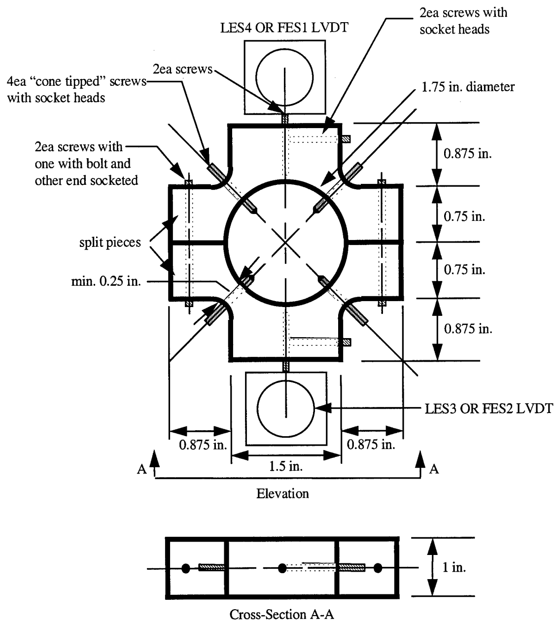
Figure 2.18 LVDT Bracket
