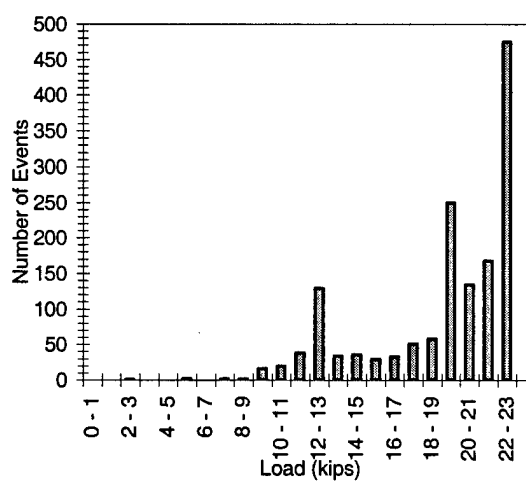
Figure F.27 1M1-5-2-15.0-3
