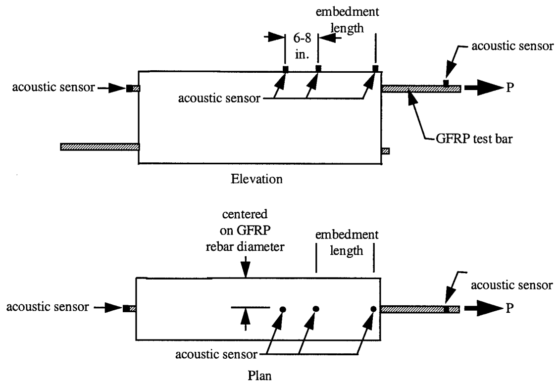
Figure 2.21 Acoustic Sensor Layout
