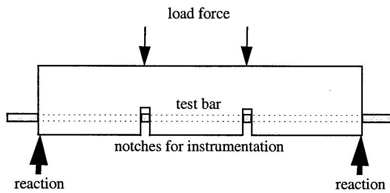
Figure 1.4 Notch Beam Bond Test
