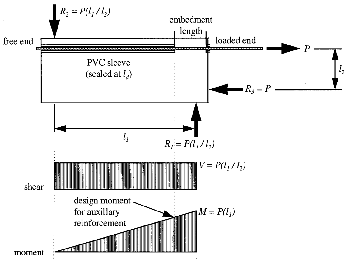
Figure 2.4 Shear and Moment Diagrams
