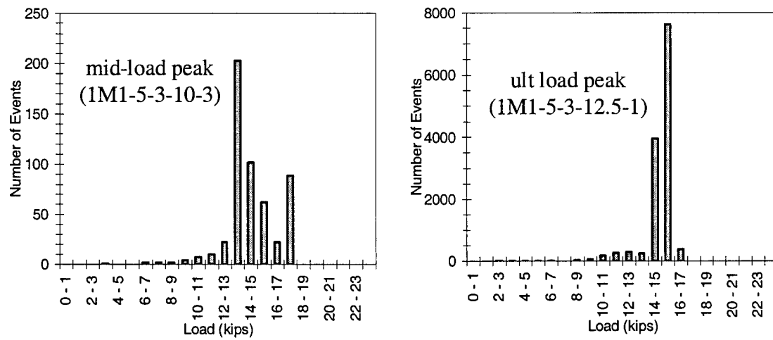
Figure 3.37 M1, B3 (bar sensors) AE Peaks
