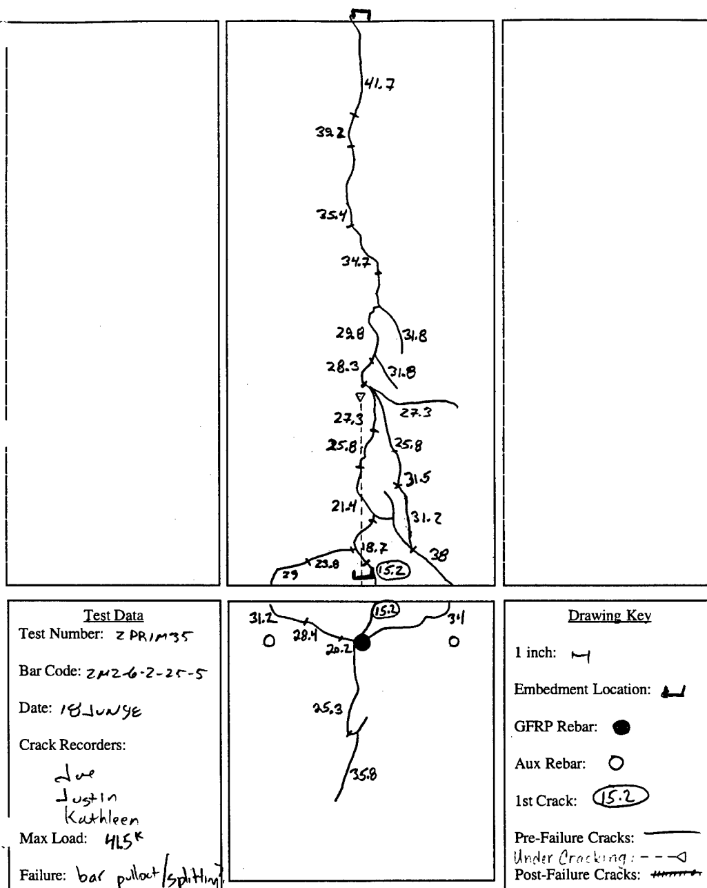
Figure E.59 2M2-6-2-25.0-5
