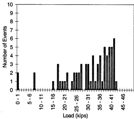
Figure F.56 2M2-6-2-25.0-2
