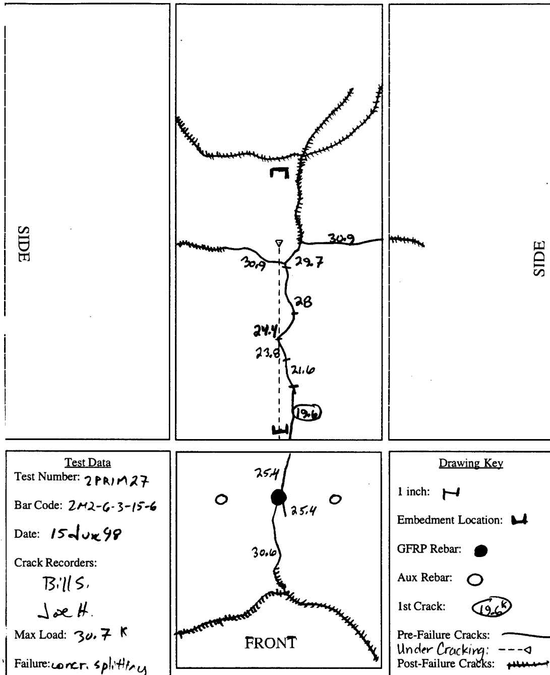
Figure 3.40 M2, Sample Crack Pattern
