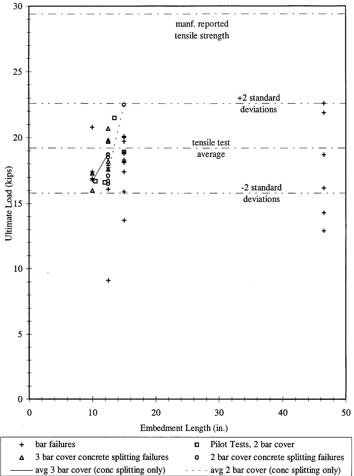
Figure 3.52 M1, Embedment Length versus Ultimate Load
