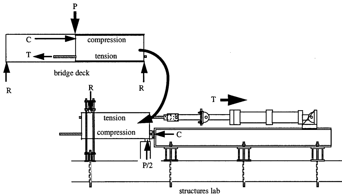
Figure 1.7 Inverted Half-Beam Bond Test
