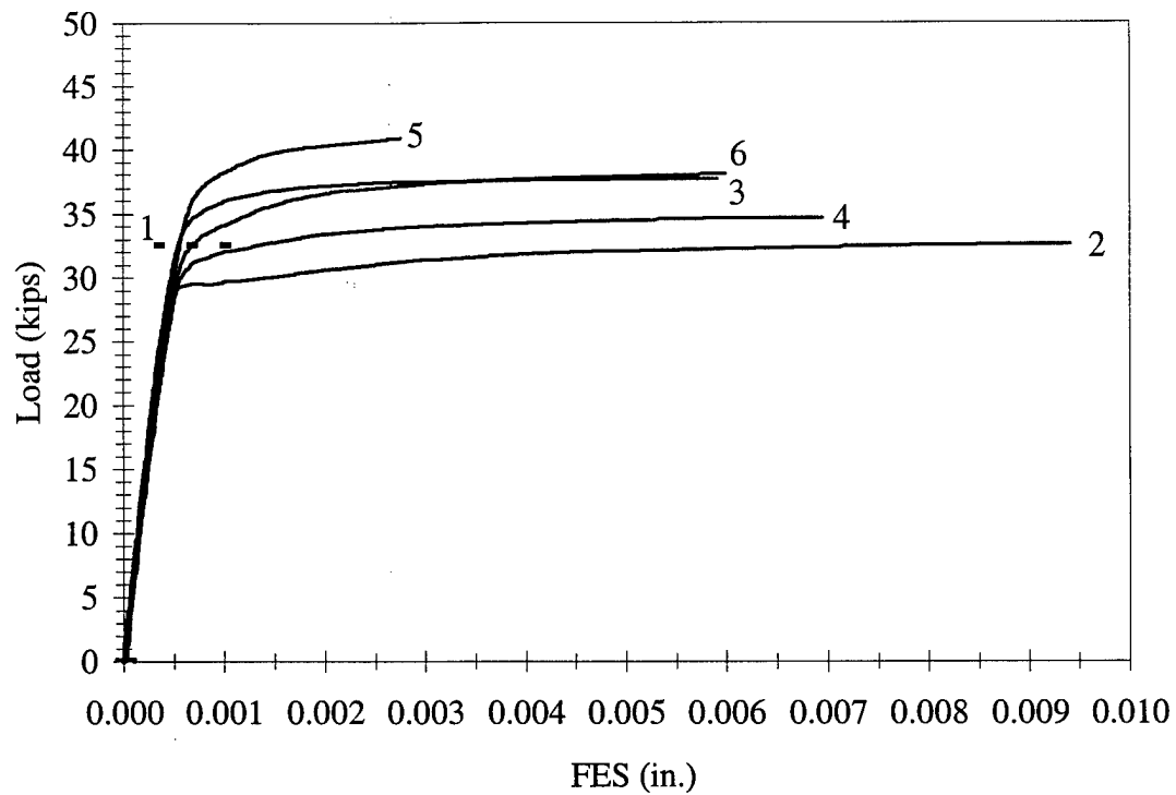
Figure 3.21 FES vs. Load, M2-6-2-20.0
