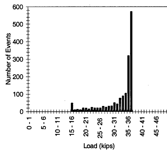
Figure F.55 2M2-6-2-25.0-1
