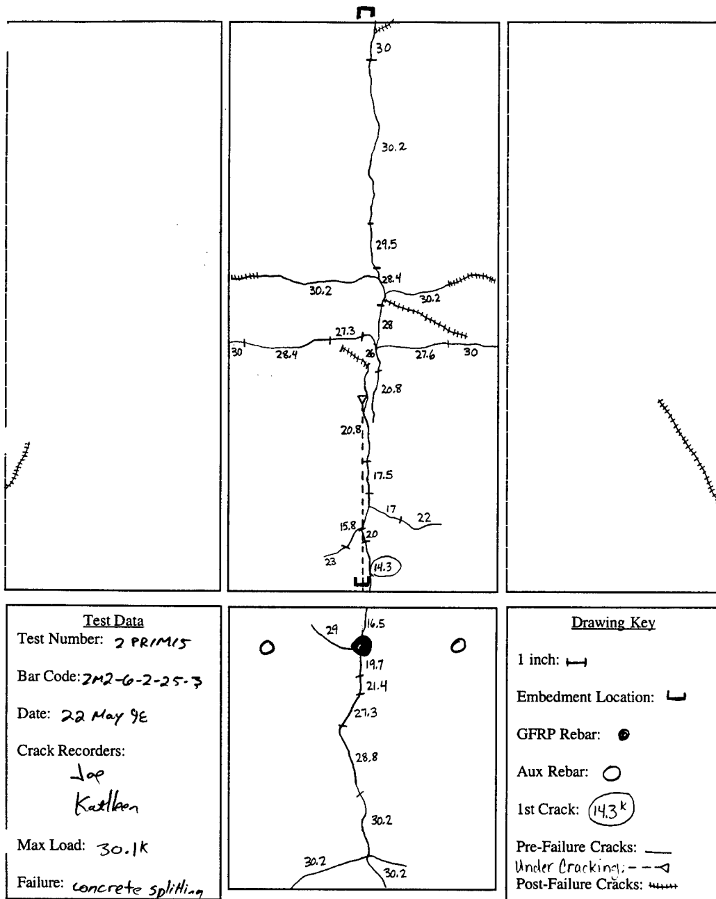
Figure E.57 2M2-6-2-25.0-3
