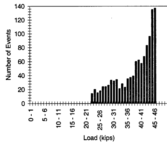
Figure F.53 2M2-6-2-47.0-2
