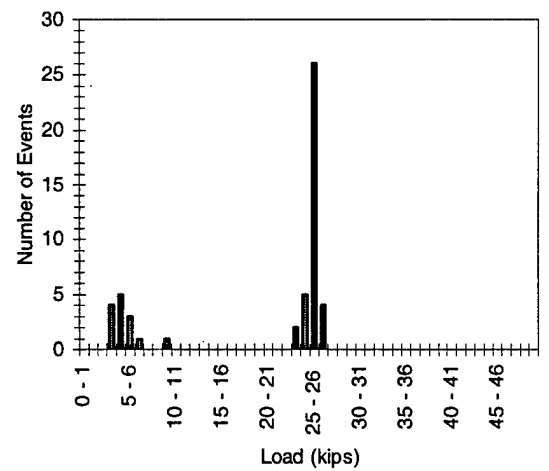
Figure F.47 2M2-6-3-15.0-2
