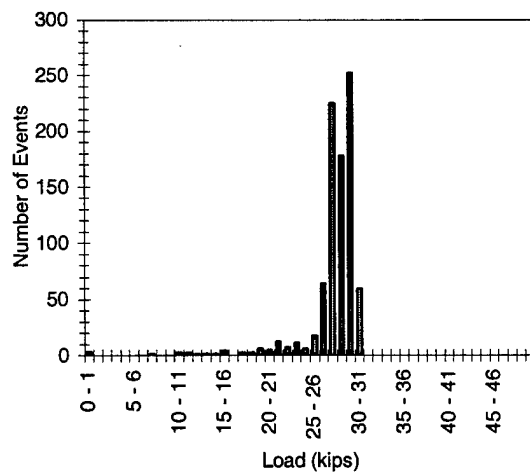
Figure F.57 2M2-6-2-25.0-3
