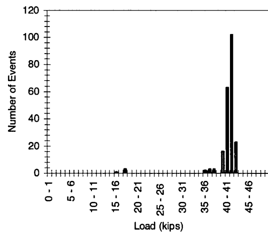
Figure F.44 2M2-6-3-20.0-5
