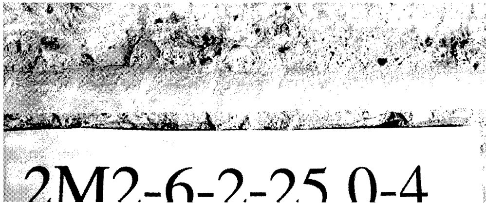
Figure 3.49 M2, Bar Impressions in Concrete
