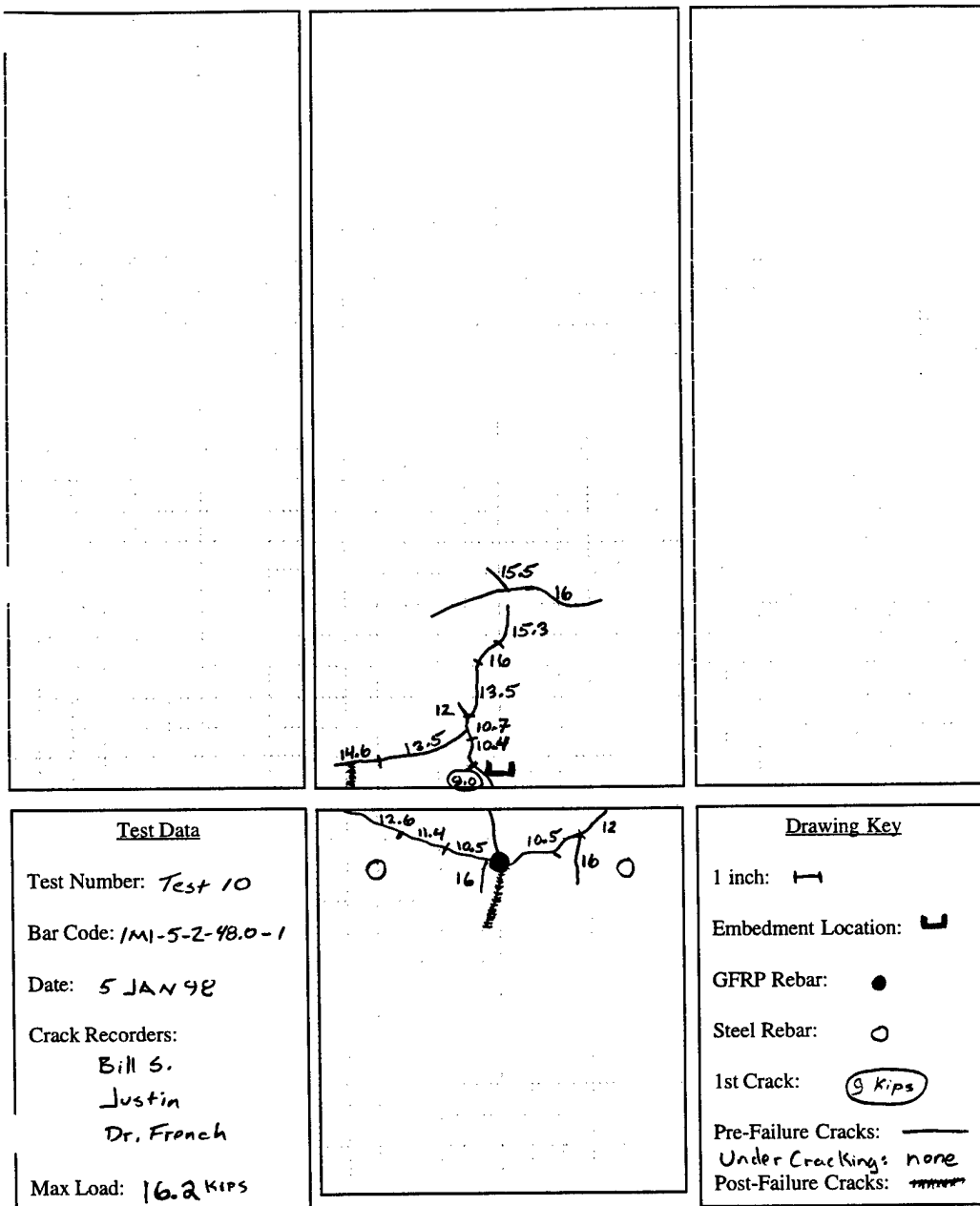
Figure E.19 1M1-5-2-47.0-1
