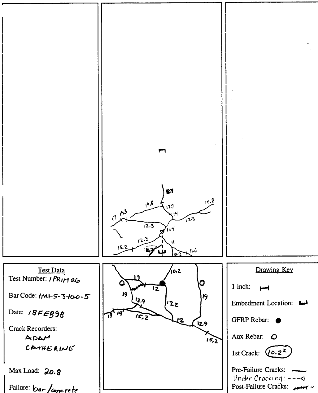
Figure E.17 1M1-5-3-10.0-5
