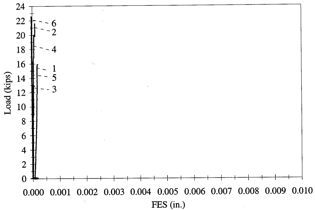
Figure 3.7 FES vs. Load, M1-5-2-47.0
