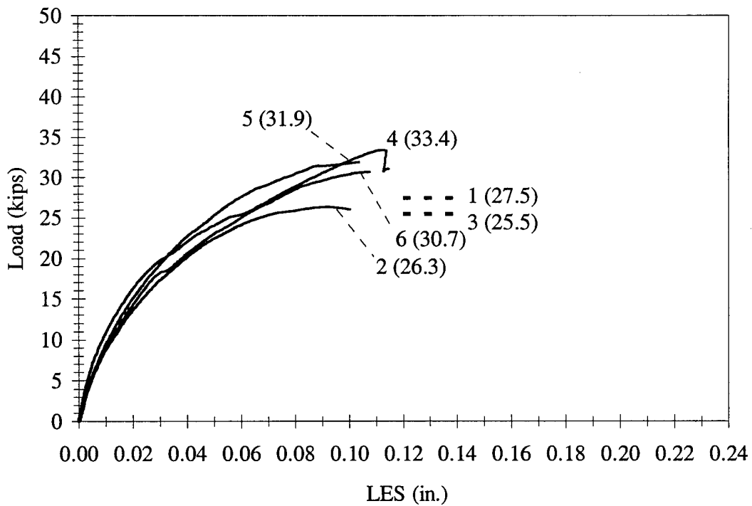
Figure 3.16 LES vs. Load, M2-6-3-15.0
