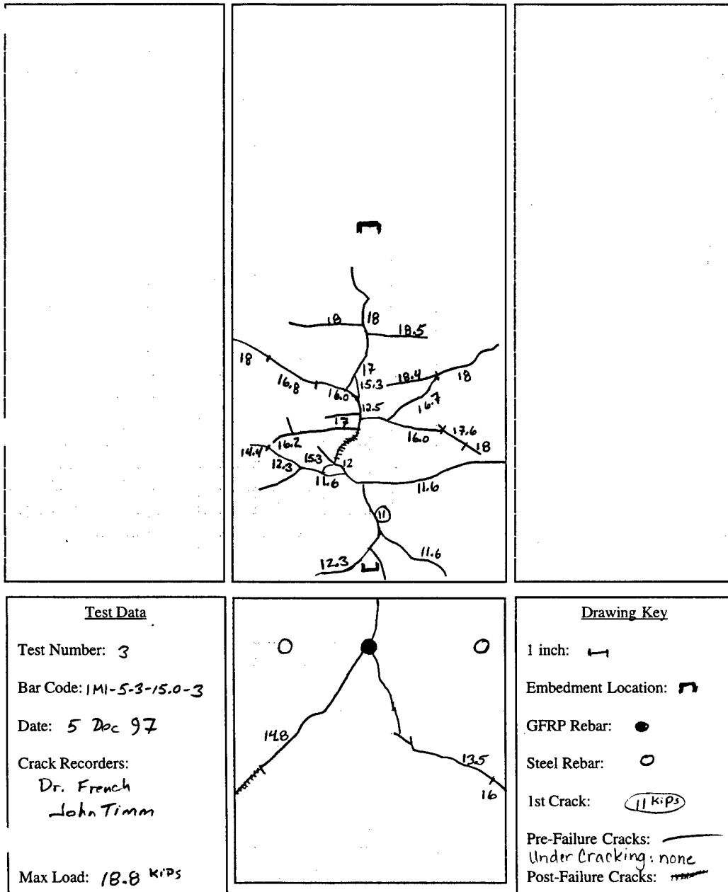
Figure E.3 1M1-5-3-15.0-3
