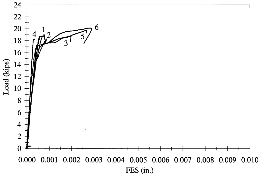
Figure 3.1 FES vs. Load, M1-5-3-15.0
