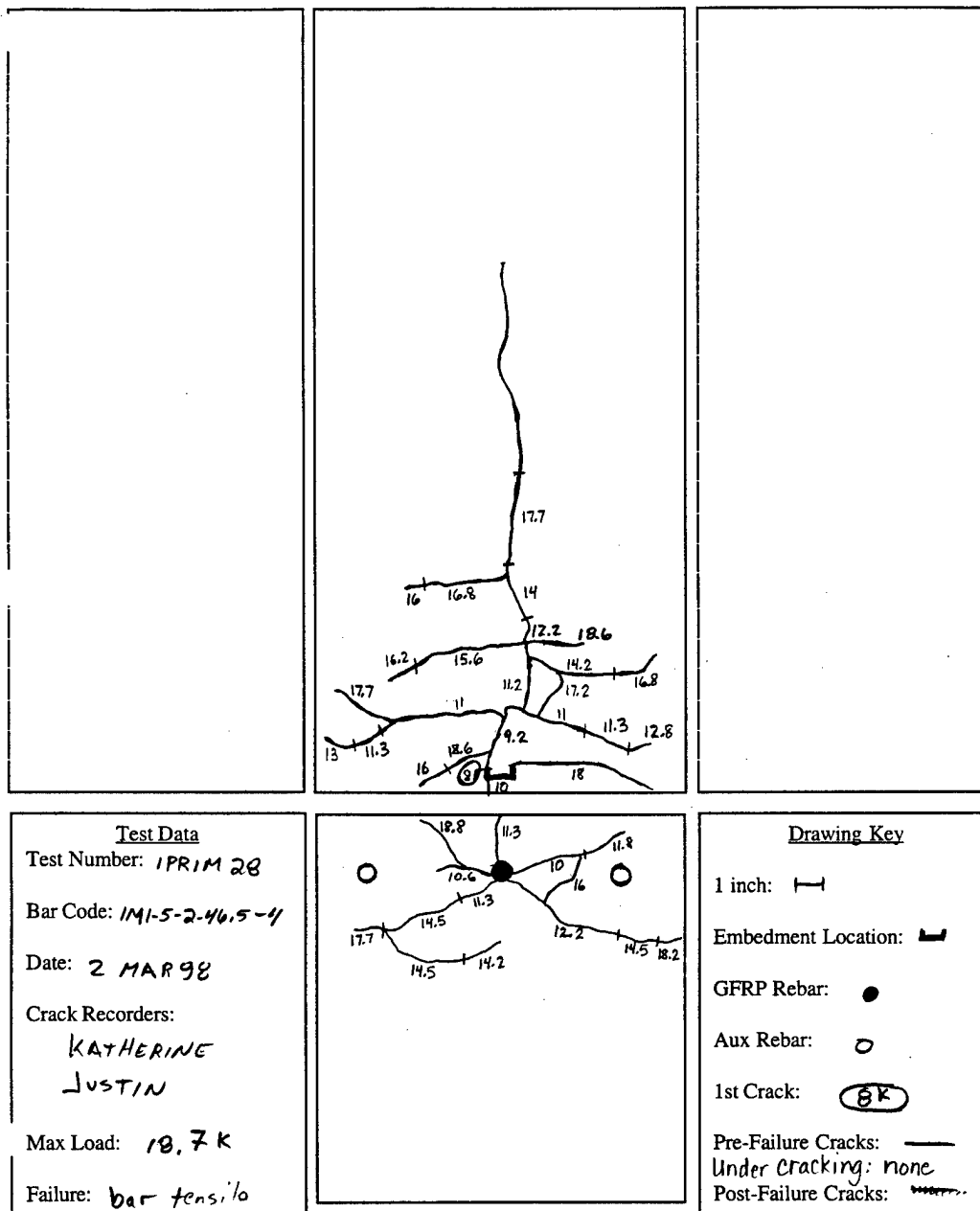
Figure E.22 1M1-5-2-47.0-4
