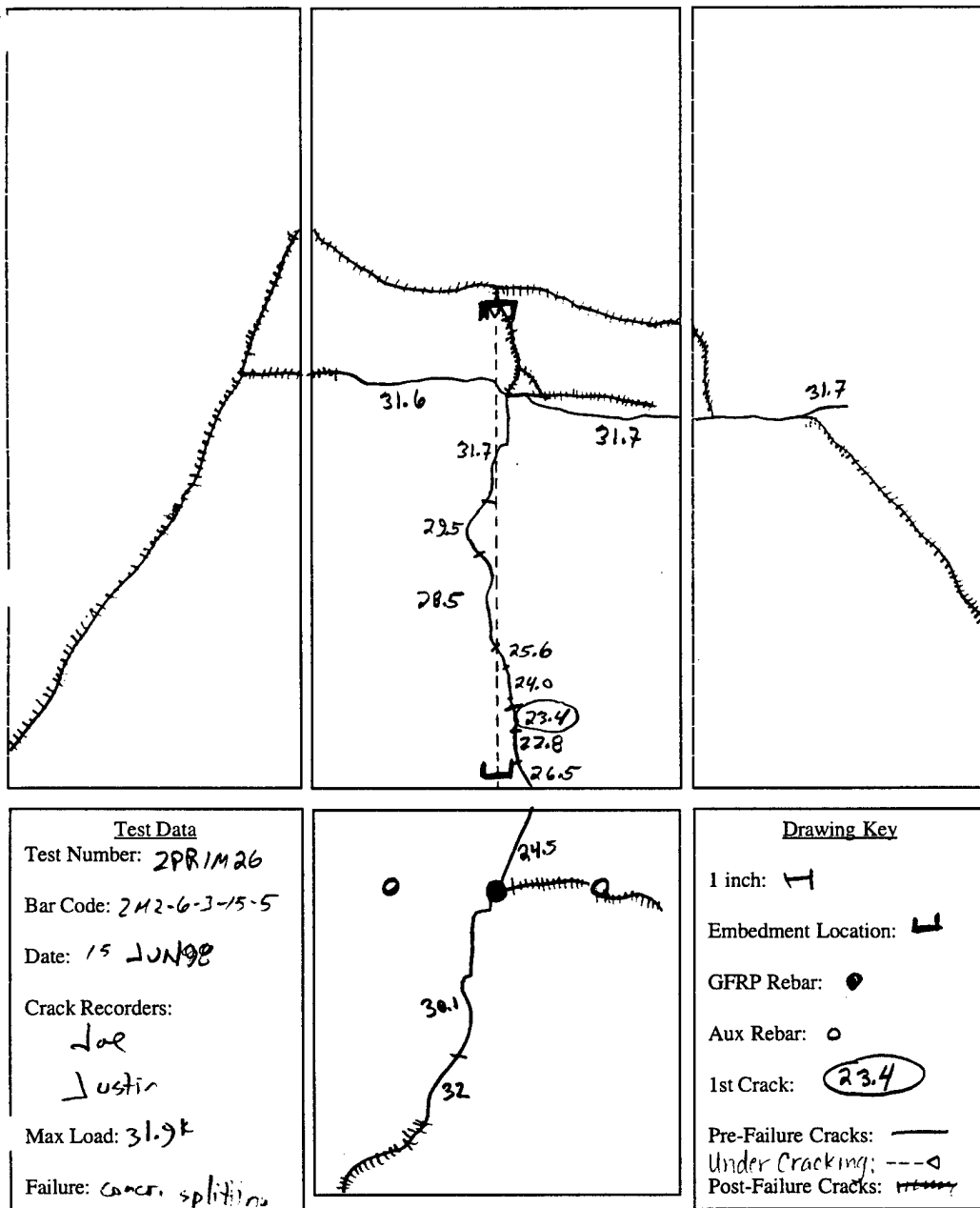
Figure E.50 2M2-6-3-15.0-5
