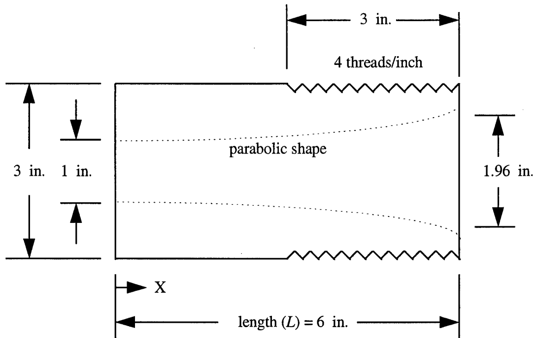
Figure 2.11 Aluminum Parabolic Grip for No.5 and No.6 GFRP Rebar
