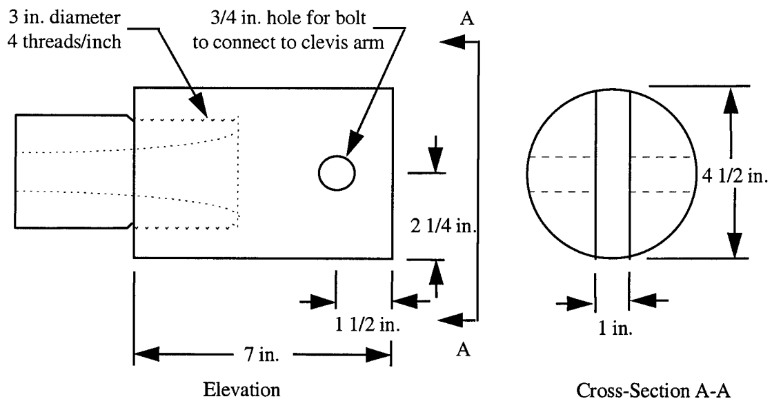
Figure 2.13 Steel Connector for No.5 and 6 GFRP Rebar Aluminum Parabolic Grip
