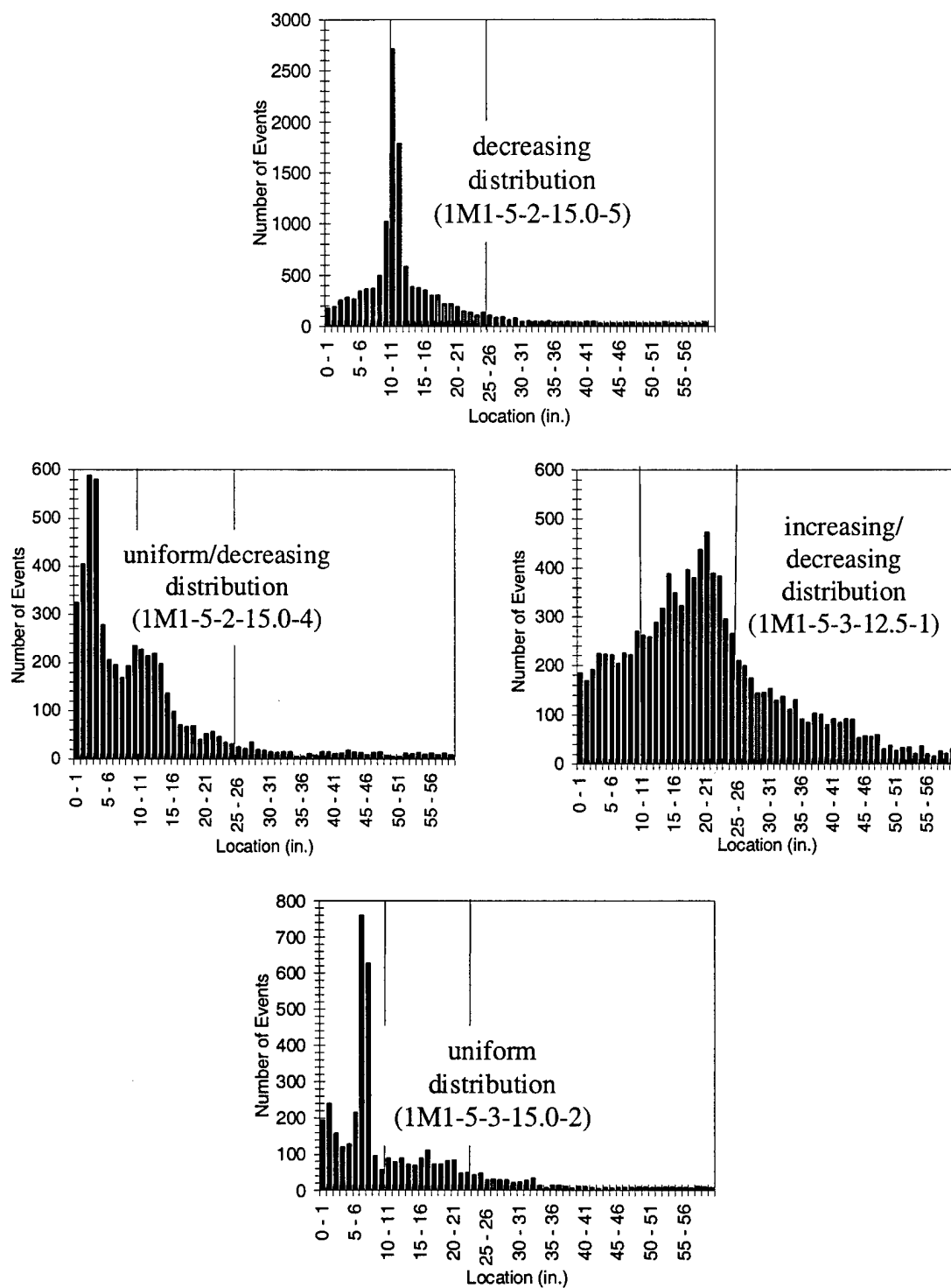
Figure 3.33 M1, B2 (bar sensors) Distribution Patterns
