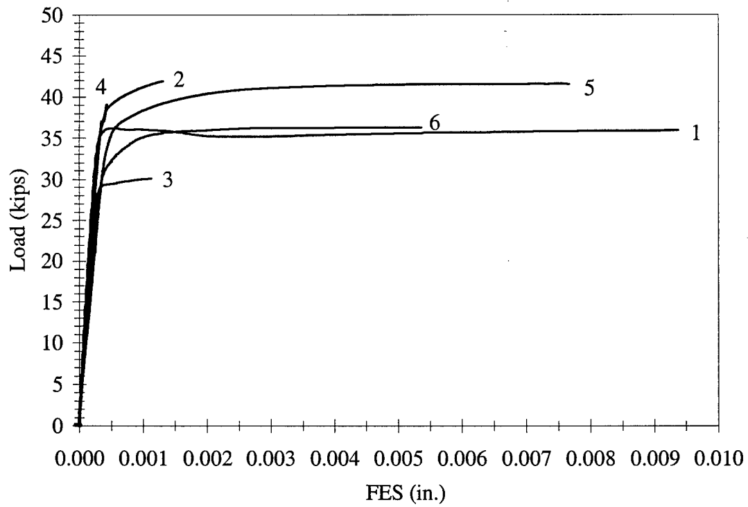
Figure 3.19 FES vs. Load, M2-6-2-25.0
