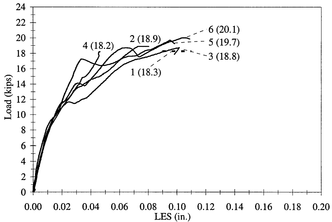
Figure 3.2 LES vs. Load, M1-5-3-15.0
