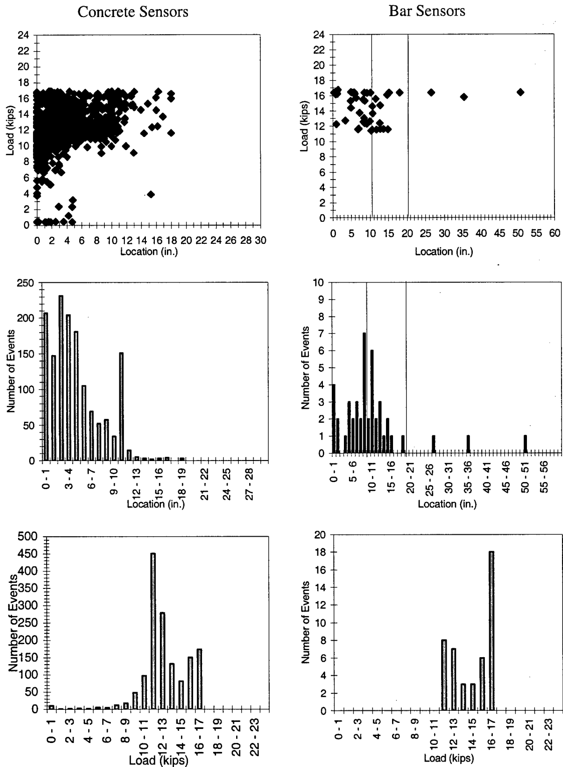
Figure F.16 1M1-5-3-10.0-4
