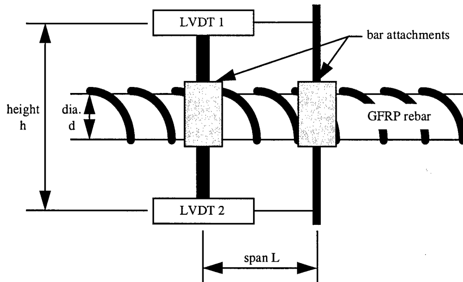
Figure D.1 LVDT Setup
