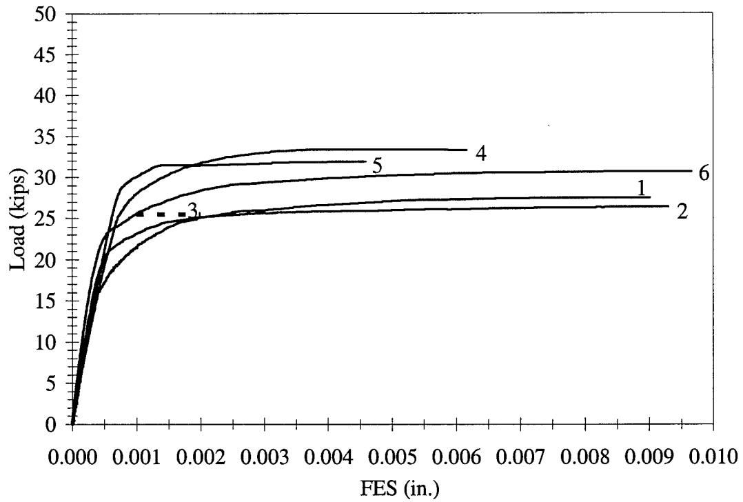
Figure 3.15 FES vs. Load, M2-6-3-15.0
