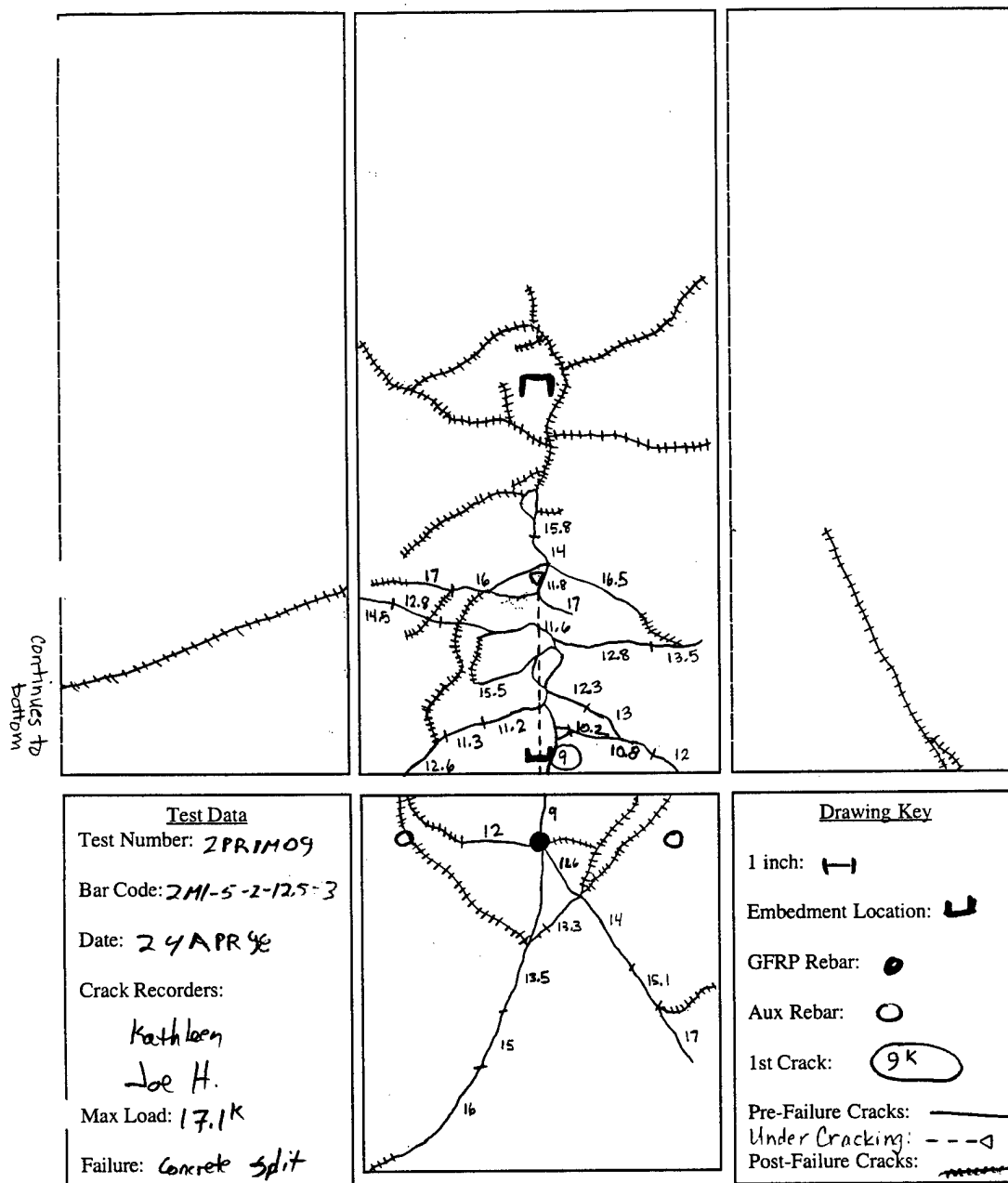
Figure E.39 2M1-5-2-12.5-3
