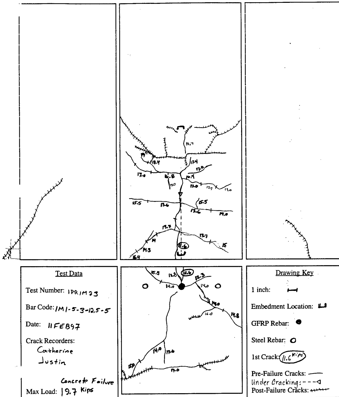
Figure E.11 1M1-5-3-12.5-5
