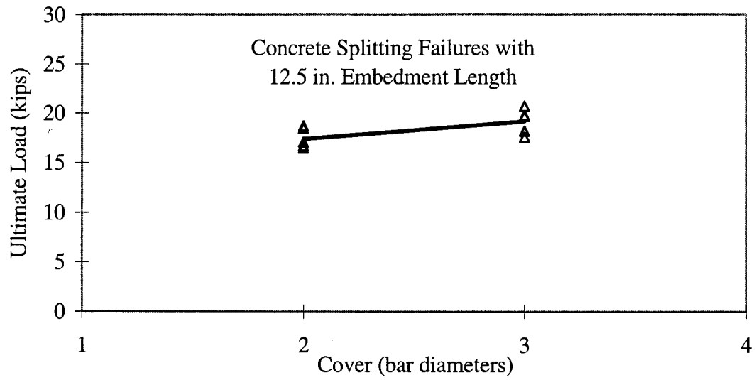
Figure 3.55 M1, Cover versus Ultimate Load
