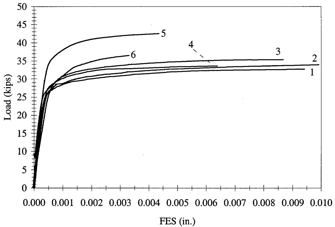
Figure 3.13 FES vs. Load, M2-6-3-20.0
