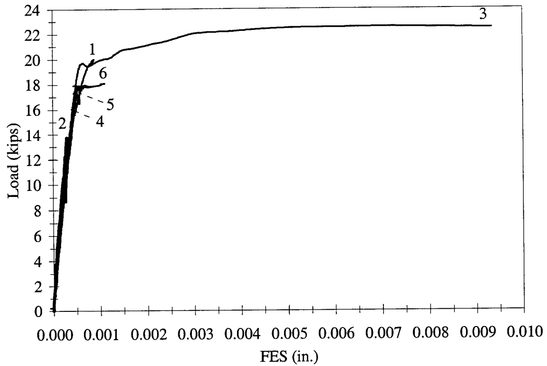
Figure 3.9 FES vs. Load, M1-5-2-15.0
