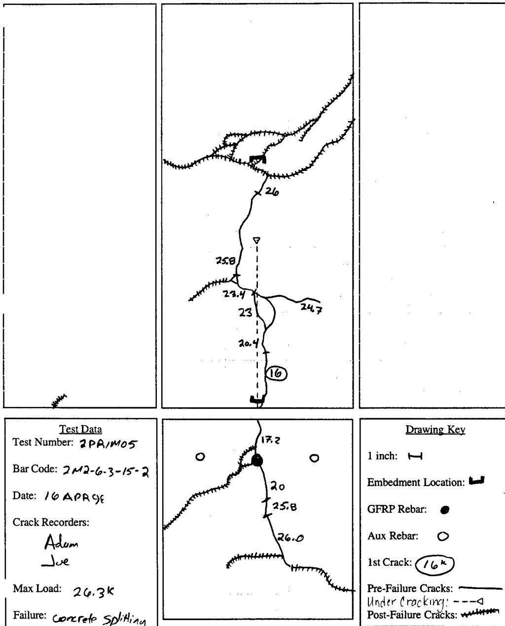
Figure E.47 2M2-6-3-15.0-2
