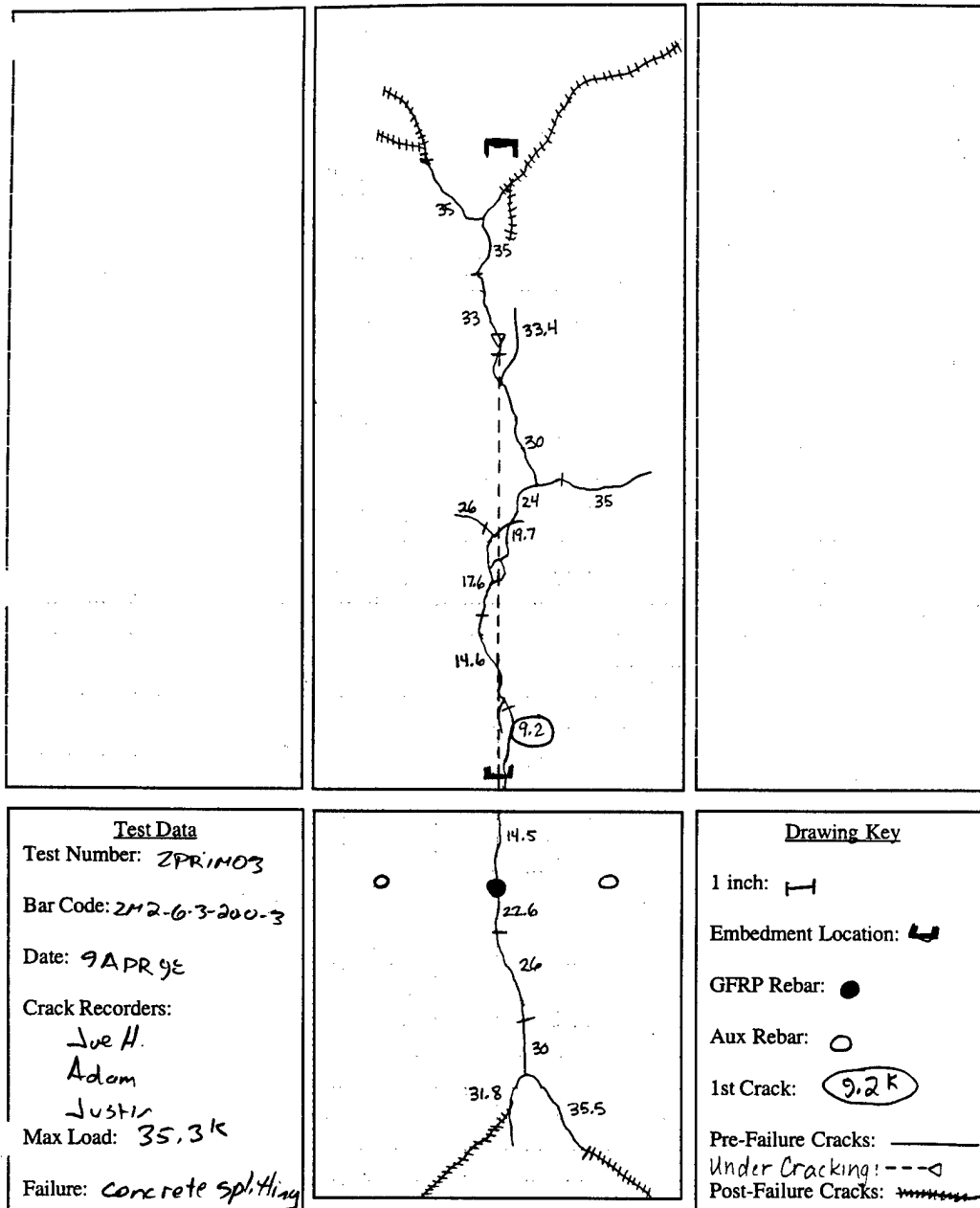
Figure E.42 2M2-6-3-20.0-3
