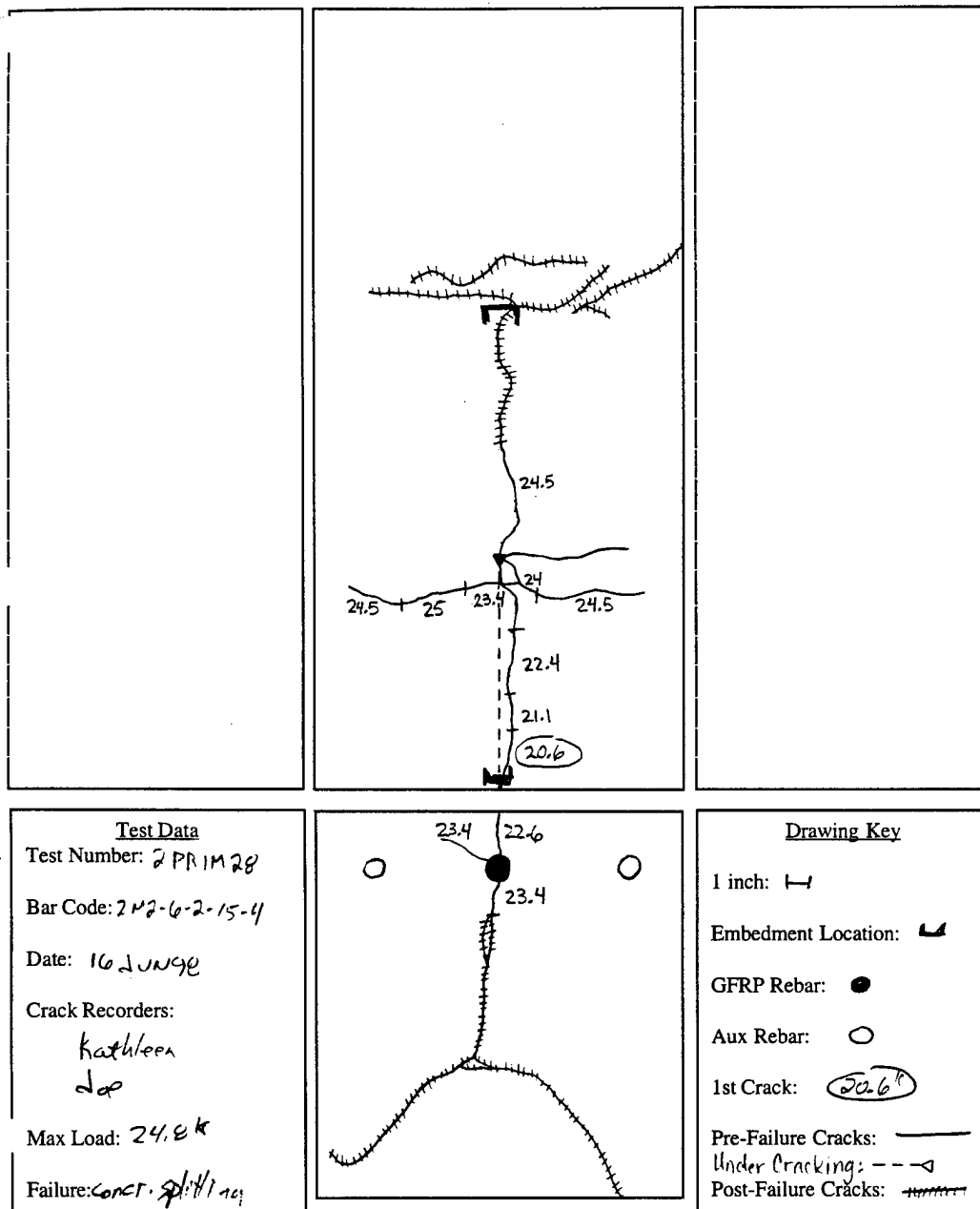
Figure E.70 2M2-6-2-15.0-4
