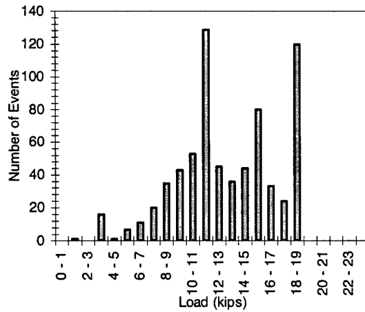
Figure F.1 1M1-5-3-15.0-1
