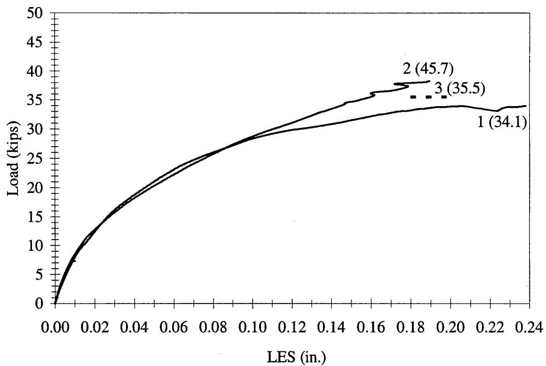
Figure 3.18 LES vs. Load, M2-6-2-47.0
