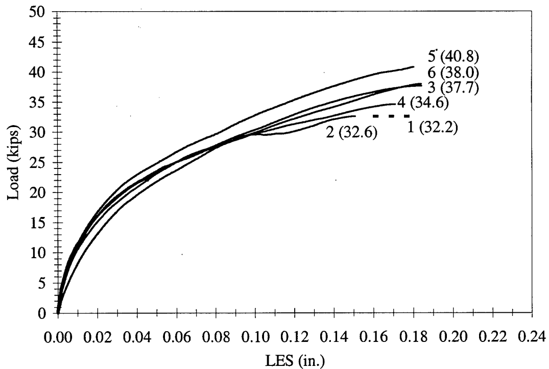
Figure 3.22 LES vs. Load, M2-6-2-20.0
