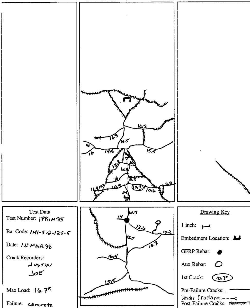
Figure E.35 1M1-5-2-12.5-5
