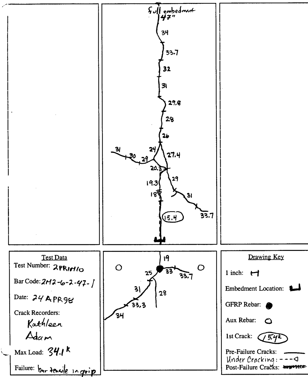
Figure E.52 2M2-6-2-47.0-1
