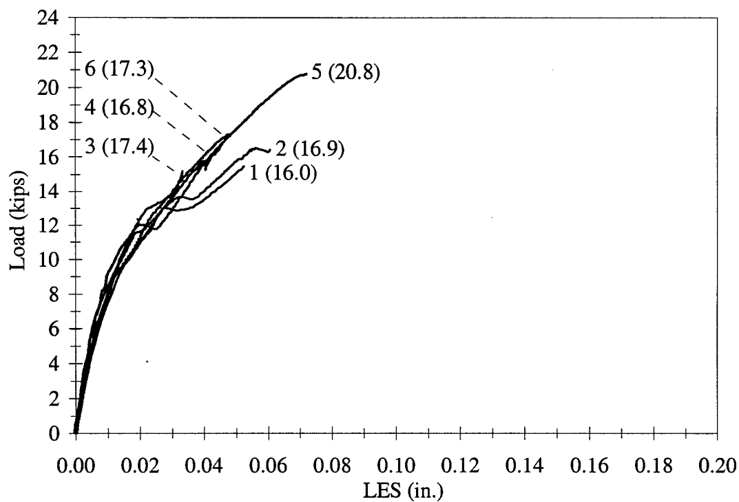
Figure 3.6 LES vs. Load, M1-5-3-10.0
