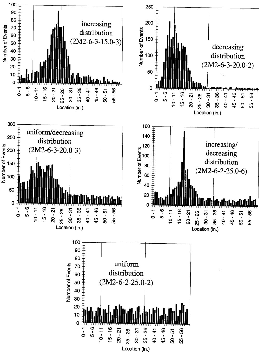
Figure 3.34 M2, B2 (bar sensors) Distribution Patterns
