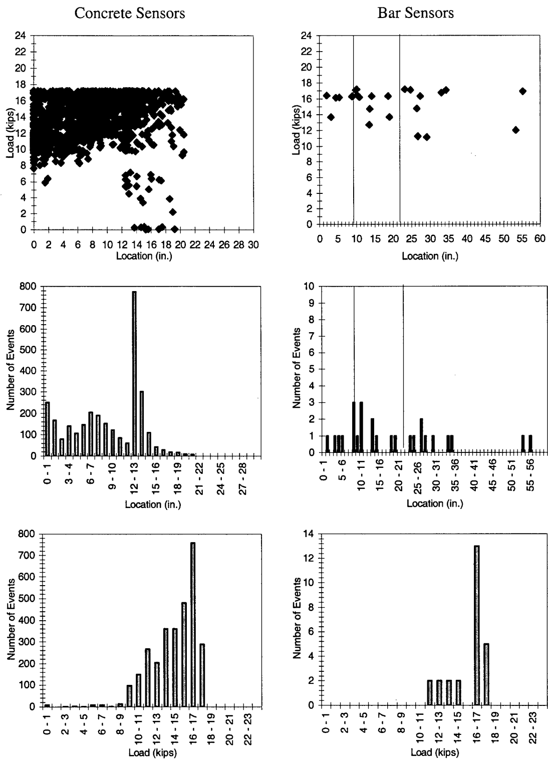
Figure F.39 2M1-5-2-12.5-3
