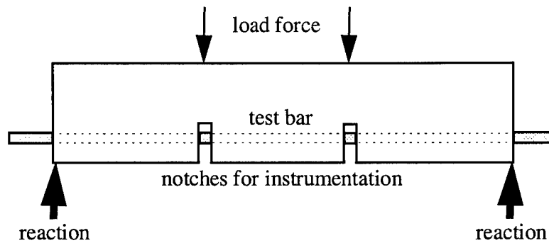
Figure 1.6 Hinge Beam Bond Test
