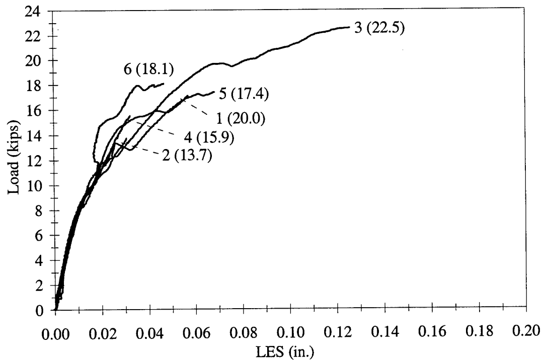
Figure 3.10 LES vs. Load, M1-5-2-15.0
