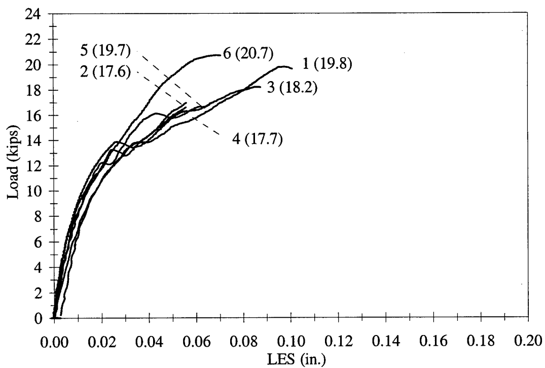
Figure 3.4 LES vs. Load, M1-5-3-12.5
