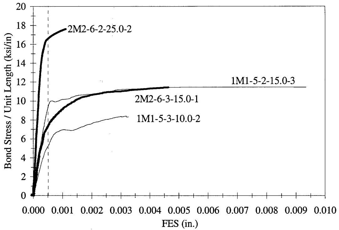
Figure 3.62 FES Comparison
