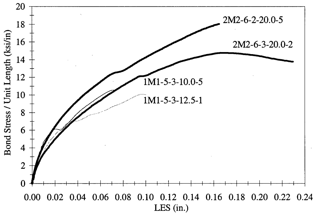
Figure 3.63 LES Comparison
