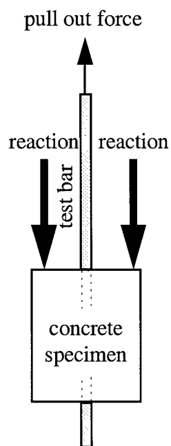
Figure 1.2 Pullout Bond Test
