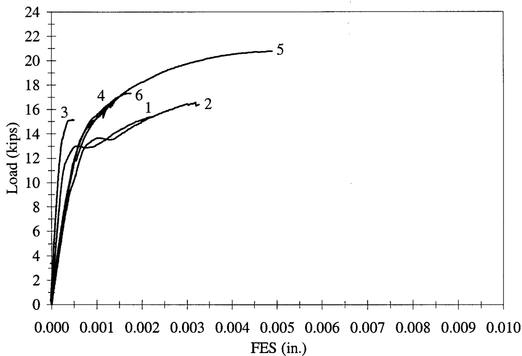
Figure 3.5 FES vs. Load, M1-5-3-10.0
