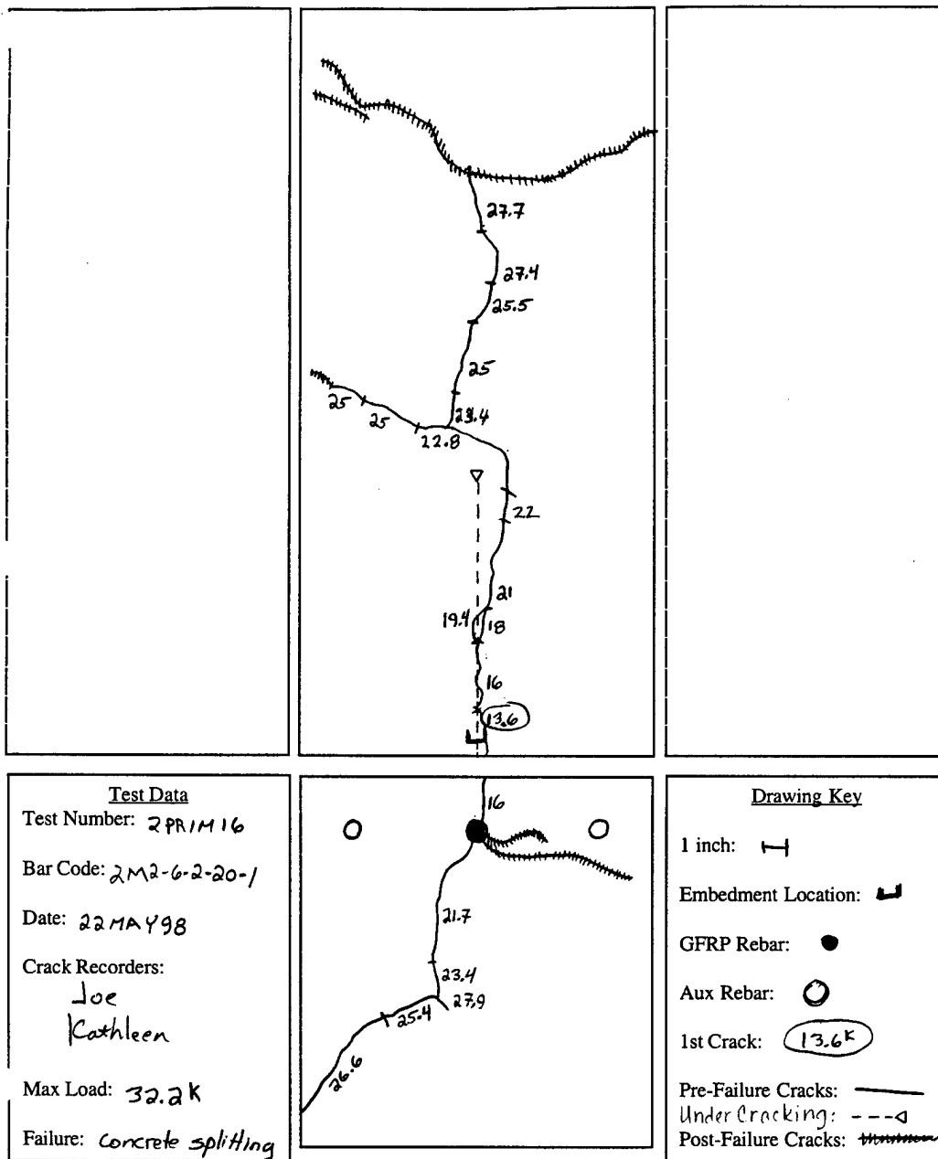
Figure E.61 2M2-6-2-20.0-1
