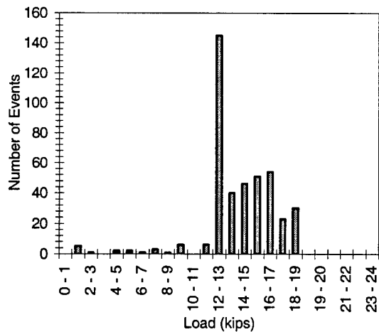
Figure F.9 1M1-5-3-12.5-3
