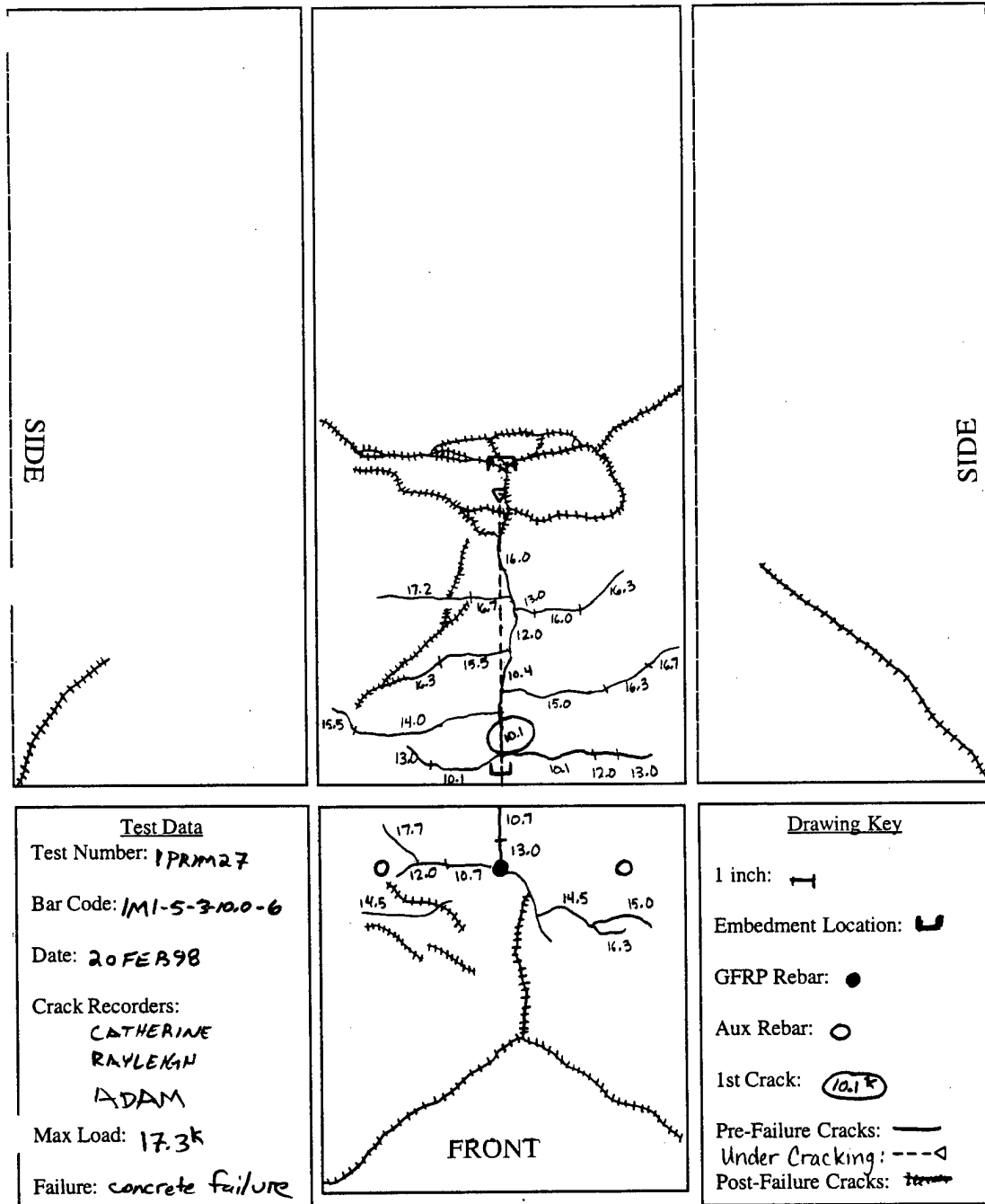
Figure 3.39 M1, Sample Crack Pattern
