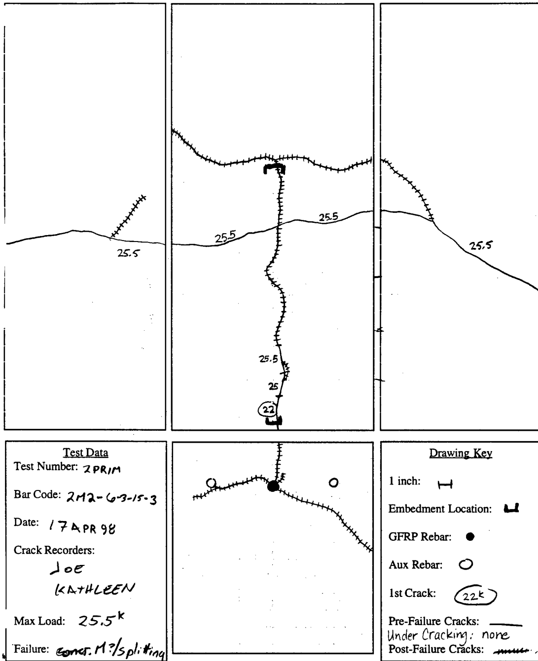
Figure 3.51 2M2-6-3-15.0-3 Crack Pattern
