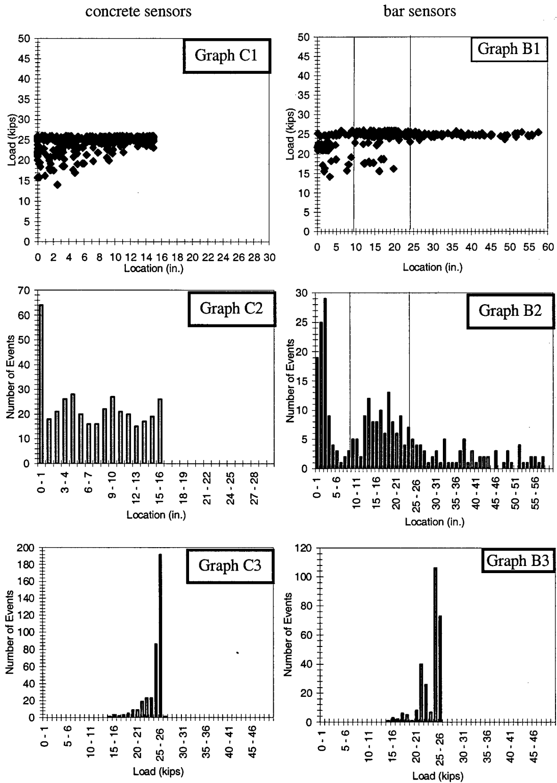
Figure 3.30 M2, Sample AE Graphs
