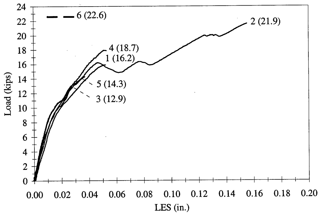
Figure 3.8 LES vs. Load, M1-5-2-47.0
