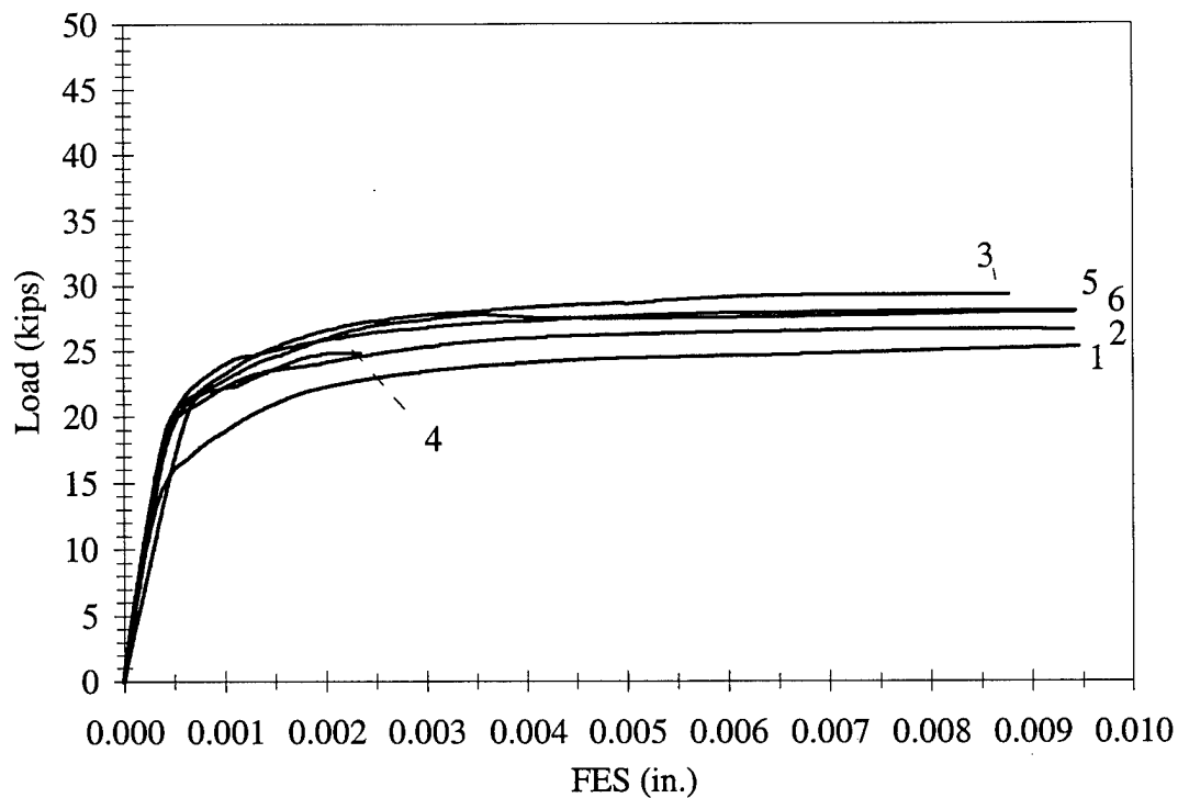
Figure 3.23 FES vs. Load, M2-6-2-15.0
