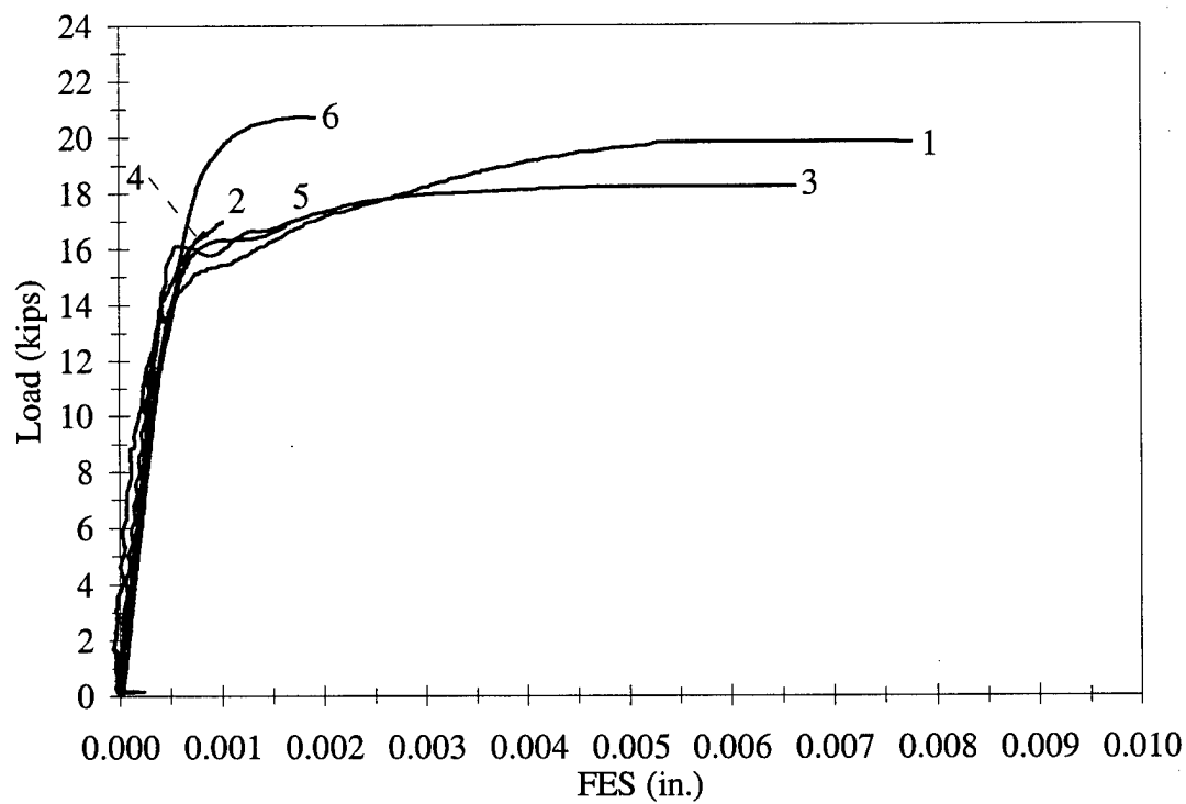
Figure 3.3 FES vs. Load, M1-5-3-12.5
