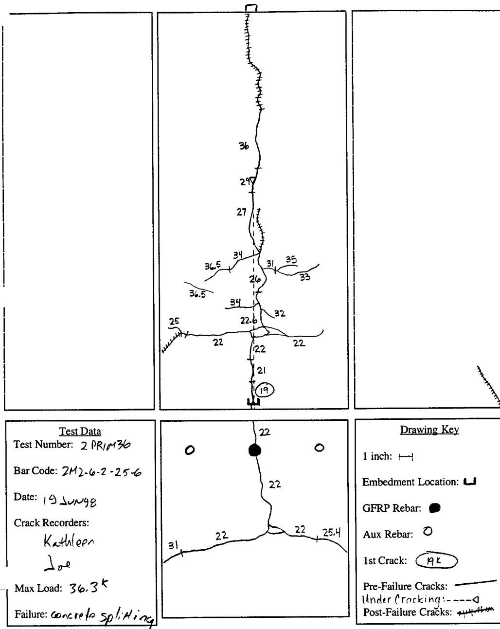
Figure E.60 2M2-6-2-25.0-6
