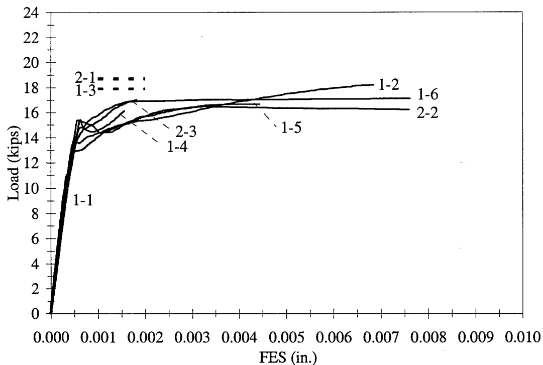
Figure 3.11 FES vs. Load, M1-5-2-12.5
