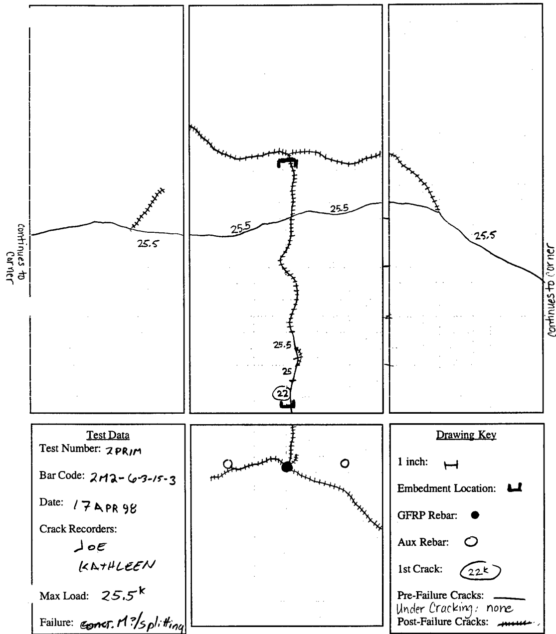
Figure E.48 2M2-6-3-15.0-3
