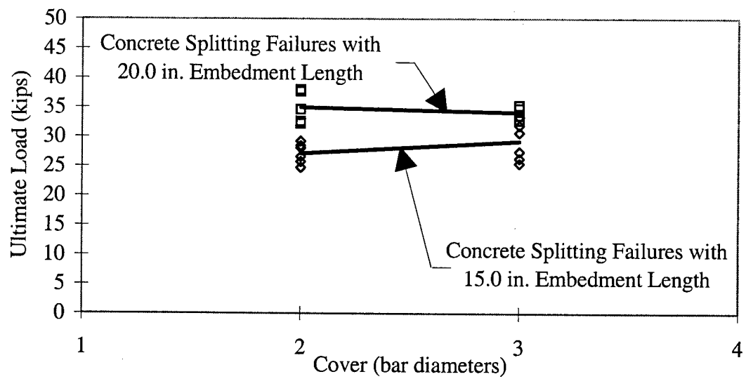
Figure 3.60 M2, Cover versus Ultimate Load
