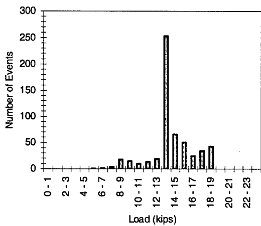
Figure F.32 1M1-5-2-12.5-2
