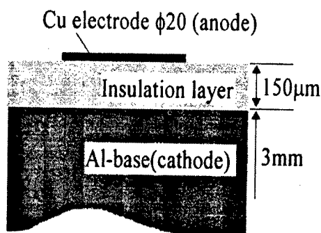
Fig. 1 Test specimen
