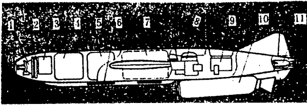
figure 2. Layout of Missile Components
