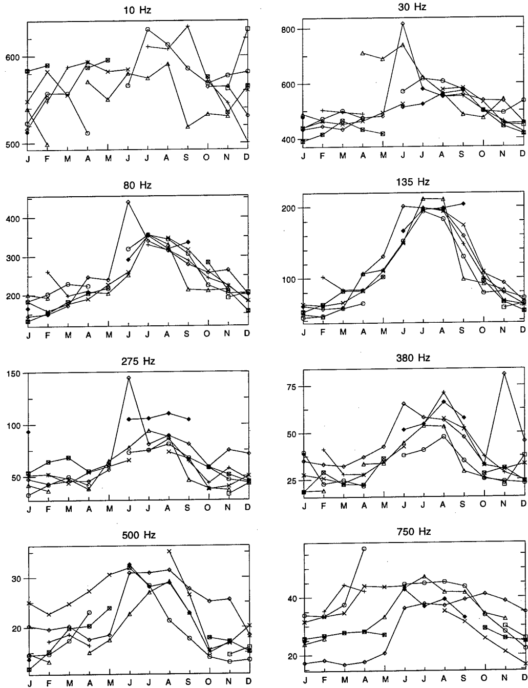
Figure 110: Monthly variation of ELF/VLF radio noise at Stanford, California, for the eight lowest-frequency channels and the 16-20 UT time block, each year shown individually. The years 1986 to 1993 are included.
