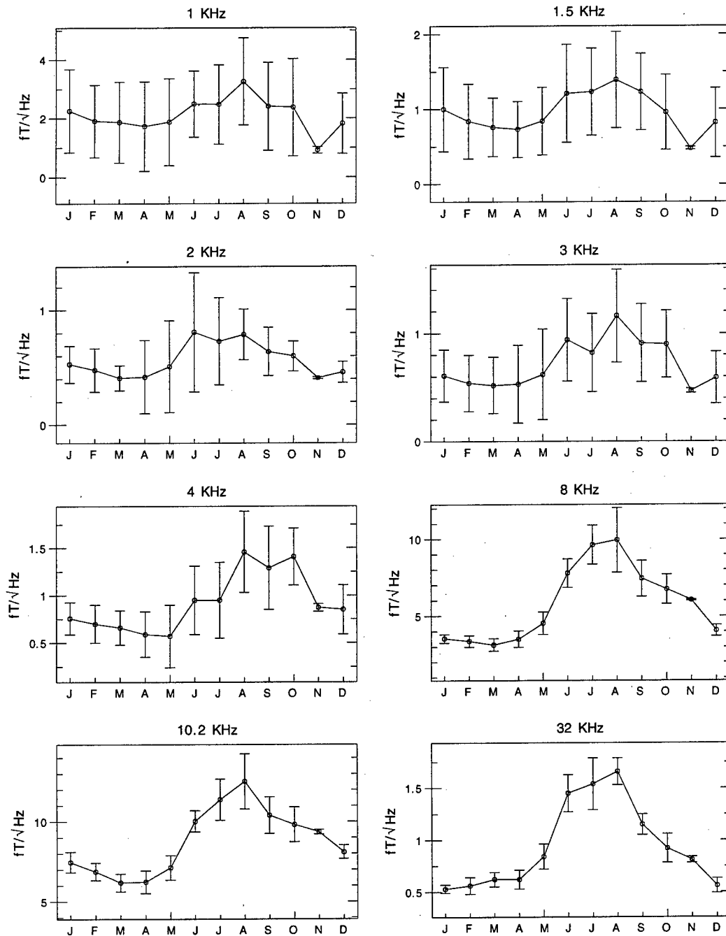
Figure 45: Monthly variation of ELF/VLF radio noise at Søndrestrom, Greenland, for the eight highest-frequency channels and the 20-24 UT time block. The years 1986 to 1991 and the year 1993 are included.
