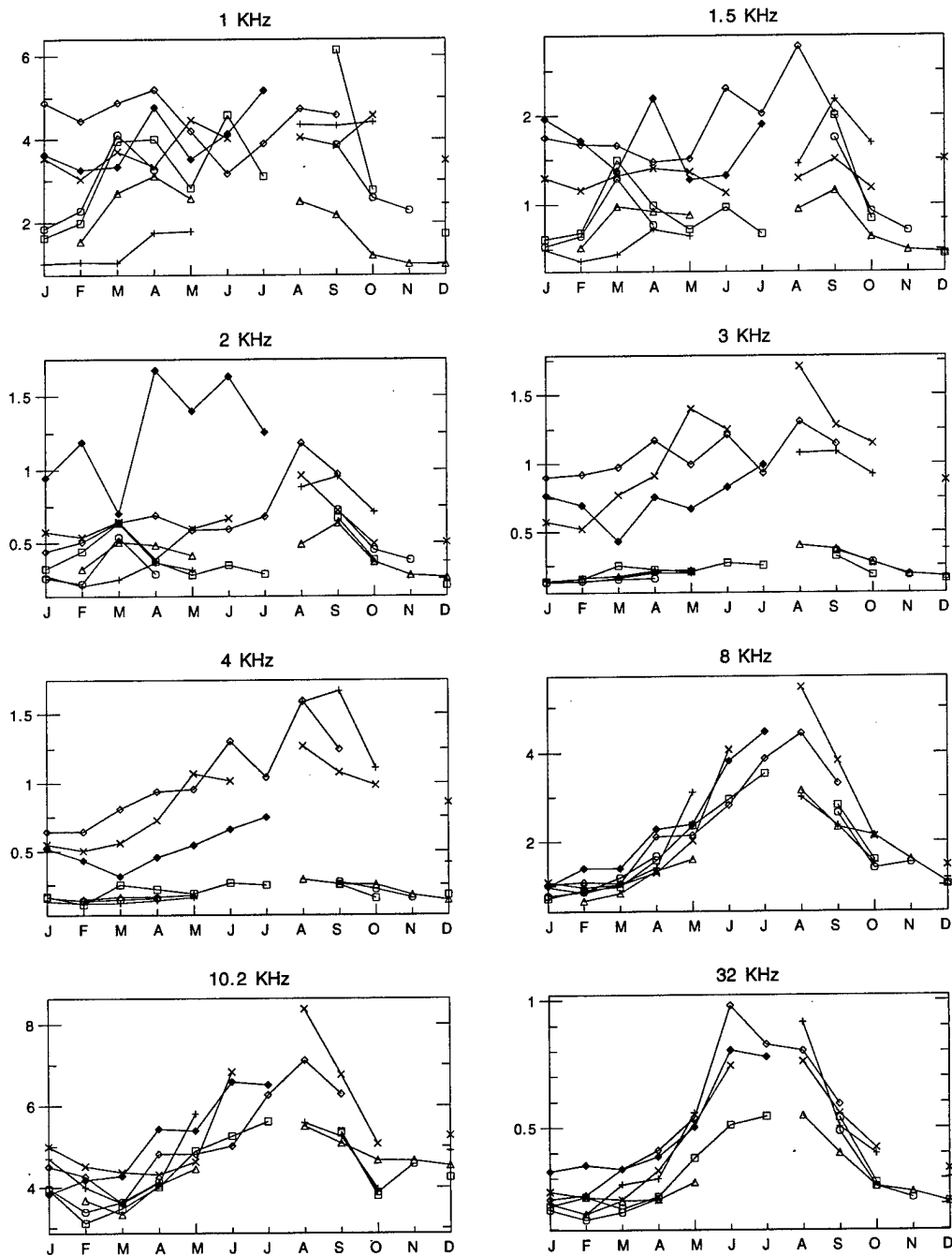
Figure 97: Monthly variation of ELF/VLF radio noise at Søndrestrøm, Greenland, for the eight highest-frequency channels and the 12-16 UT time block, each year shown individually. The years 1986 to 1991 and the year 1993 are included.
