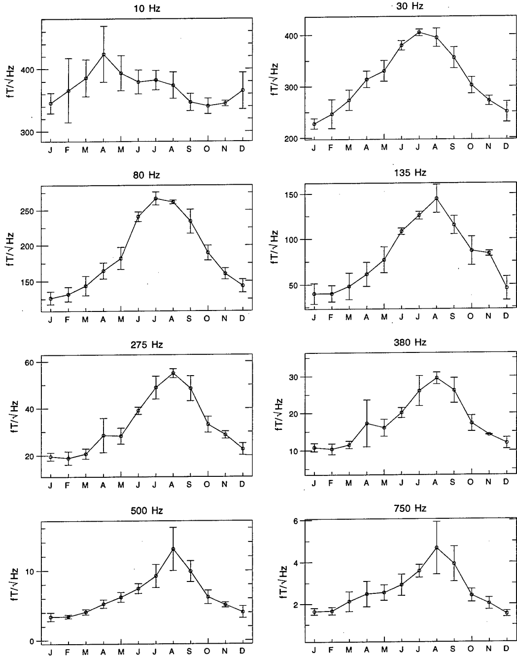
Figure 6: Monthly variation of ELF/VLF radio noise at Søndre Strømfjord, Greenland, for the eight lowest-frequency channels. The years 1986 to 1991 and 1993 are included.
