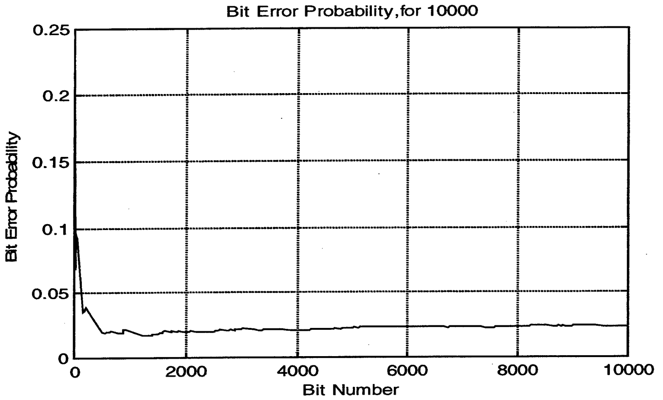
Figure 5. BER Convergence for 10^4 symbols
