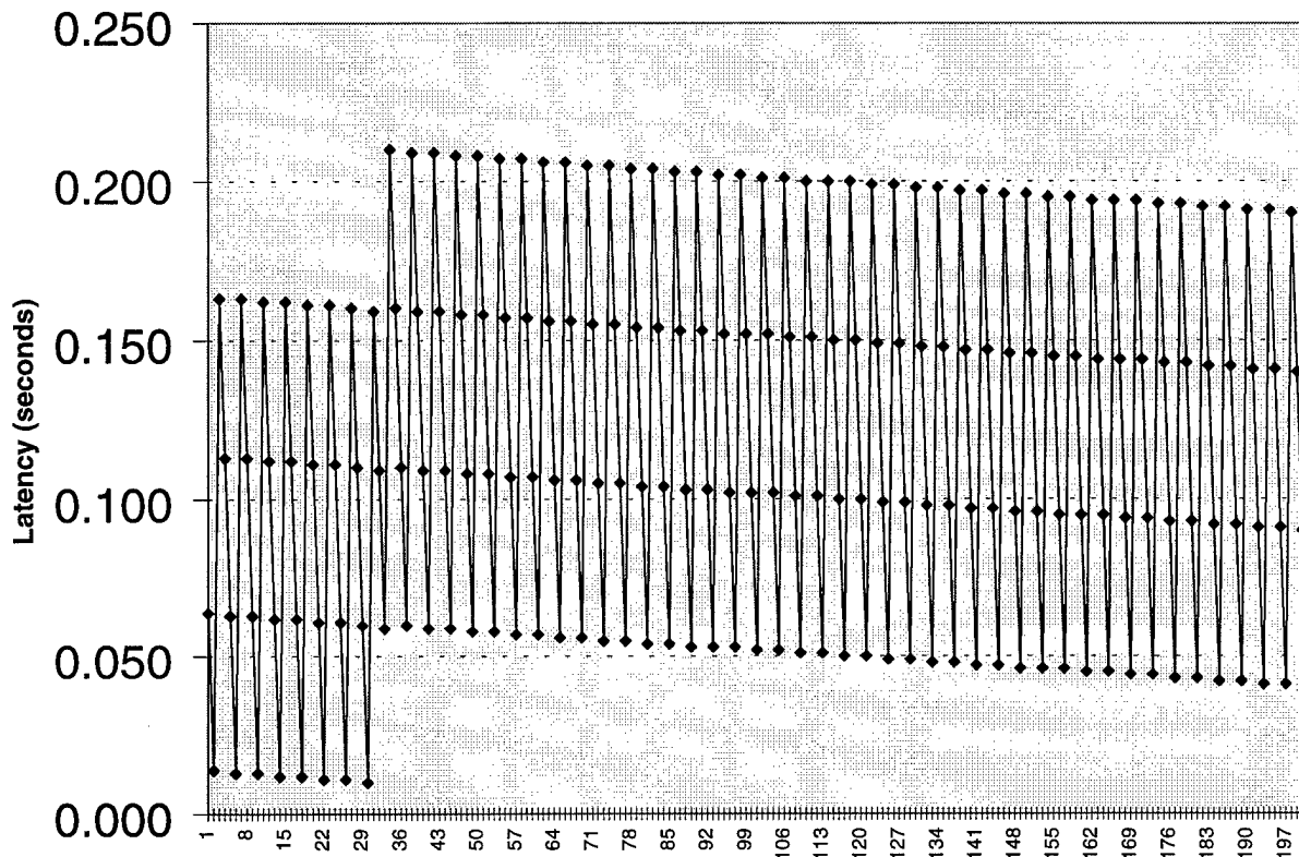
Figure 7. TCP Latency for 101 Bytes at 20 Hz
