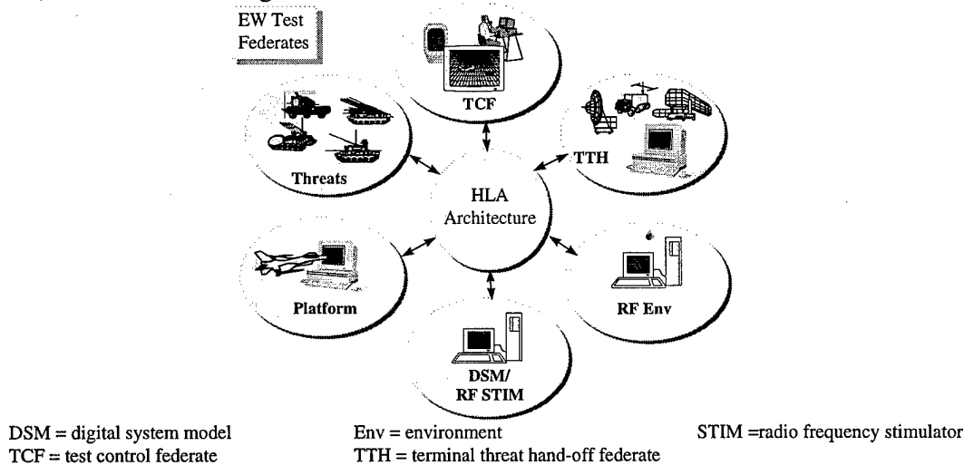
Figure 1. JADS EW Test Federate
