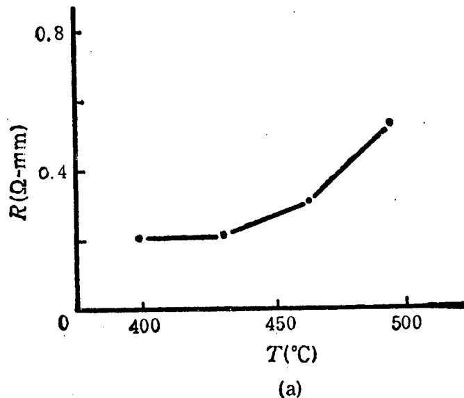
Figure 2(a). Ohmic contact resistance versus alloying temperature
