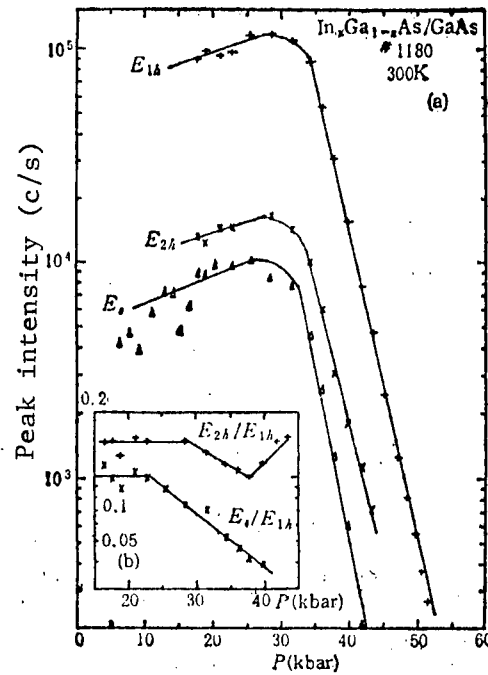
Figure 4. (a) peak intensity vs. pressure at room temperature (b) relative intensity E_s/E_{1h} and E_{2h}/E_{1h} vs. pressure at room temperature
