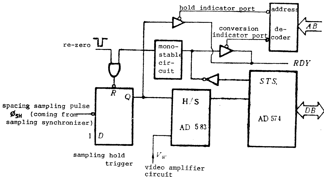
Figure 2. Data-Acquisition Interface
