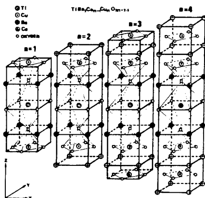
Fig.1 The crystal structures of TlBa_2Ca_nCu_{1-n}O_{2n+5}
