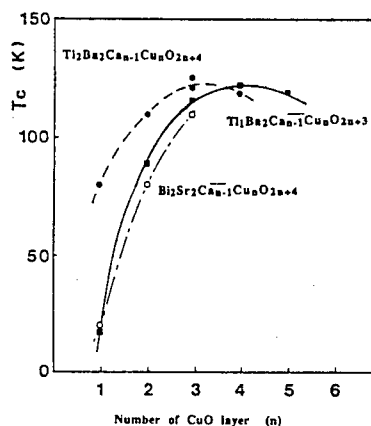
Fig. 10 T_c values versus the number ( n ) of Cu-O layers of \text{TiBa}_2\text{Ca}_{n-1}\text{Cu}_n\text{O}_{2n+3} compounds compared with \text{Ti}_2\text{Ba}_2\text{Ca}_{n-1}\text{Cu}_n\text{O}_{2n+4} and \text{Bi}_2\text{Sr}_2\text{Ca}_{n-1}\text{Cu}_n\text{O}_{2n+4} compounds.
