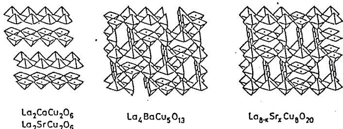
Fig. 6 Crystal structures of La_2SrCu_2O_6 , La_4BaCu_5O_{13-y} and La_{8-x}Sr_xCu_8O_{20-y} .
