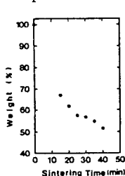
Fig. 1 Weight % ( W_{\text{sintered}}/W_{\text{initial}} ) of the sample pellet vs sintering time
