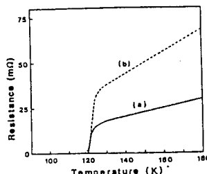
Fig. 3 Resistance versus temperature for the TlBa_2Ca_3Cu_4O_{11} sample.
