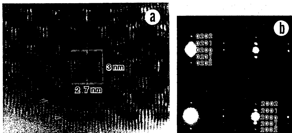
Fig.1 (a) A lattice image of \text{Bi}_2(\text{Sr,Ca})_3\text{Cu}_2\text{O}_x , taken by the incident beam parallel to the a axis. (b) A diffraction pattern, taken with the incident beam parallel to the c direction.
