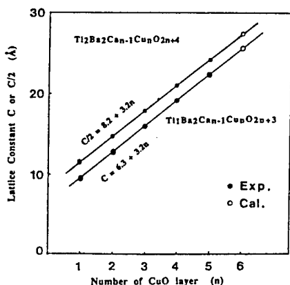
Fig. 9 The lattice constants c or c/2 versus the number of Cu-O layer for the \text{TiBa}_2\text{Ca}_{n-1}\text{Cu}_n\text{O}_{2n+3} or \text{Ti}_2\text{Ba}_2\text{Ca}_{n-1}\text{Cu}_n\text{O}_{2n+4} compounds, respectively. The lines are c=6.3+3.2n and c/2=8.2+3.2n . The filled circles are experimental ones and the open circles are calculated ones.
