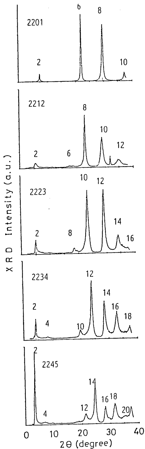
Figure 2 X-ray (Cu K\alpha ) diffraction pattern of the as-deposited multilayered films ( T_s=650^\circ\text{C} ), simulated to the 2201, 2212, 2223, 2234 and 2245 phases, respectively. The integer Q marked on the diffraction lines represents the index Q of the diffraction line arising from (00 Q ) planes.
