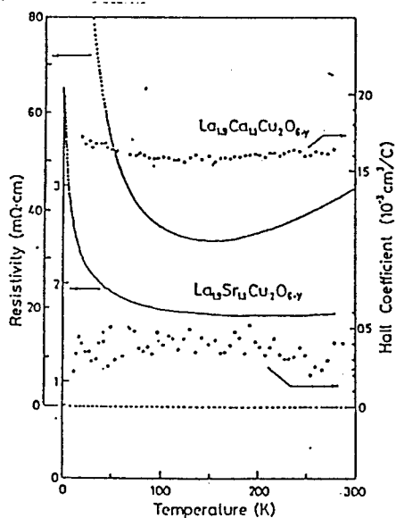
Fig. 7 Resistivity and Hall coefficient of La_{1.9}Ca_{0.1}Cu_2O_{6+y} and La_{1.9}Sr_{0.1}Cu_2O_{6+y} .
