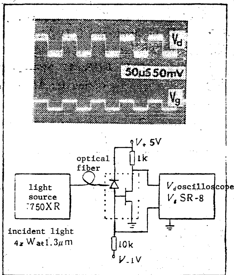
Figure 5. Measured Photodetection Characteristics of Monolithic Integrated Photoreceiver and Schematic of Measurement System
