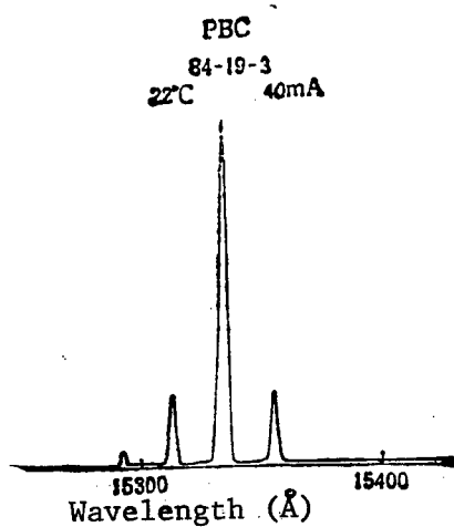
Figure 5. Emission Spectrum
