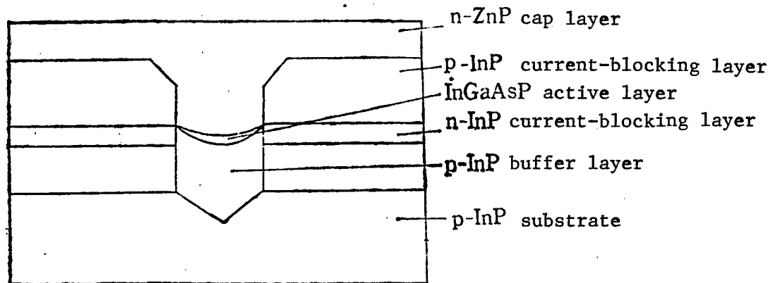
Figure 1. Structure of p-Substrate Buried Crescent (PBC) Laser
