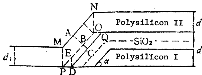
Figure 6. Profile of Double-Layer Polysilicon Structure With Sloped Polysilicon-I Sidewall
