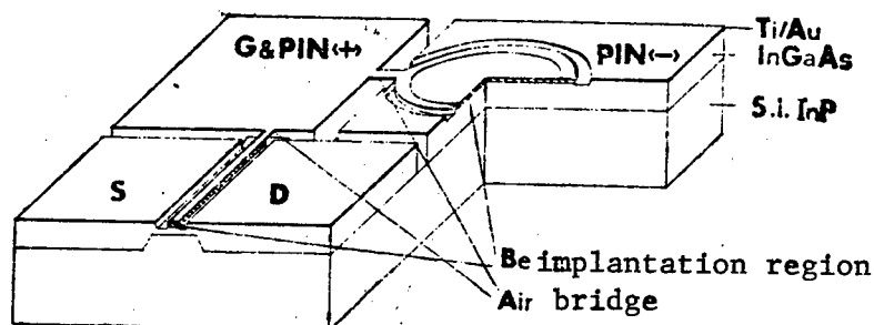
Figure 2. Structure of Quasiplanar Monolithic Integrated InGaAs PIN-JFET Photoreceiver
