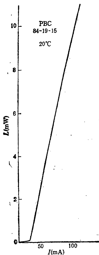
Figure 3. Light Output vs Current
