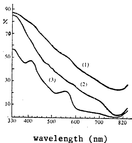
Figure 6. Absorptance Curves of the Whole Skin, Epidermis and Dermis; Sample From the Outer Leg
