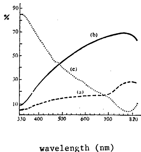
Figure 1. Reflectance, Transmittance and Absorptance Curves of the Epidermis on the Skin From the Outside Leg
