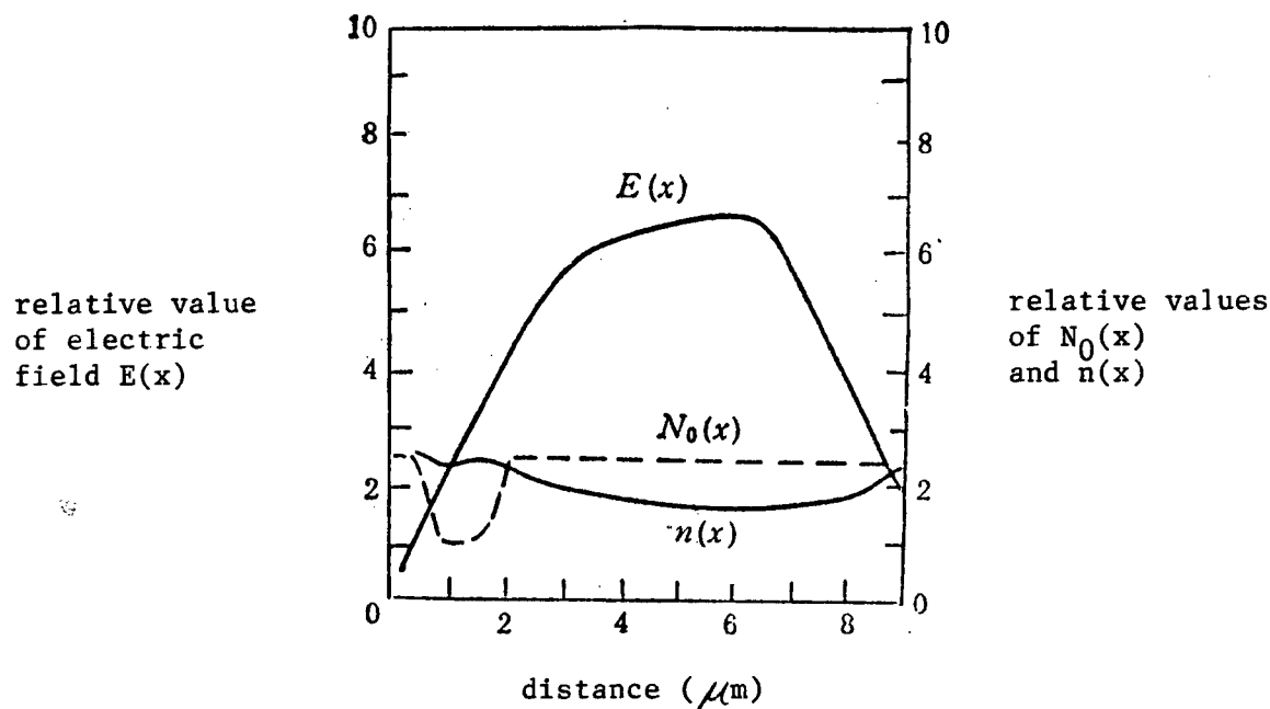
Figure 3. Electric Field and Concentration Distributions in a Stationary Domain Formed at a Deep Notch
