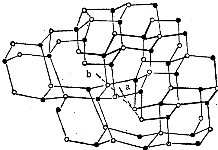
Figure 8. Lattice Model of GaAs with two edge dislocations. a is direction of dislocation, b is direction of Burger vector, and slip plane is (100).
