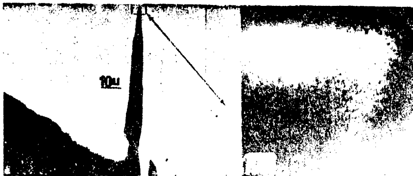
Figure 6. Electron micrographs of the ground/space interface in single crystal B.
