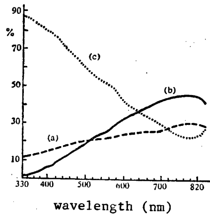
Figure 3. Reflectance, Transmittance and Absorptance Curves of the Whole Skin From the Outside Leg
