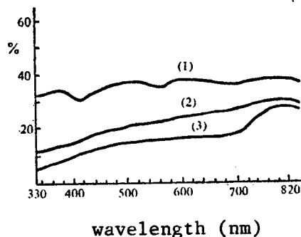
Figure 4. Reflectance Curves of Dermis, the Whole Skin and Epidermis of Sample From the Outer Leg
