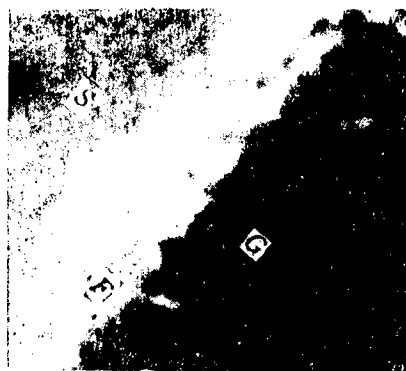
Figure 7(a). Cathodoluminescence of the interface in single crystal A. F is the interface, G is the seed-crystal region, and S is the space-grown material (X200).
