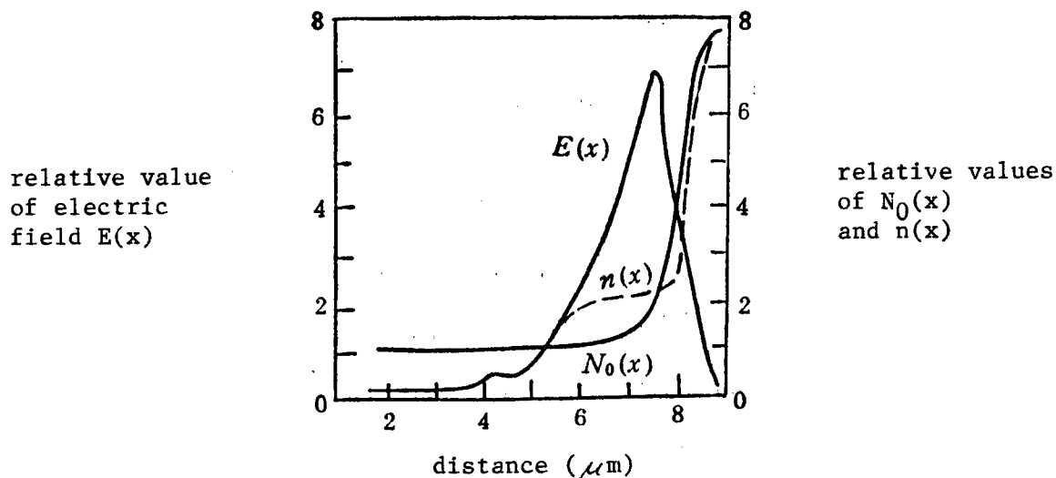
Figure 2. Electric Field and Concentration Distributions in a Stationary Domain Formed at the Anode
