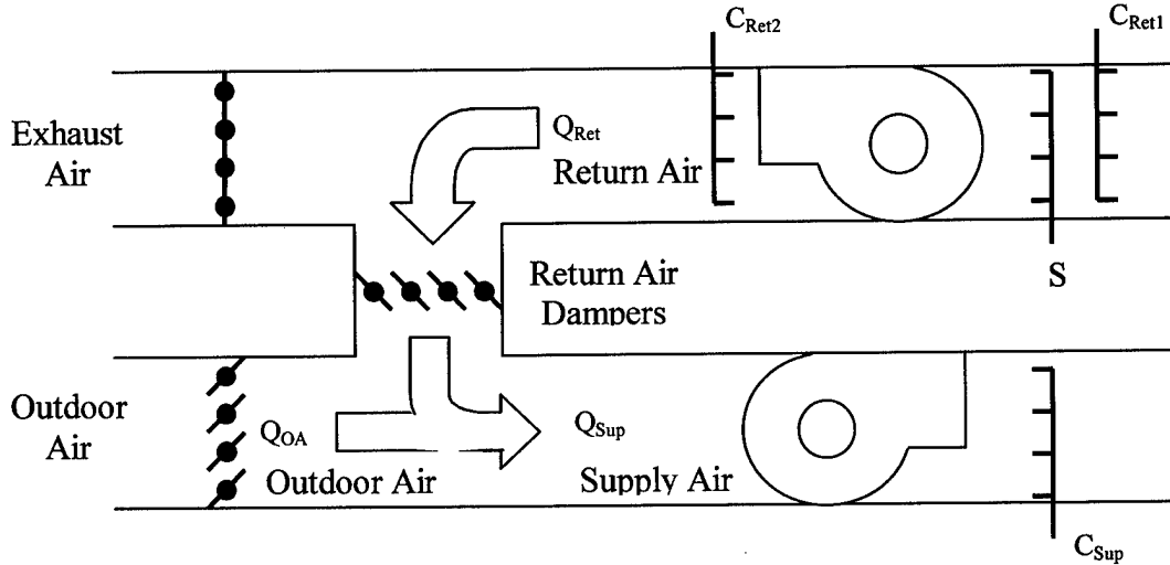
Figure E1 – Air-Handler OA Flow Rate Measurement - Tracer Gas with Return Air
