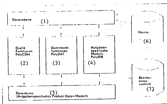
Figure 1. Schematic Buildup of PolyCAD
