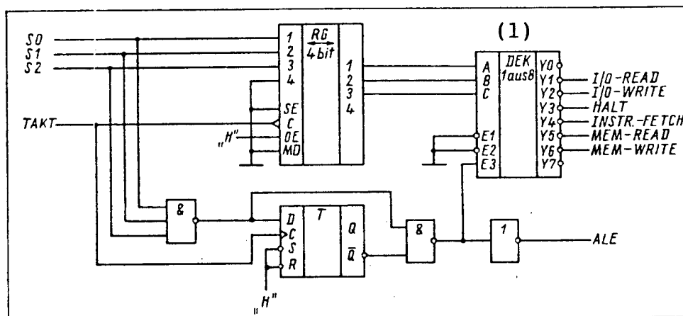
Figure 2: Circuit for the bus control
