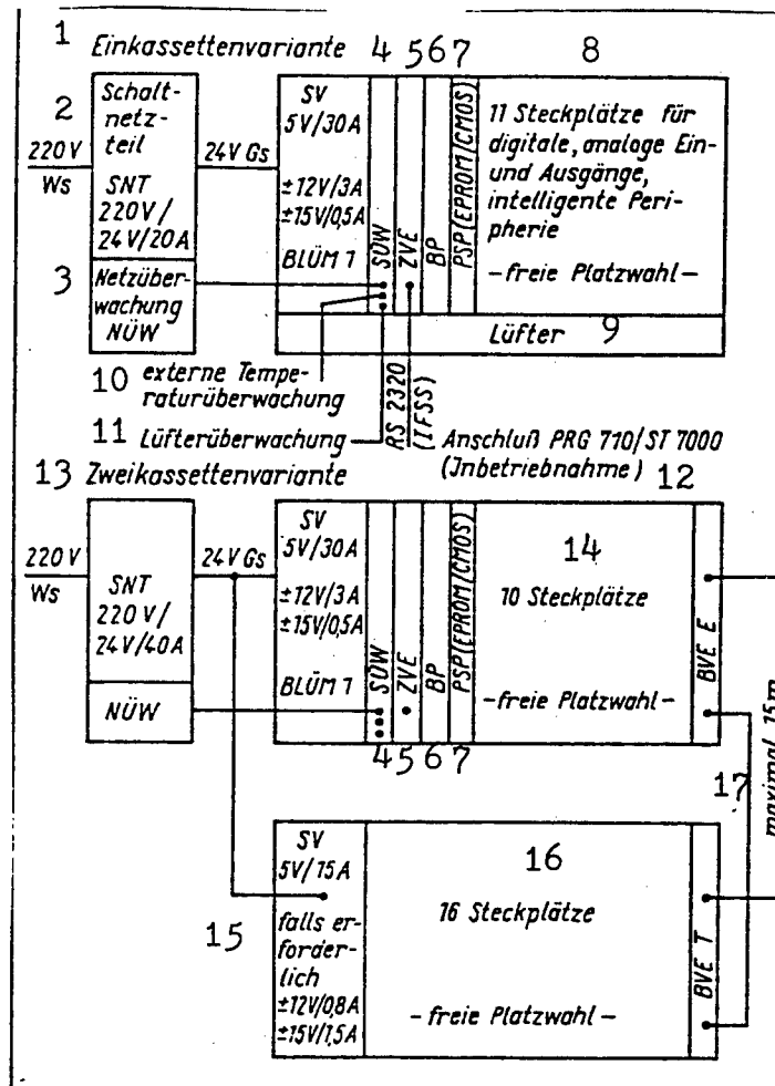
Fig. 2. One-Expansion-Chassis and Two-Expansion-Chassis Variants of the SPS 7000
