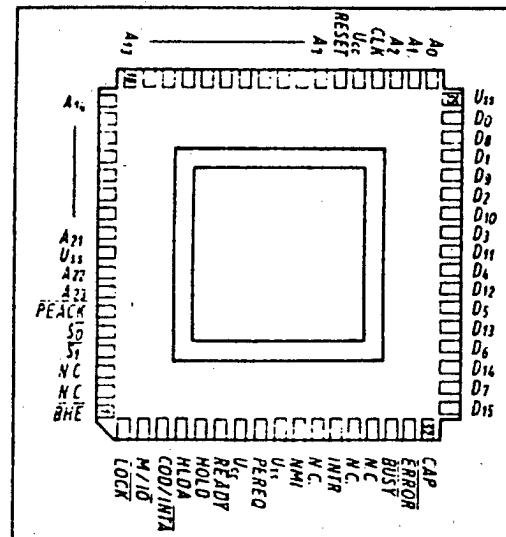
Figure 4. Pin assignment
