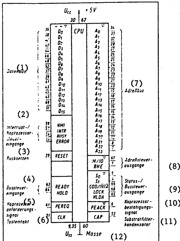
Figure 3. Diagram of the U80601
