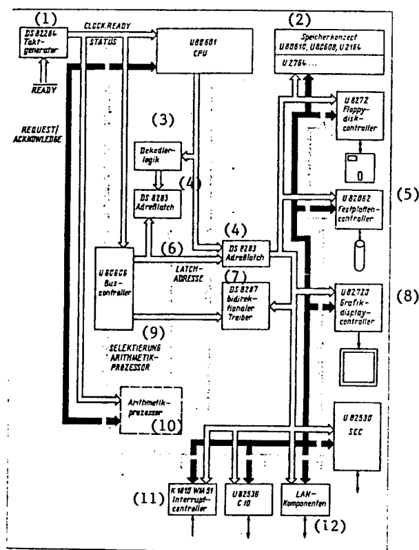
Figure 1. U80600 system configuration
