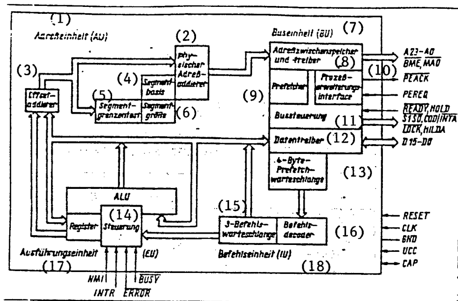
Figure 1. Block diagram of the U80601
