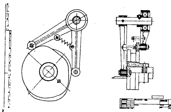
Figure 2. Drawing produced with PolyCAD (sector)
