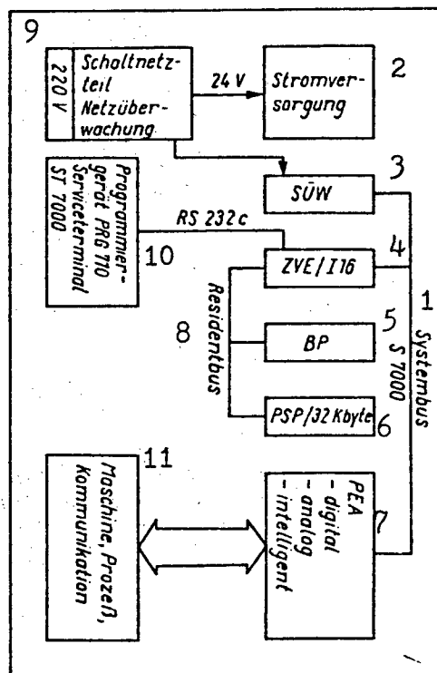
Fig. 1. Structure of the SPS 7000
