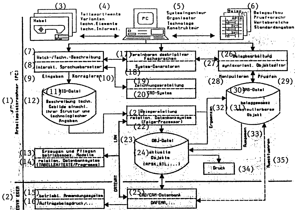
Figure 2. Structure and Functions of RTV 2000
