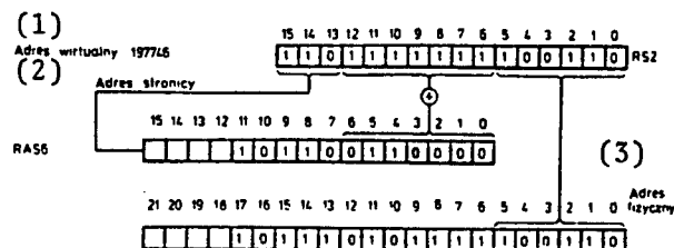
Figure 3. Diagram of physical address generation.
