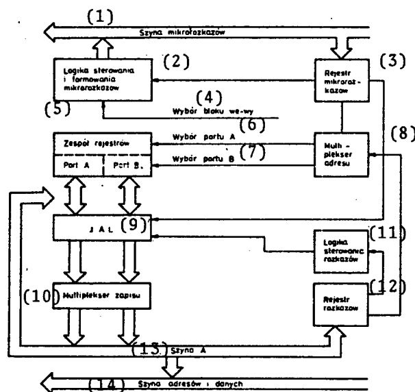
Figure 2. Block diagram of processing.
