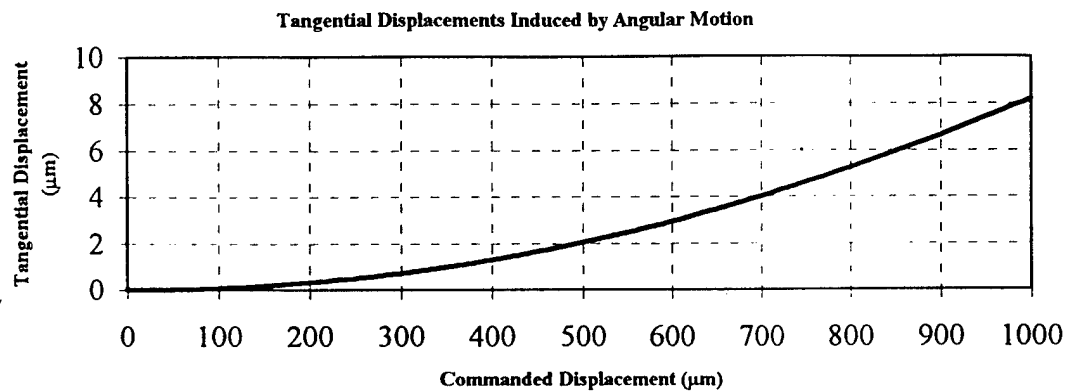
Figure 3.9: Quantification of the Tangential Motion of the Indentor when a Normal Motion is Desired
