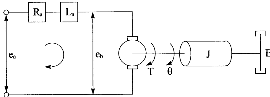
Figure 3.4: Schematic of the DC Motor
