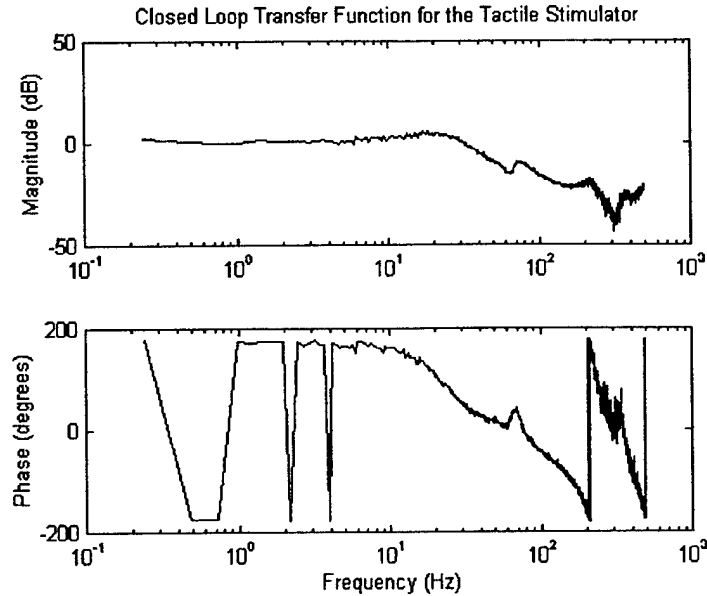
Figure 3.7: Bode Plot of the Closed Loop Transfer Function of the Tactile Stimulator System
