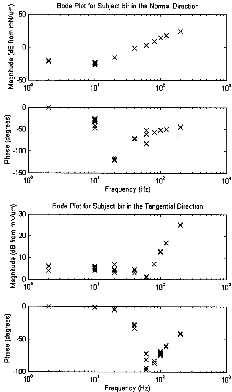
Figure 5.4: Normal and Tangential Transfer Functions for subject bir, all data points
