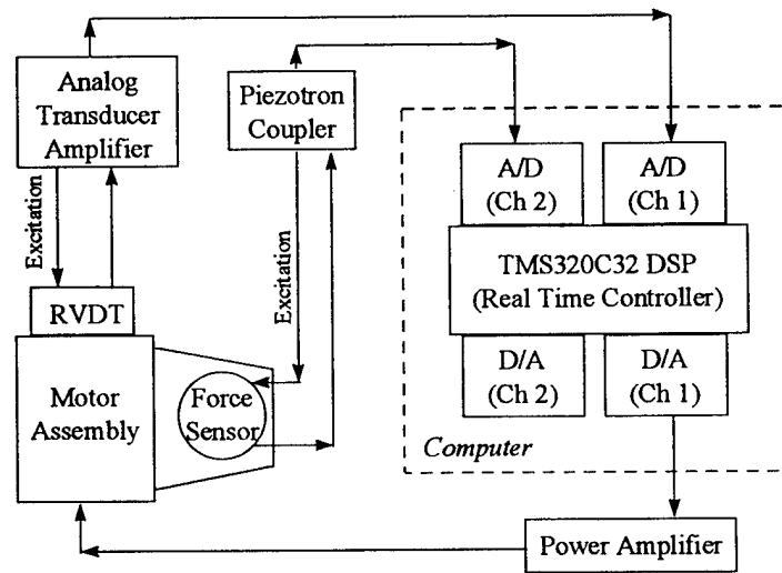
Figure 3.2: Signal Flow Diagram of the Tactile Stimulator System
