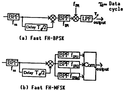
Figure 1. Block Diagrams of Differential Despreading System
