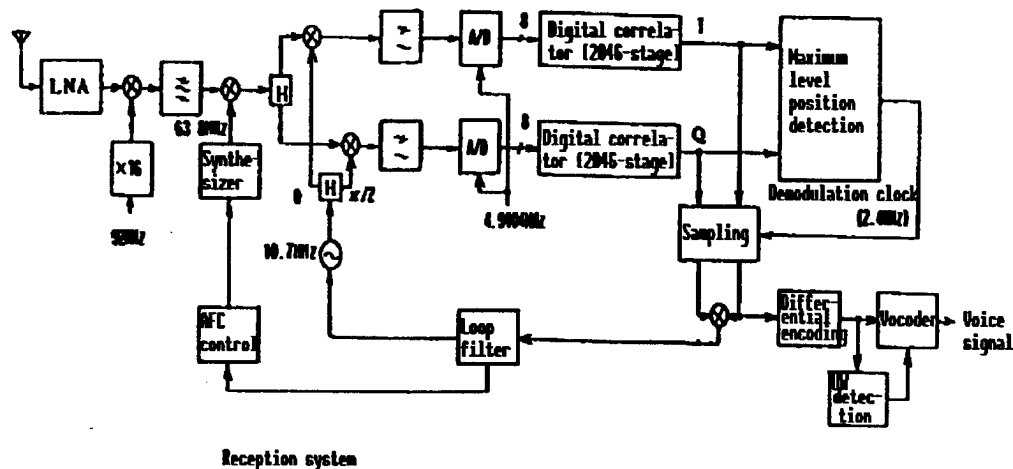
Figure 1. Configuration of Spread-Spectrum Communications Equipment for Mobile Satellite Communications
