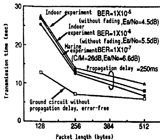
Figure 3. Average Transmission Time
