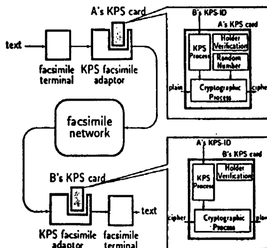
Figure 3. Example of Cryptographic Communications System Using KPSL1CARD Cards
