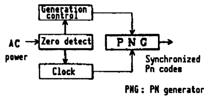
Figure 1. Power-Synchronized PN Code Generator
