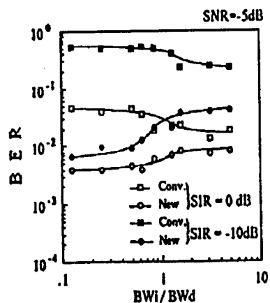
Figure 3. Relationship Between Normalized Interference Band and Bit Error Rate
