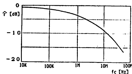
Figure 2. Degradation of Correlation Value f
