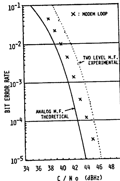
Figure 1. Bit Error Characteristics
