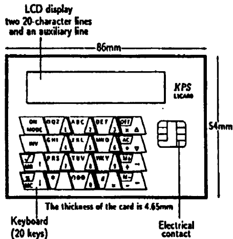
Figure 1. External Configuration of KPSL1CARD
