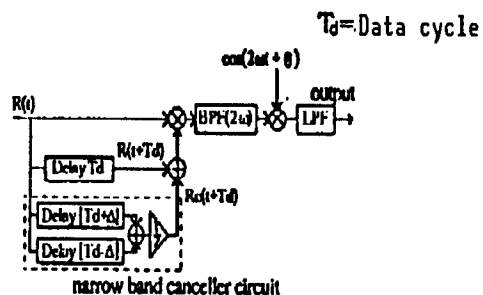
Figure 2. Block Diagram of Differential Despreader With Narrow-Band Interference Canceller Circuit
