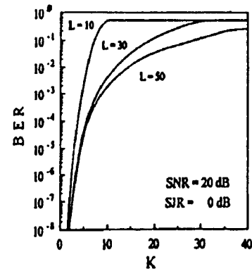
Figure 4. Error Rate Vs. Number of Interfering Stations
