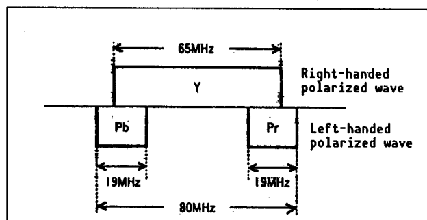
Figure 4. Frequency Allocation of FPU for Wireless Camera
