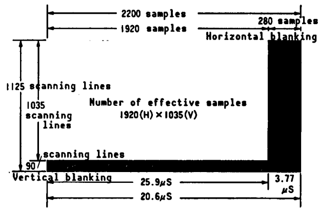
Figure 2. Screen Structure of HDTV Standard
