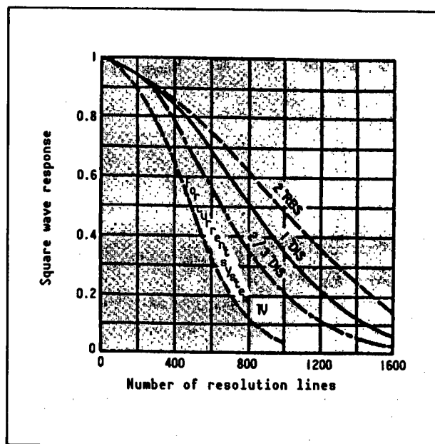
Figure 1. Resolution Characteristics of Various Camera Tubes
