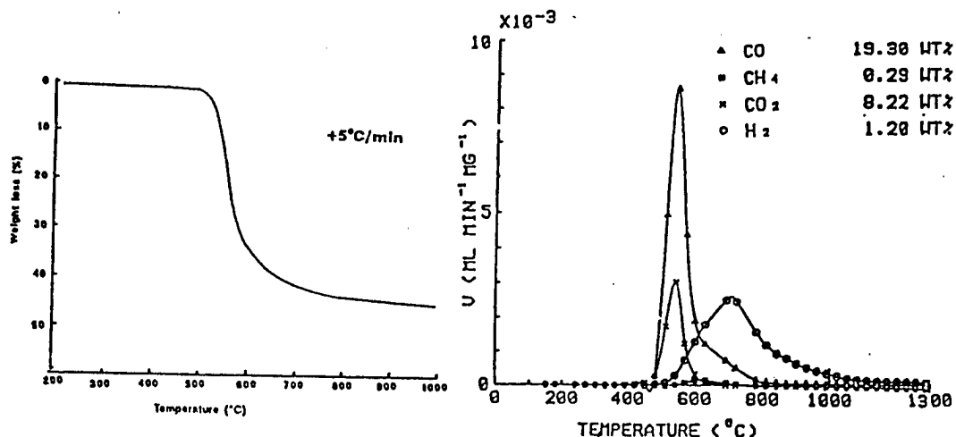
Figure 3. (a) TGA, (b) Analysis of Gaseous Products
