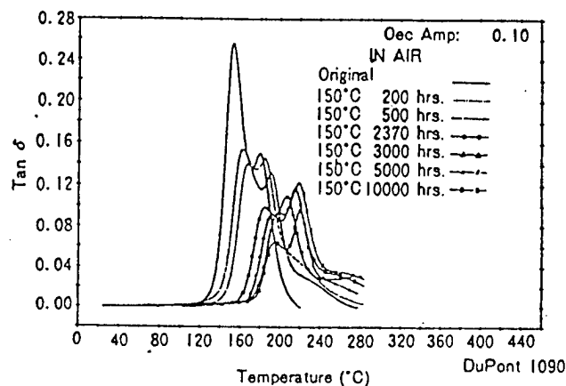
Figure 5. \tan \delta of Thermal Aging CFRP
