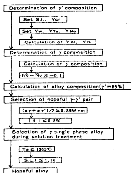
Figure 2. Flow Chart of Alloy Design for Ni-Cr-Al-W-Ta-Mo Series
