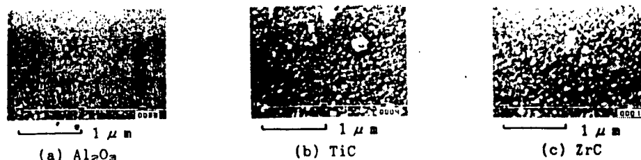
Fig.6 SEM Photographs of prepared fine particles at P_t = 100\text{Torr} .
