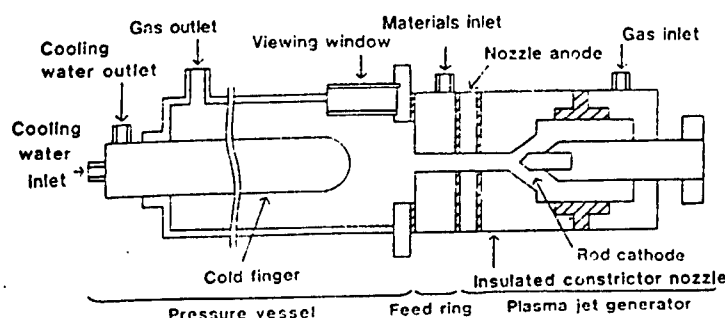
Figure 1. Schematic Diagram of the Plasma Jet Reactor System, Where the Forced Constricted Type Plasma Jet Generator Is Equipped
