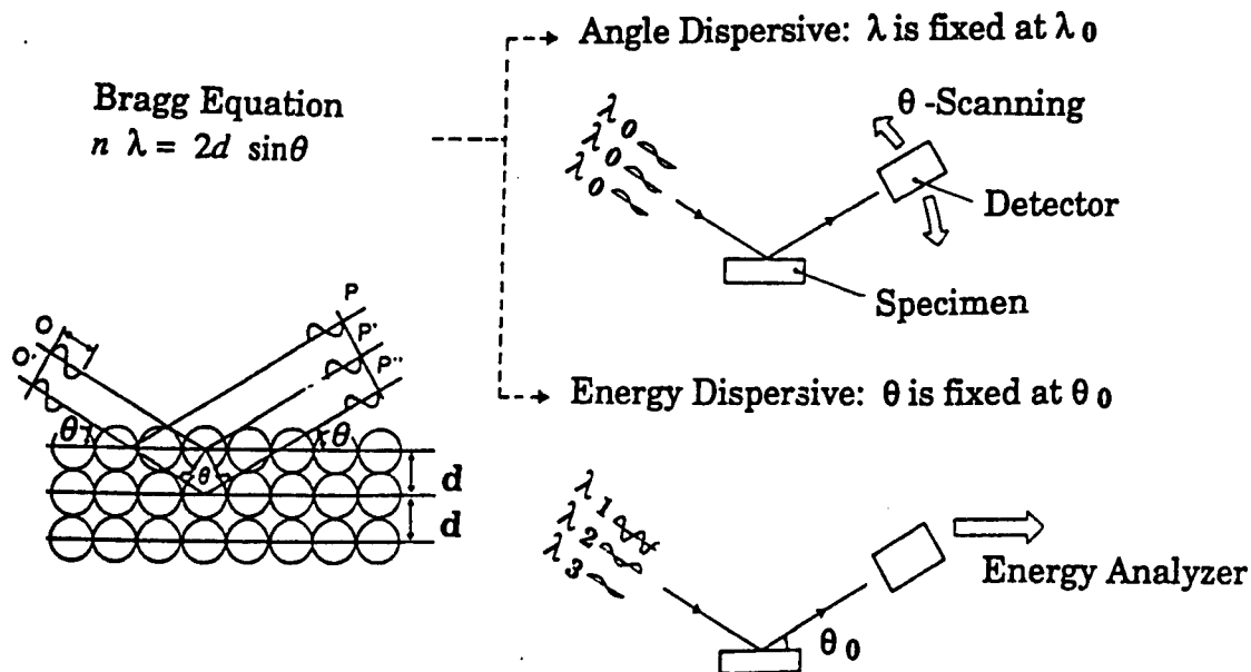
Figure 2. The Principle of X-Ray Diffraction
