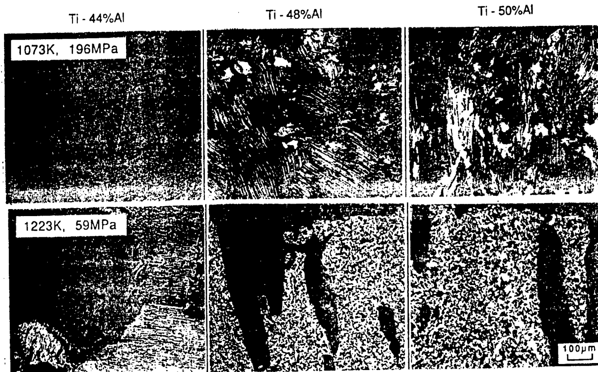
Photo 4. Microstructure and Crack/Void Appearance Near Creep Ruptured Surface
