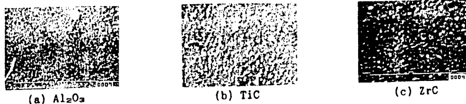
Fig.5 SEM Photographs of prepared fine particles at P_t = 760\text{Torr} .
