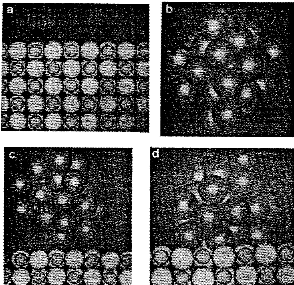
Figure 9. Computer Graphic Images of MgO (100) Plane (a), \text{Au}_{32} Cluster (b), and Process for Fixation of \text{Au}_{32} Cluster on MgO (100) Plane (c),(d)
