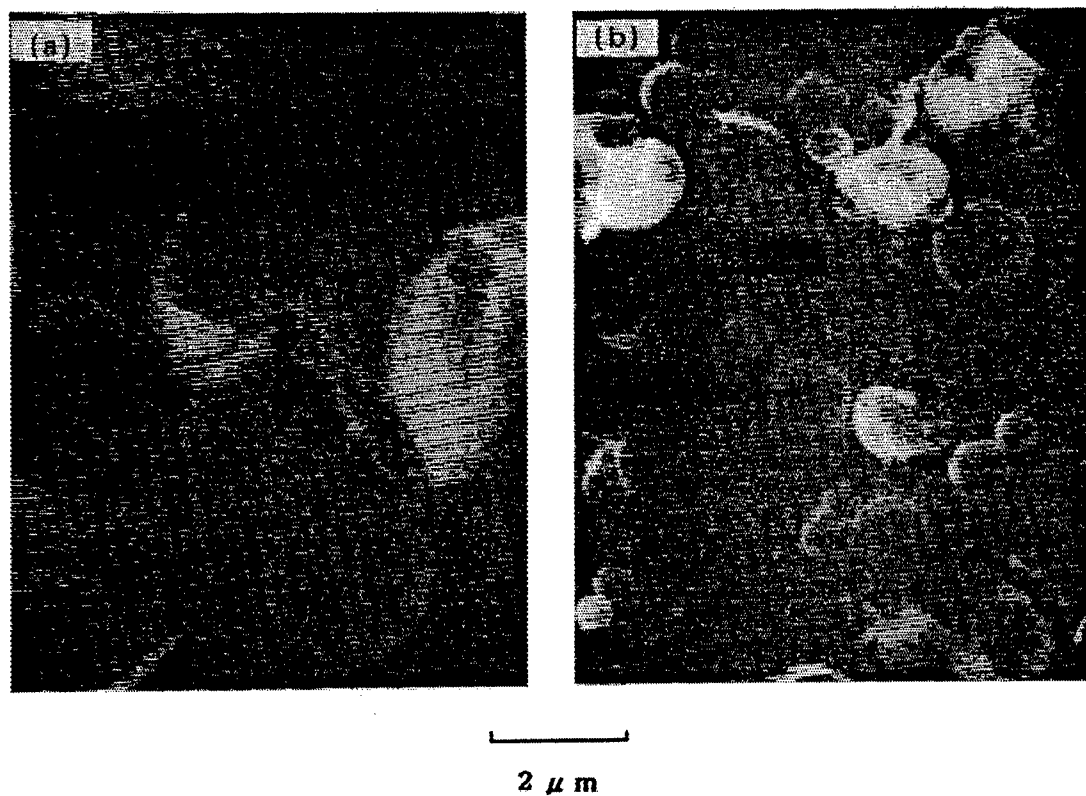
Figure 5. Effect of Air Flow on Morphological Changes of Grains of 2mol%Y 2 O 3 -ZrO 2 Synthesized Powder
