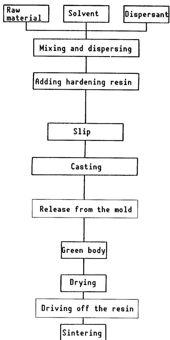
Figure 1. Manufacturing Process
