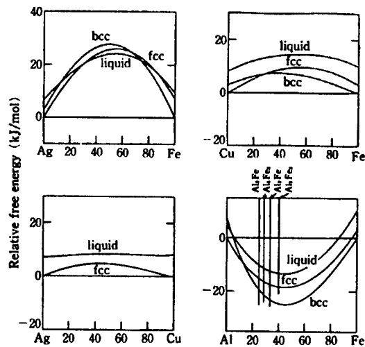
Figure 6. Relative Value of Free Energy at 500 K for Various Phases in Ag-Fe, Cu-Fe, Ag-Cu, and Al-Fe Alloys. The diagrams are plotted using mixtures of the powders for the elements as the standard line.
