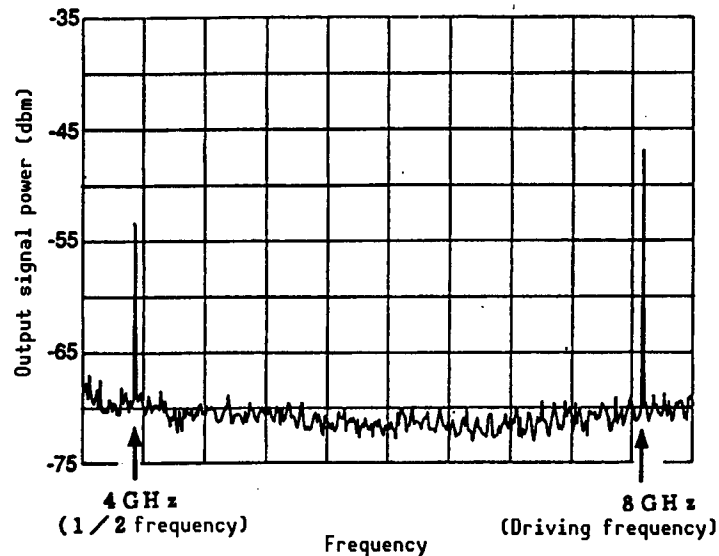
Figure 5. Frequency Analysis Result of High Frequency Operation
