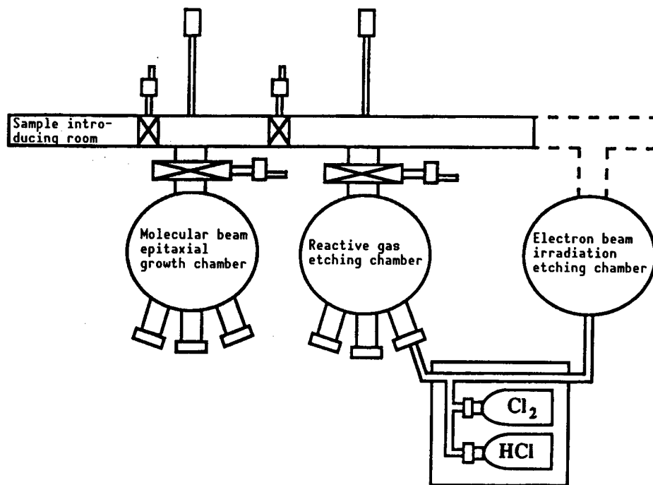
Figure 6. Ultrahigh Vacuum Through System
