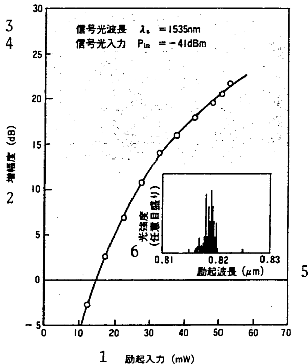
Figure 4. Amplification Characteristics of 0.8 \mu\text{m} Band Key:—1. Excitation input—2. Amplification degree (dB)—3. Signal light wavelength—4. Signal light input—5. Excitation wavelength ( \mu\text{m} )—6. Light intensity (arbitrary scale)
