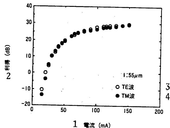
Figure 2. Amplification Characteristics of Semiconductor Optical Amplifier Element (current dependence of TE and TM wave gains)
