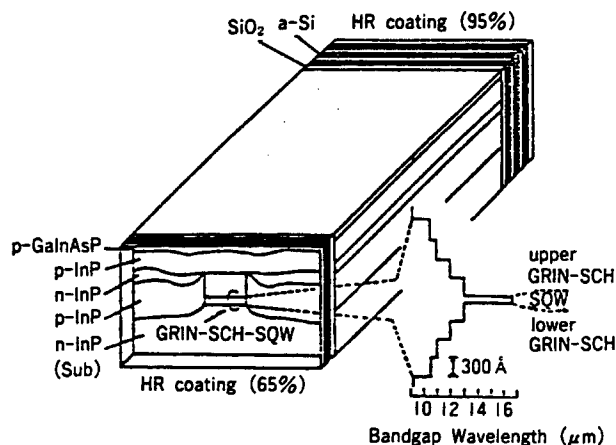
Figure 8. GRIN-SCH-SQW LD
