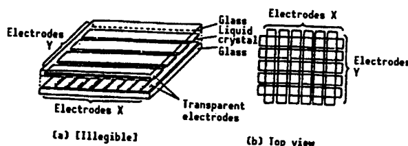
Figure 9. Structure of Large-Scale Simple Matrix System: Two sets of transparent electrodes are arranged to cross at right angles, with the liquid crystal, covered by glass, in the middle.
