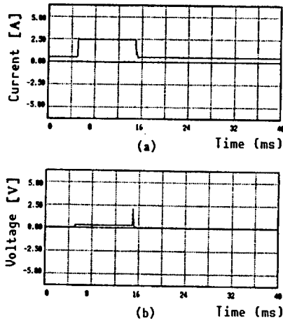
Figure 1. Switching Characteristics (a) Current waveform (b) Voltage waveform
