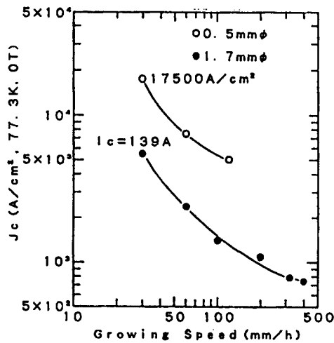
Figure 1. Relationship Between J_c and Growing Speed After Annealing
