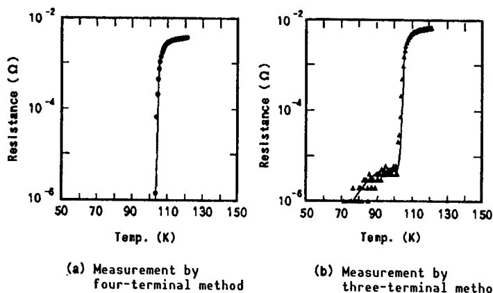
Figure 2. Results of Measurement of Critical Temperature and Connection Resistance
