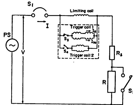
Figure 3. Operating Characteristics
