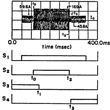
Figure 2. Test Circuit
