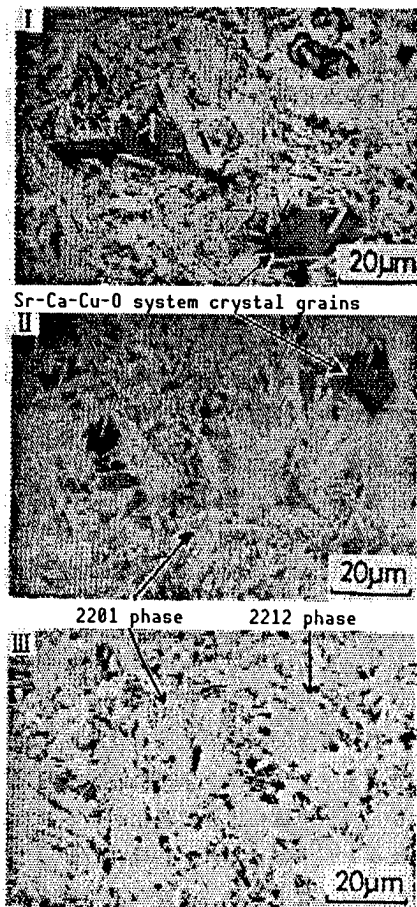
Figure 1. SEM (BEI) Image of Each Specimen
