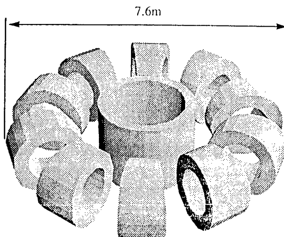
Figure 1. Hybrid SMES
