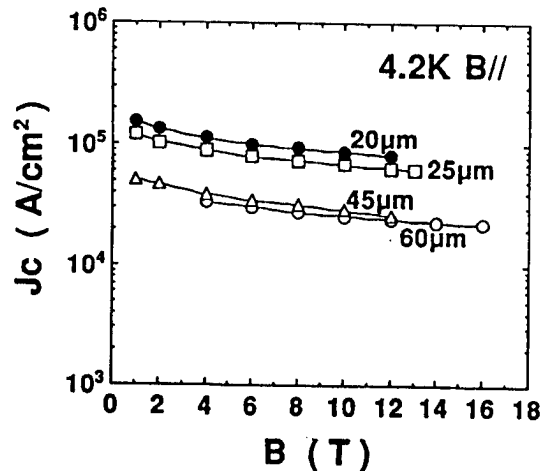
Figure 2. J_c -B Characteristics Based on SC Core Thickness
