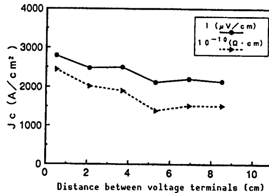
Figure 2. Relationship Between Inter-Voltage Terminal Distance and J_c (Tape thickness: 0.2 mm)
