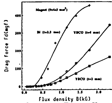
Figure 2. Drag Force Versus Flux Density
