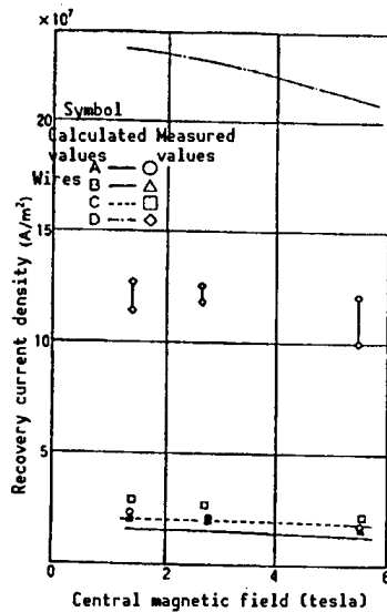
Figure 2. Results of Recovery Current Measurement
