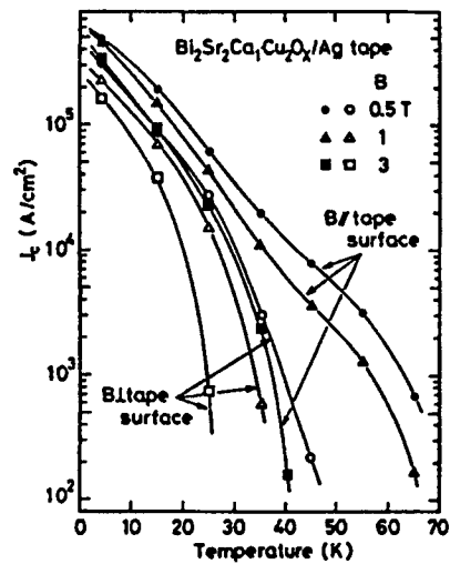
Figure 2. Temperature Dependence of J_c Obtained by dc Magnetization
