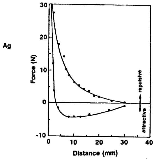
Figure 2. Relationship Between Flotation Force and Distance
