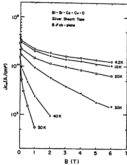
Figure 1. J_{c_{sc}}-B Characteristics of Bi-Based Tape
