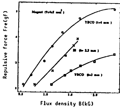
Figure 3. Repulsive Force Versus Flux Density
