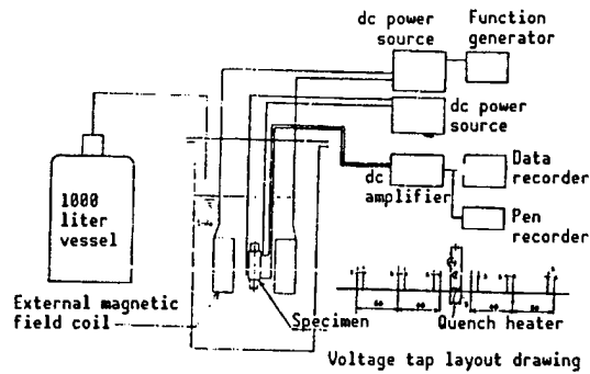
Figure 1. Test System
