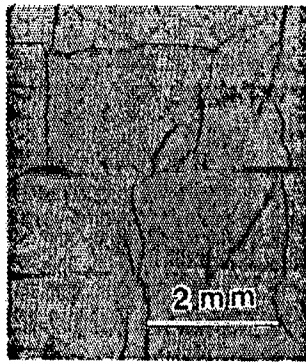
Figure 1. Structure of Lap-Quenched Antecedent Part
