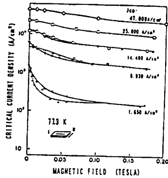
Figure 2. History Effects of Ag/BiPbSrCaCuO
