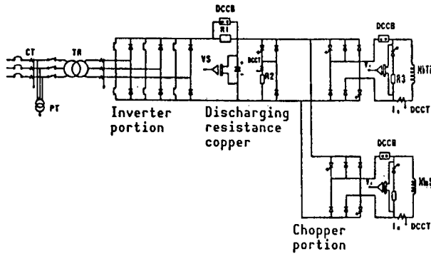
Figure 1. Principle-Demonstration System
