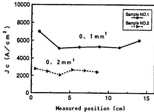
Figure 1. Distribution of J_c of \text{Bi}_2\text{Sr}_2\text{CaCu}_2\text{O}_x System Ag-sheathed Tape Wire in Longitudinal Direction
