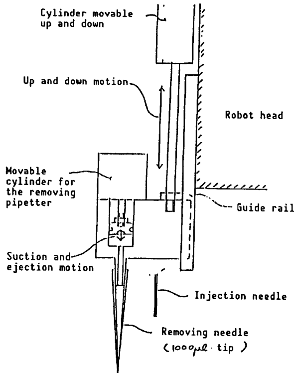
Figure 10. Removing Pipetter
