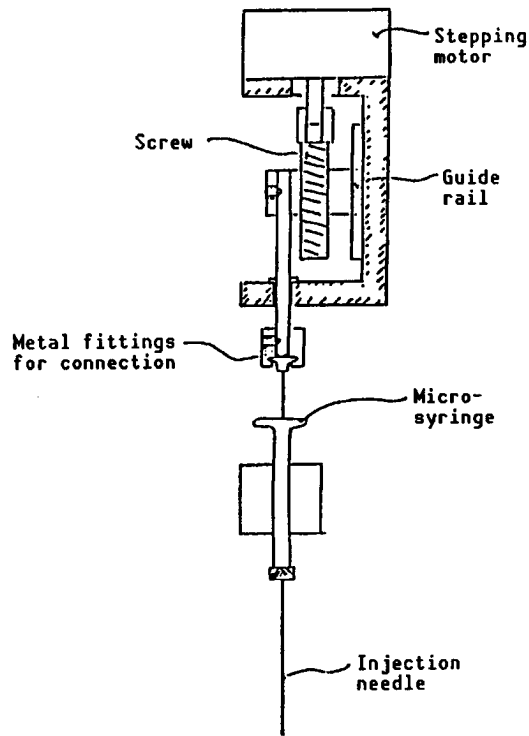
Figure 8. Injection Pipetter
