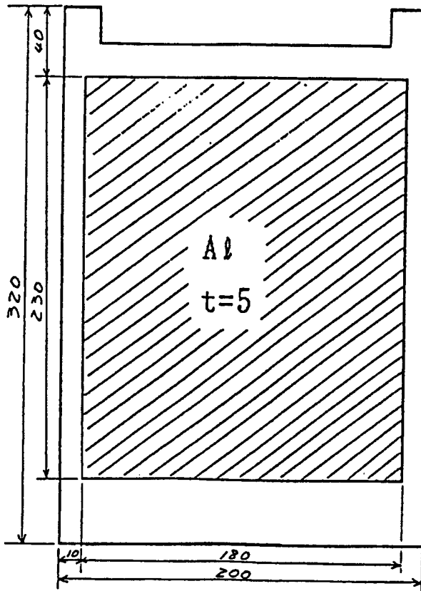
Figure 20. Outside Shape of Plate (With radiation plate)
