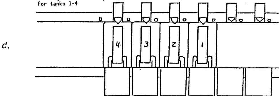
Figure 14. Conveyance Method During Prerunning
