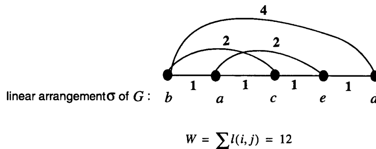
Figure 4.2: An assignment of lengths to the edges of G .
