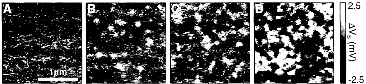
Fig. 4. Photoactivity of single dopant atoms and surface traps shown in xy maps of changes in V_s ( \Delta V_s ), induced by exposure to (A) no light and light at (B) 850 nm, (C) 770 nm, and (D) 690 nm. Individual photo-ionized (neutralized) sites with a single-electron charge are seen as light (dark) spots; that is, light spots mark new positive charges, and dark spots, new negative charges. The sensitivity of the color scale is about an order of magnitude greater than that in Fig. 3.
