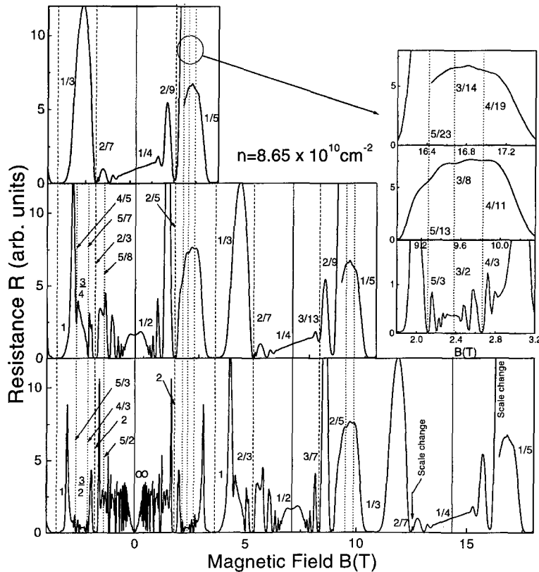
Fig. 1. Magneto-resistance of a high-mobility, two-dimensional electron gas at T \sim 25 mK. The middle and top sections of the main figure are offset by one and two-times the magnetic field corresponding to \nu = \frac{1}{2} and \nu = \frac{1}{4} . This figure shows many self-similarities inherent in such data. Vertical lines indicate but a few of such corresponding filling fractions. The inset shows weak features that are just becoming visible in the most recent specimens and their relationship to previously observed fractions.
