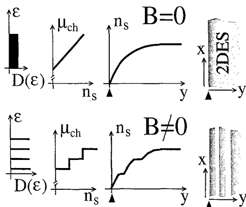
Fig. 1. Sketches of the density of states D(\varepsilon) versus single-particle energy \varepsilon , the chemical potential \mu_{\text{ch}} versus sheet electron concentration n_s , and the electron concentration profile at the edge of an idealized 2DES with and without magnetic field B .
