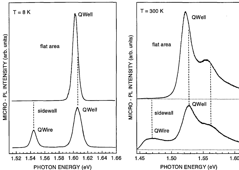
Fig. 5. Five \mu m-PL spectra taken at 8 K (left) and 300 K (right) from the flat area of the mesa (upper curves) and from the \{311\} sidewall (lower curves).
