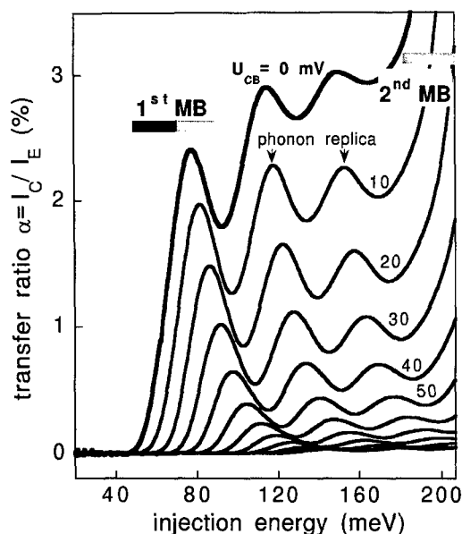
Fig. 6. Transfer ratio \alpha versus injection energy at different collector base voltages. The dark bars indicate the calculated position of the minibands. The gray bars represents the full-width at half-maximum of the injected electron energy distribution.
