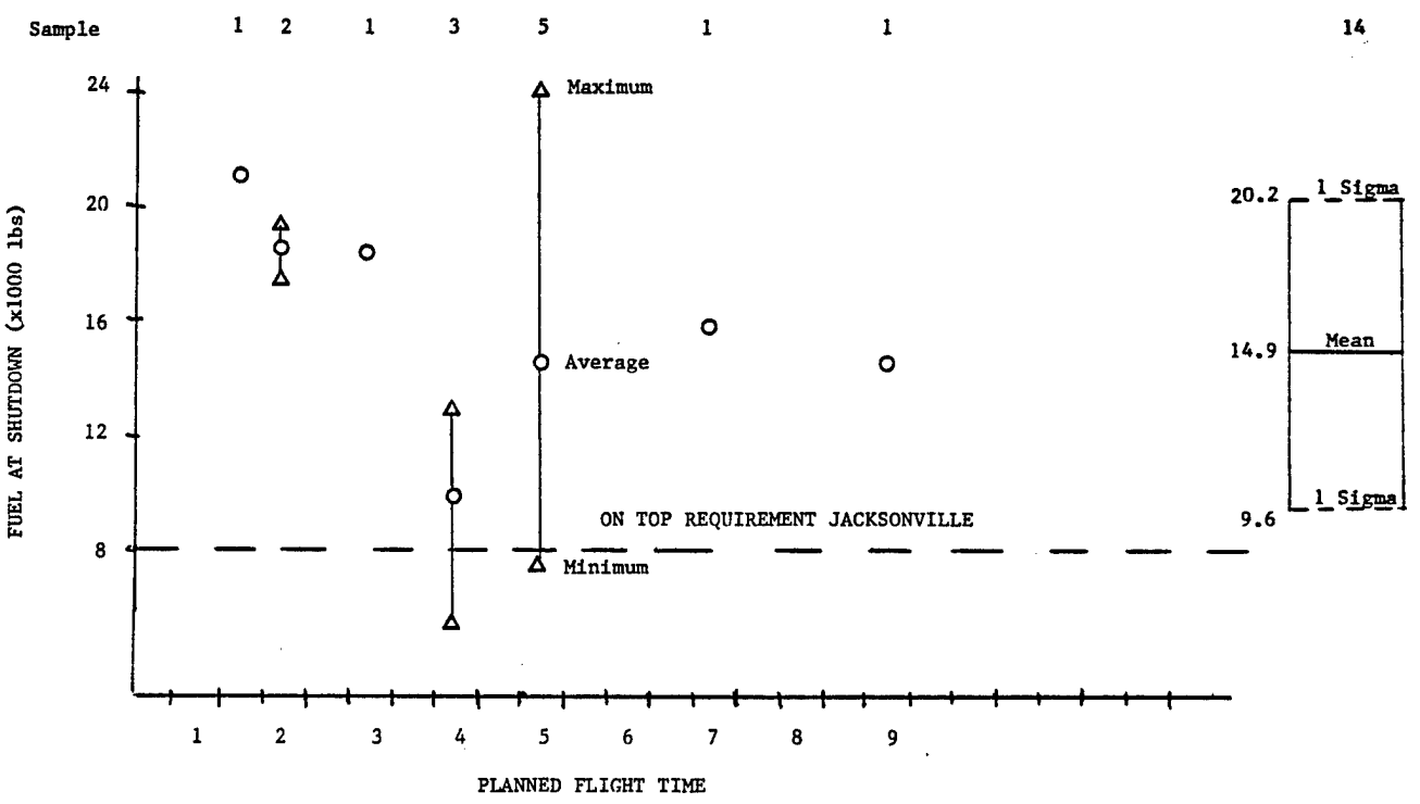
Figure 4-5 Squadron B November Fuel At Shutdown And Flight Time
