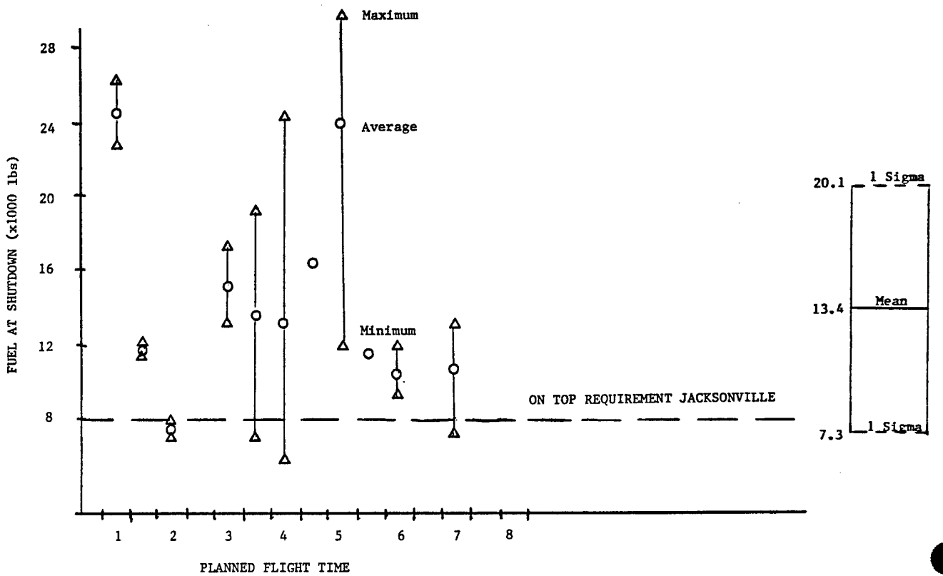
Figure 4-8 Squadron C January Fuel At Shutdown And Flight Time
