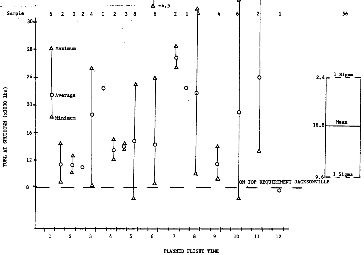
Figure 4-7 Squadron B January Fuel At Shutdown And Flight Time
