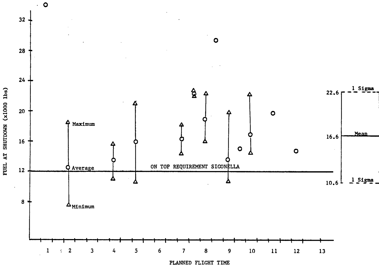
Figure 4-3 Squadron A December Fuel At Shutdown And Flight Time
