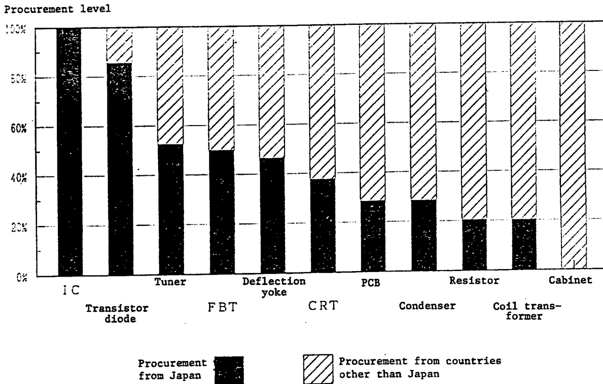
Figure 6. Levels of Parts Procurements From Japan in Overseas Production of Color TVs (by two major Japanese firms)
