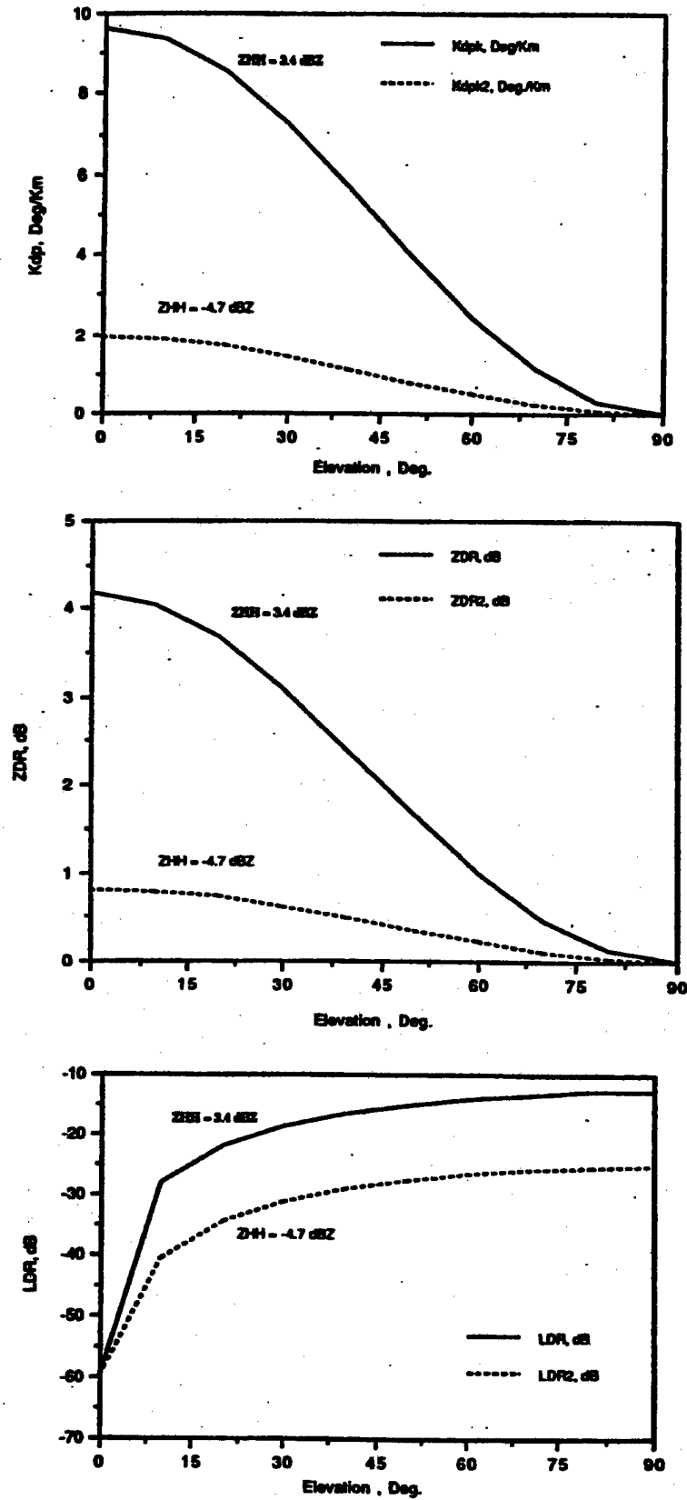
Figure 1.4: Same as Figure 1.3 except for needles. (From Evans and Vivekanandan 1990)
