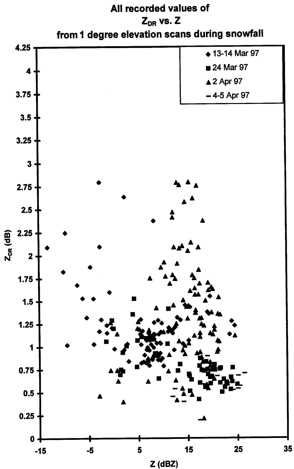
Figure 3.7: Z_{DR} vs. Z from 1 degree scans during all snowfall periods for 4 events.
