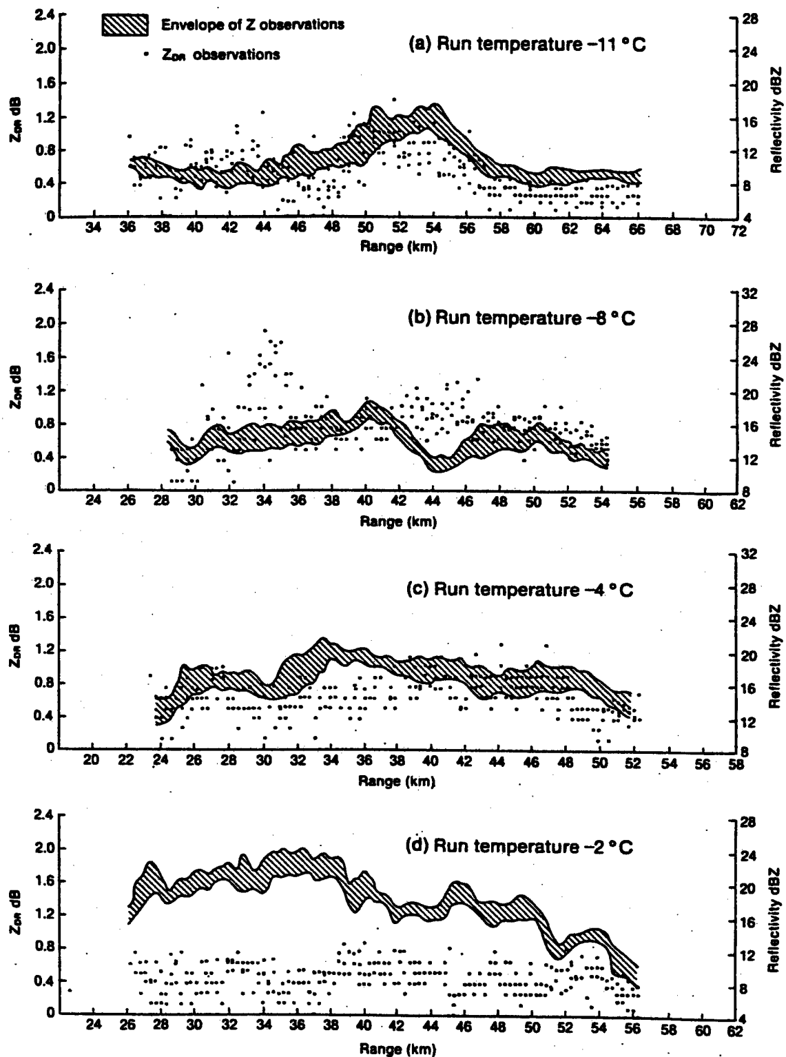
Figure 1.8: Z and Z_{\text{DR}} radar observations corresponding to four aircraft runs described in Table 1.3. (From Bader et al. 1987)
