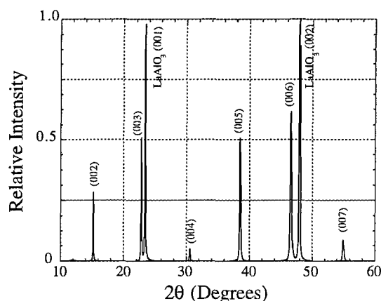
Figure 4. X-ray diffraction pattern showing the high crystalline quality c -axis orientation of the YBCO film on the (001) oriented single crystal LaAlO 3 substrate.
