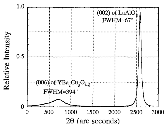
Figure 5. Two-crystal x-ray rocking curve spectrum of a YBCO film on an (001) oriented single crystal \text{LaAlO}_3 substrate. The 400 arc-second FWHM rocking curve width for the YBCO film indicates the single-crystal-like nature of the HTSC film.
