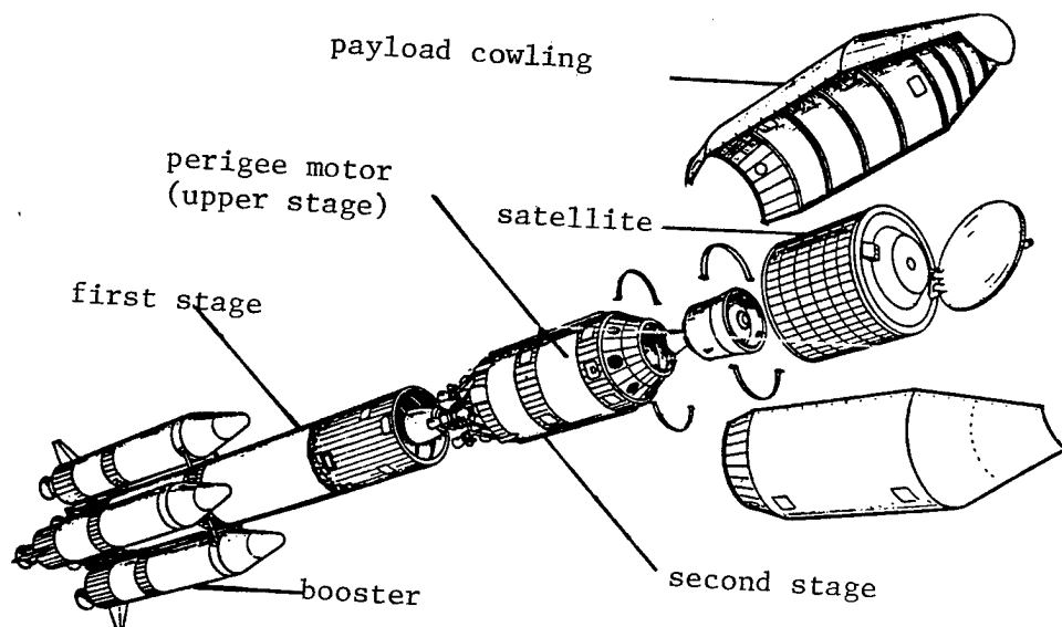
Figure 2. Payload Compartment of the Long March-2E
