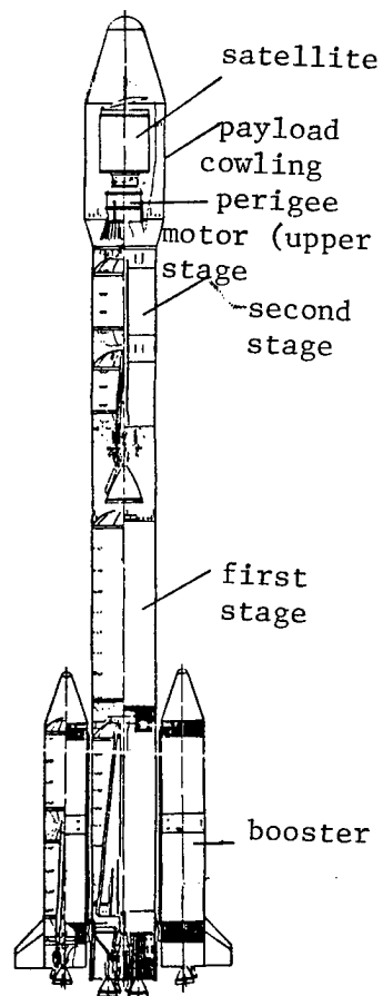
Figure 1: Components of the Long March-2E
