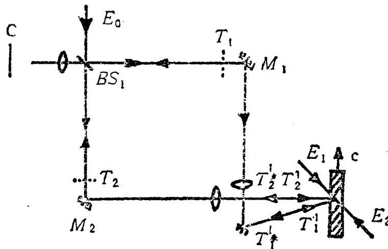
Figure 1. Principle of Real-Time Parallel Image Subtraction Using Mach-Zehnder Phase-Conjugate Six-Wave Mixing Technique
