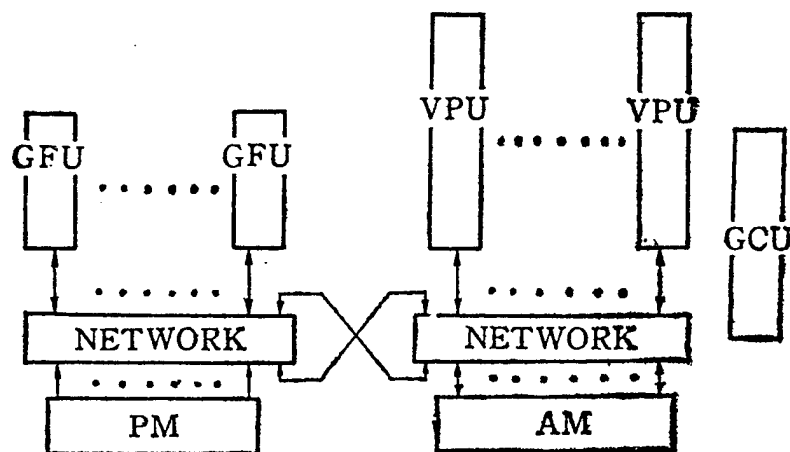
Figure 3.1. Structure of the SDS-1 System
