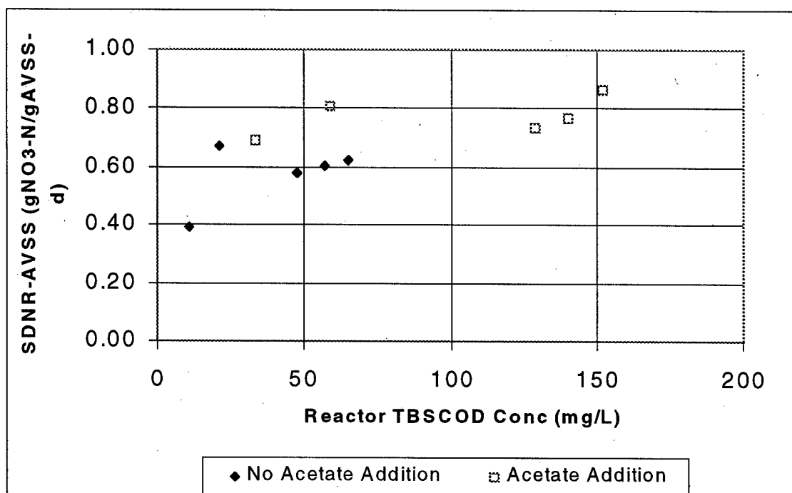
Figure 4.30 SDNR_{AVSS} (g NO 3 -N/g AVSS-d) versus Reactor TBSCOD Concentration (mg/L) after Correcting Raw Data for Temperature and Active Mass Fraction for all LOTT Test Runs
