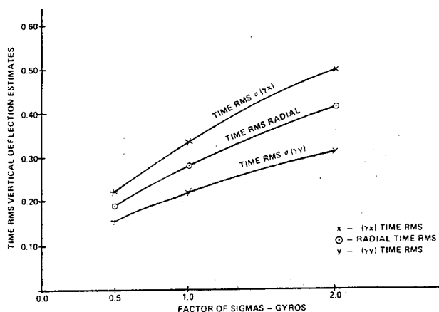
FIGURE 4— TIME RMS VERSUS FACTOR ON GYRO ERRORS
