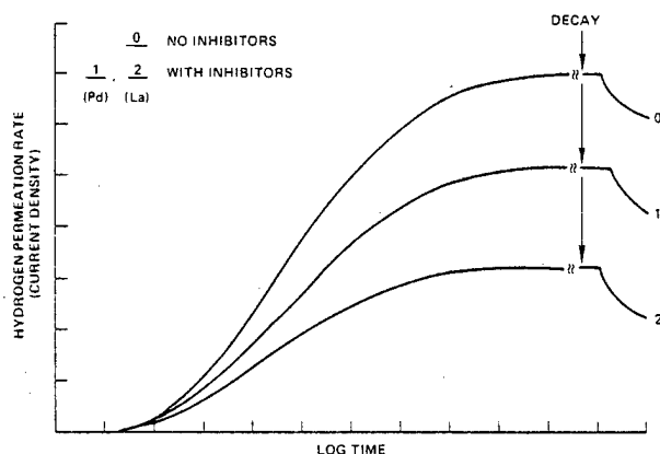
FIGURE 3 – EFFECT OF INHIBITORS ON HYDROGEN PERMEATION IN IRON
