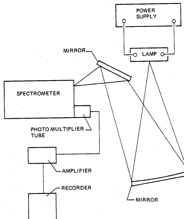
FIGURE 1 – SPECTROSCOPY APPARATUS
