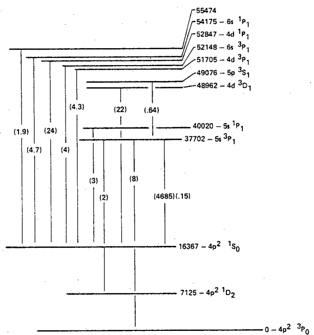
FIGURE 2 - Ge I
