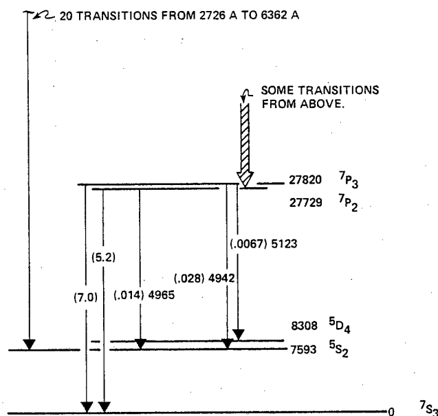
FIGURE 3 - Cr I
