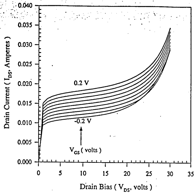
Fig. 2 : Pentode-like characteristics of the fabricated HJFET, W_m = W_t = 1\ \mu\text{m} , the gate-bias is increased in steps of 50\text{ mV} .
