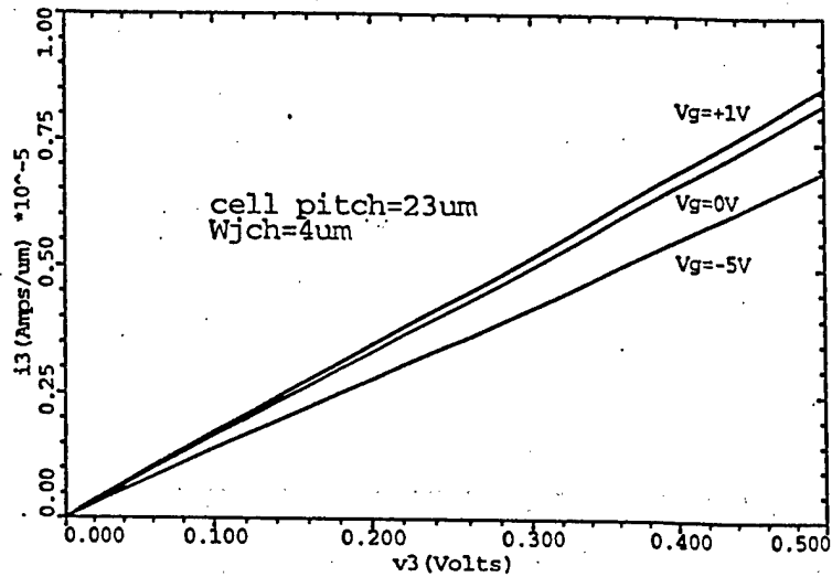
Fig.3 Simulated on-state I-V characteristics of the 6H-SiC JFET structure. (Dose= 1e13/\text{cm}^2 , W_{jch}=4\mu\text{m} )
