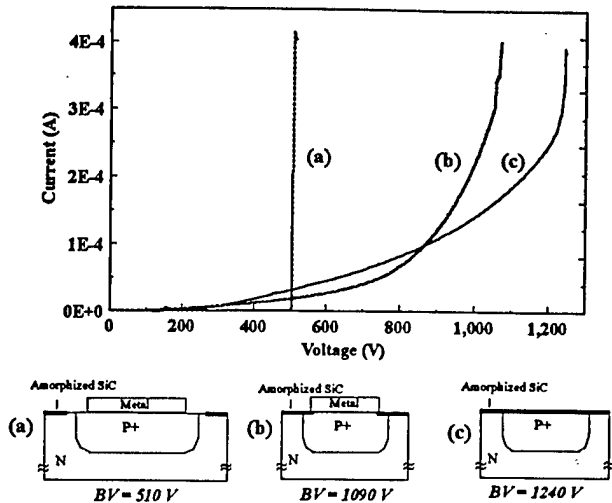
Fig. 7 Reverse I-V characteristics of the P^+/N diode of the ACCUFET with and without edge termination using amorphization. Breakdown voltage of upto 1240 V were measured after argon implant edge termination.
