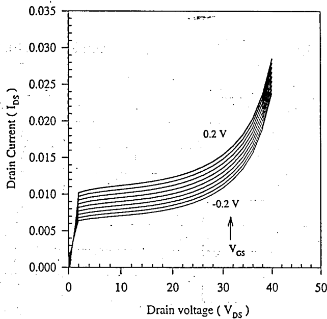
Fig. 3 : Pentode-like characteristics of the fabricated HJFET, W_m = 1, W_t = 3\ \mu\text{m} , the gate-bias is increased in steps of 50\text{ mV} .
