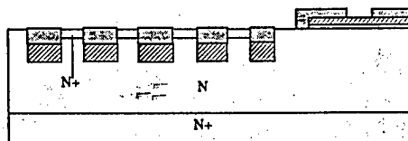
(g) After Contact etching
