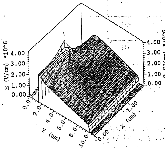
Fig. 13 ( b ) : Three-Dimensional Electric Field Distribution at V_{gs} = -25\text{ V} and V_{ds} = 1200\text{ V} for structure with W_m = 1.5\mu\text{m} and doping = 1 \times 10^{16}\text{ cm}^{-3} .
