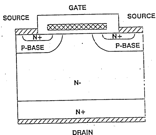
Fig.1 ( a ) : Cross Section Of a D-MOSFET
