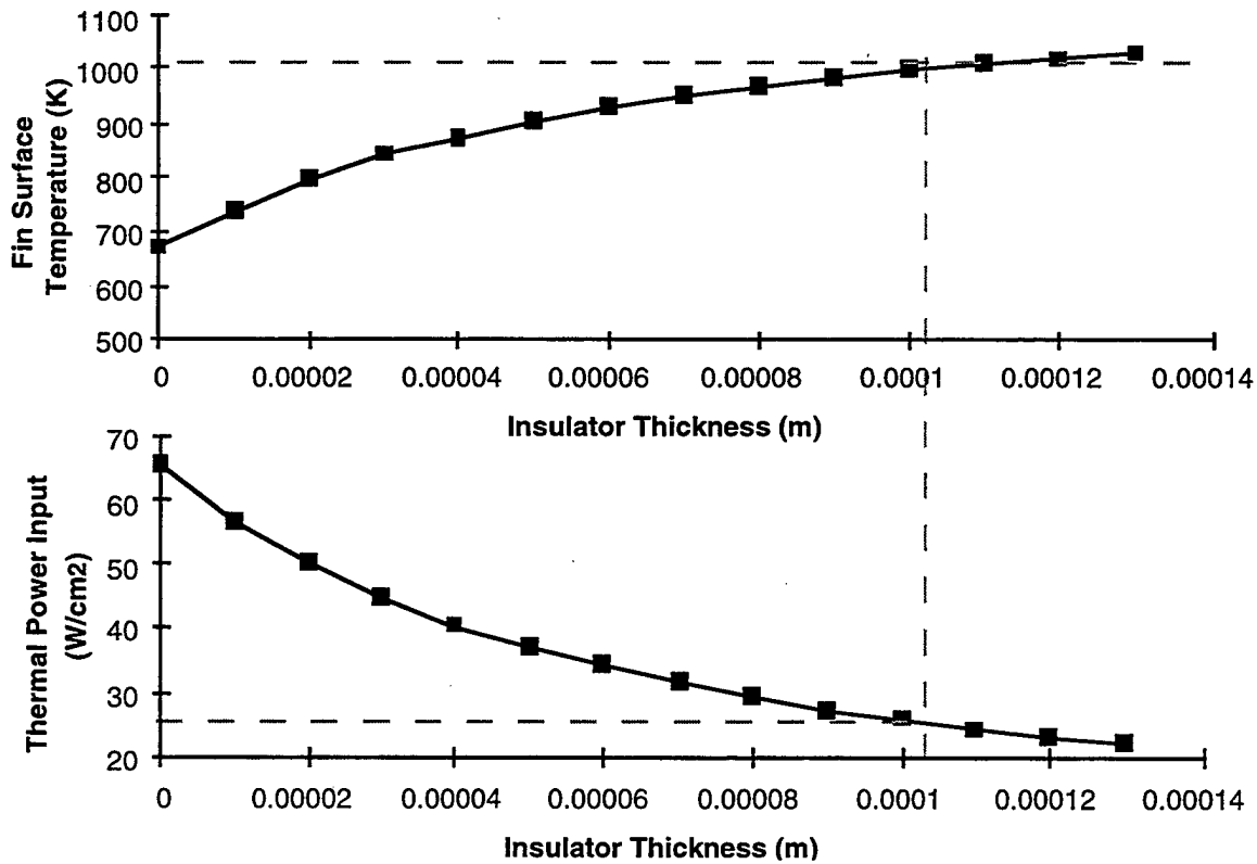
Figure 13. Fin skin temperature and thermal input heat flux as a function of insulator thickness.
