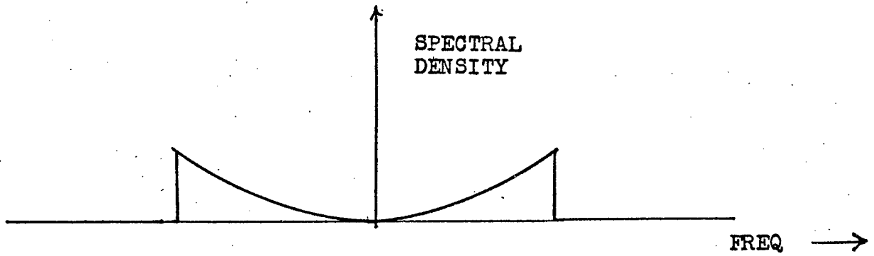
FIGURE 6b POWER SPECTRAL DENSITY AFTER NULLING
