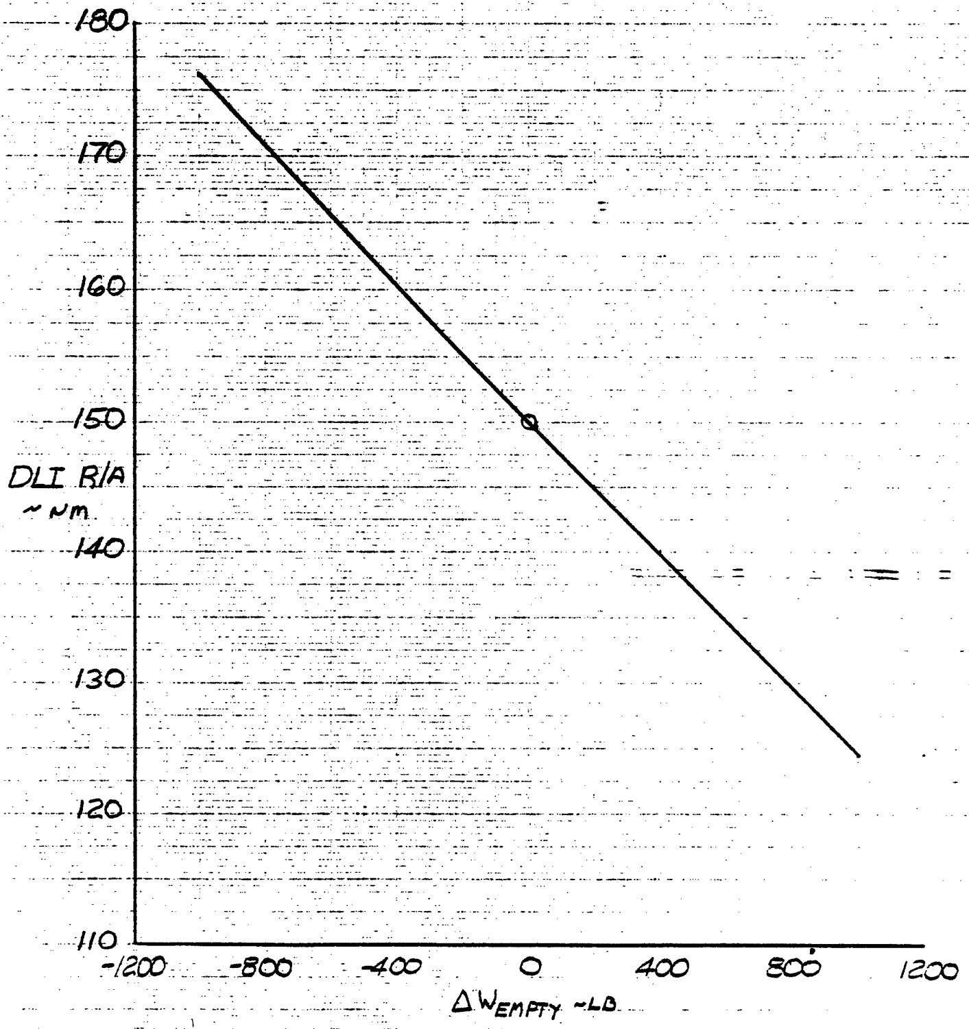
Figure 46. Lift + Lift/Cruise DLI Radius of Action Sensitivity to Empty Weight
