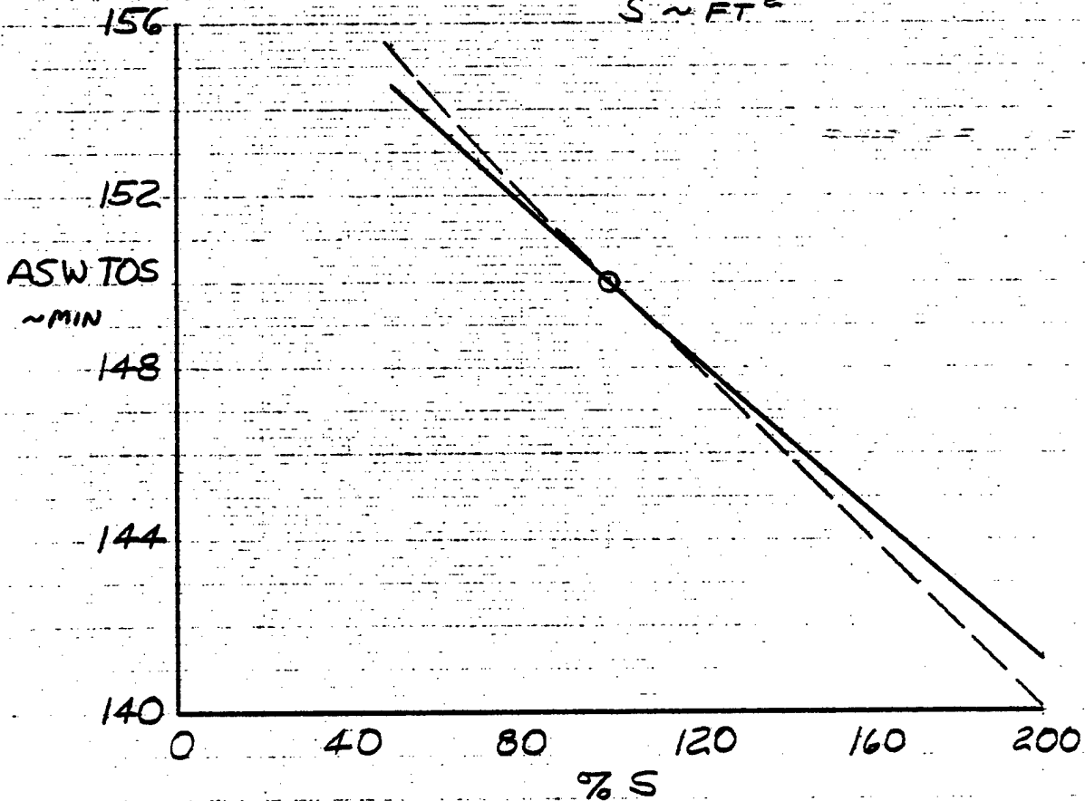
Figure 37. Tandem Fan ASW Time on Station Sensitivity to Tail Size Variation
