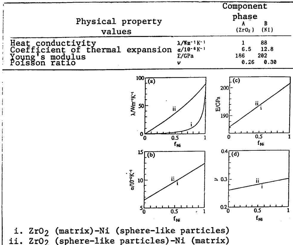
Figure 10. Input Data and Calculation Result of Physical Property Values for ZrO_2 -Ni Group
