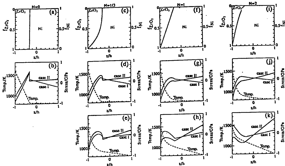
Figure 11. Example of Thermal Stress for ZrO_2 -Ni Group FGM (steady state elasticity analysis)
