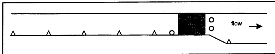
Figure 9. Plan view of a section of the McNary juvenile bypass channel showing radio-telemetry antennae locations. Antennae are indicated as triangles for general monitoring and rate of travel, or circles for specific monitoring near the test devices (shaded area). General monitoring antennae upchannel from the test devices were spaced 27 m apart. Drawing not to scale.
