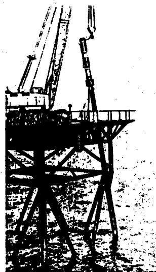
Fig. 3. The MEM-30 Hammer During Industrial Testing When a Pile on the Housing Unit of the Golitsina-4 Platform Was Driven
