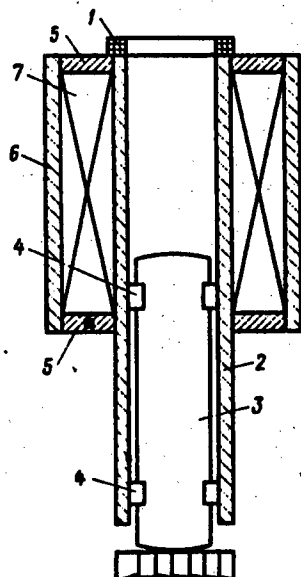
Fig. 2. Single-Acting Hammer
