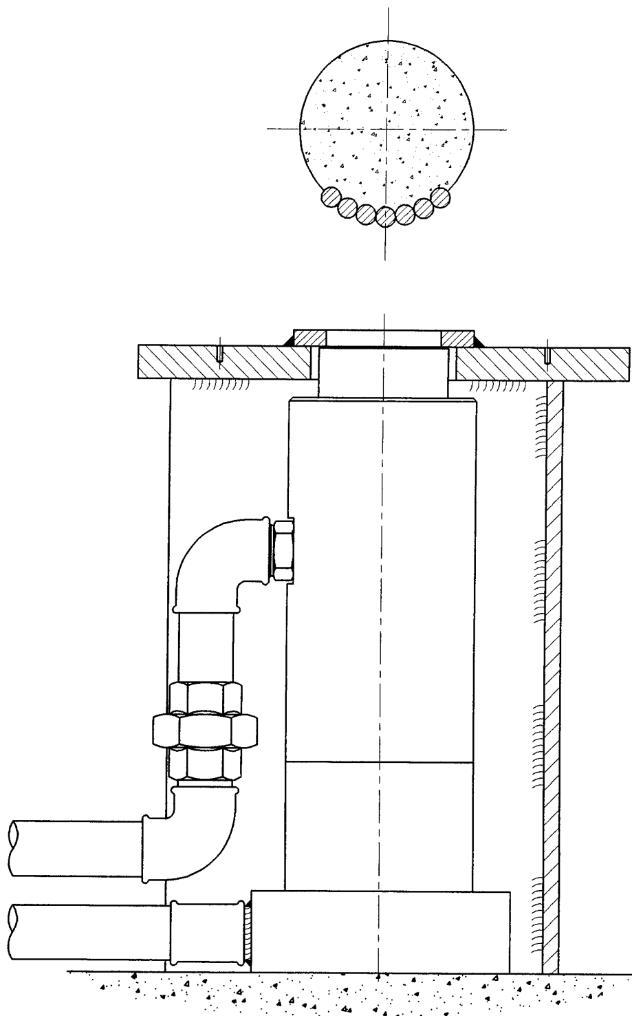
Figure 3.4: Experimental set-up.
