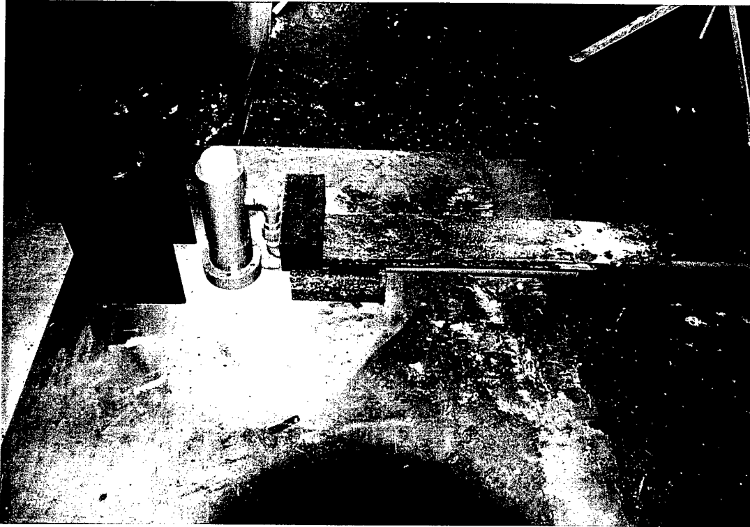
Figure 4.1: Experimental set-up. The impulse plug is placed vertically on the concrete floor of the bunker. The 'table' with the plate which smooths the blast wave is standing left of the impulse plug. The tubing which carries the instrumentation cables away are extra protected by steel bricks and plates (980109-17).
