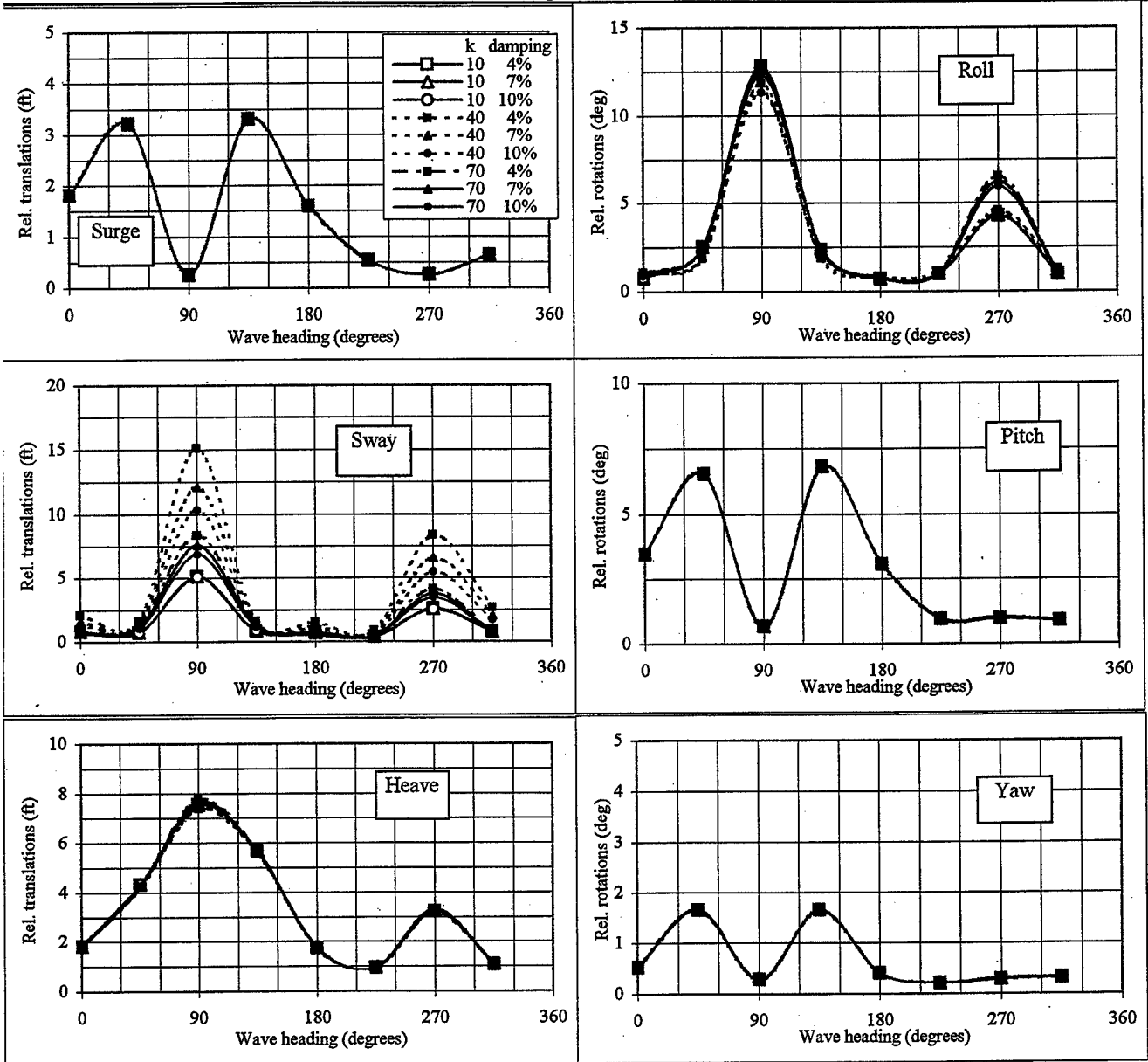
Figure 16. Relative motion of the T-ACS as seen from the ACB lighter in random seaway (ss4).
