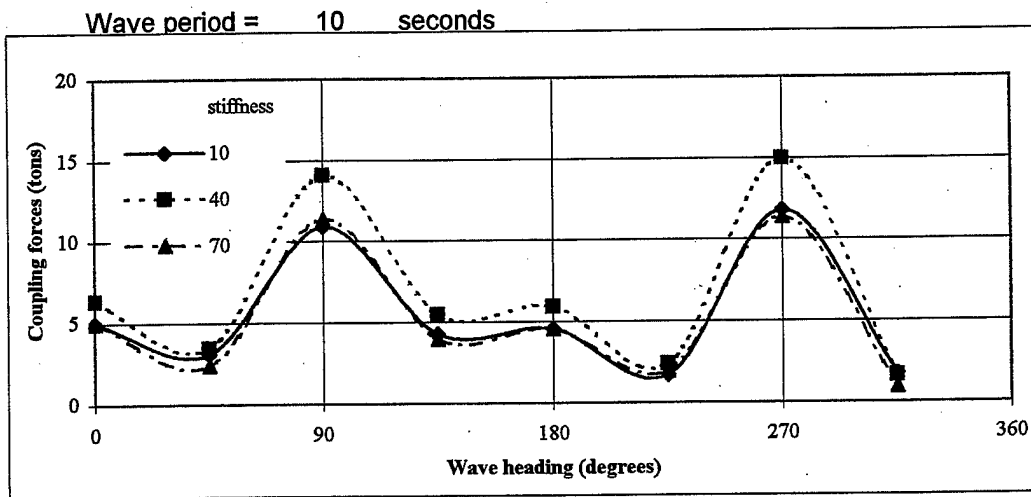
Figure 19. Coupling forces versus wave heading.
