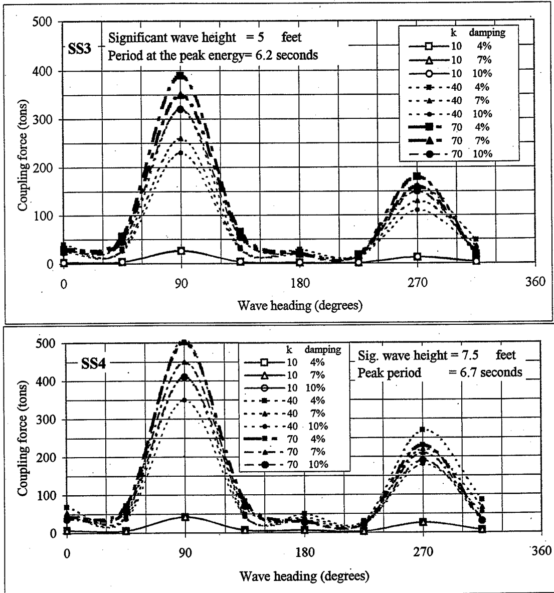
Figure 20. Coupling forces in random seaways ss3 and ss4.
