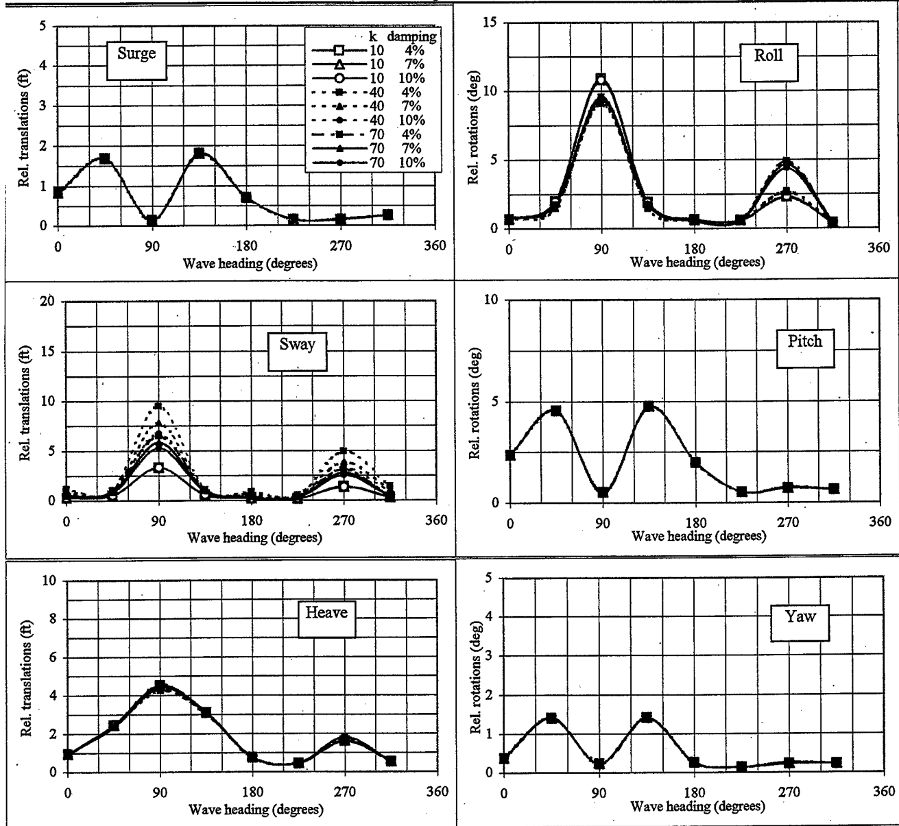
Figure 15. Relative motion of the T-ACS as seen from the ACB lighter in random seaway (ss3).
