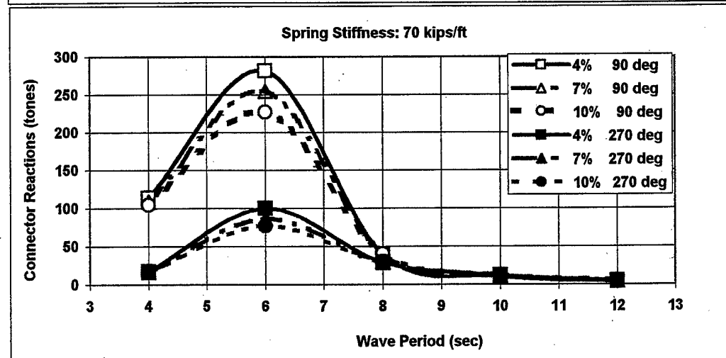
Figure 18. Coupling force versus wave period.
