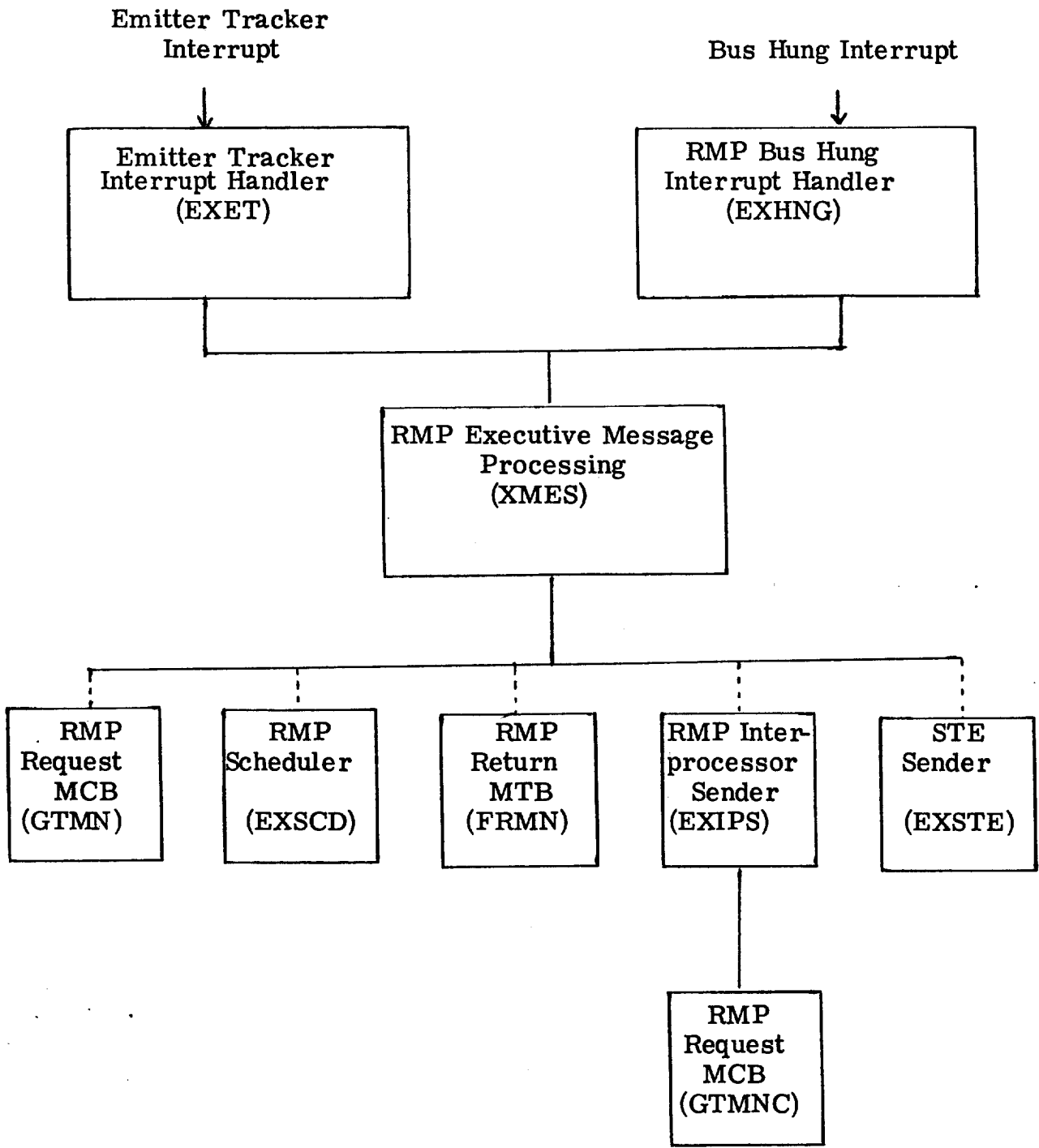
Interface Description (RMP Executive with RMP Interrupts)
