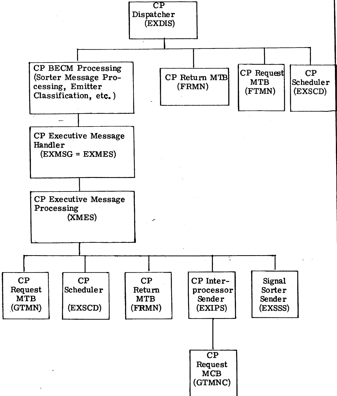
Interface Description (CP Executive with CP BECM, RMP EXEC, AP EXEC and SS)
