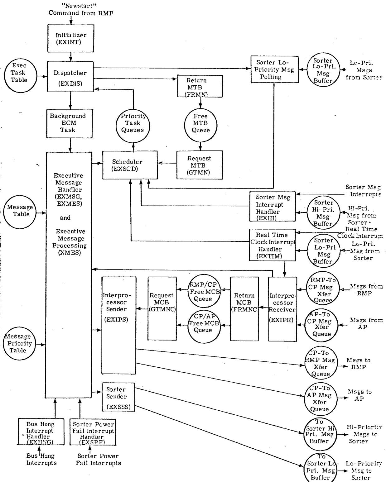
Figure 2. CP EXEC Block Diagram
