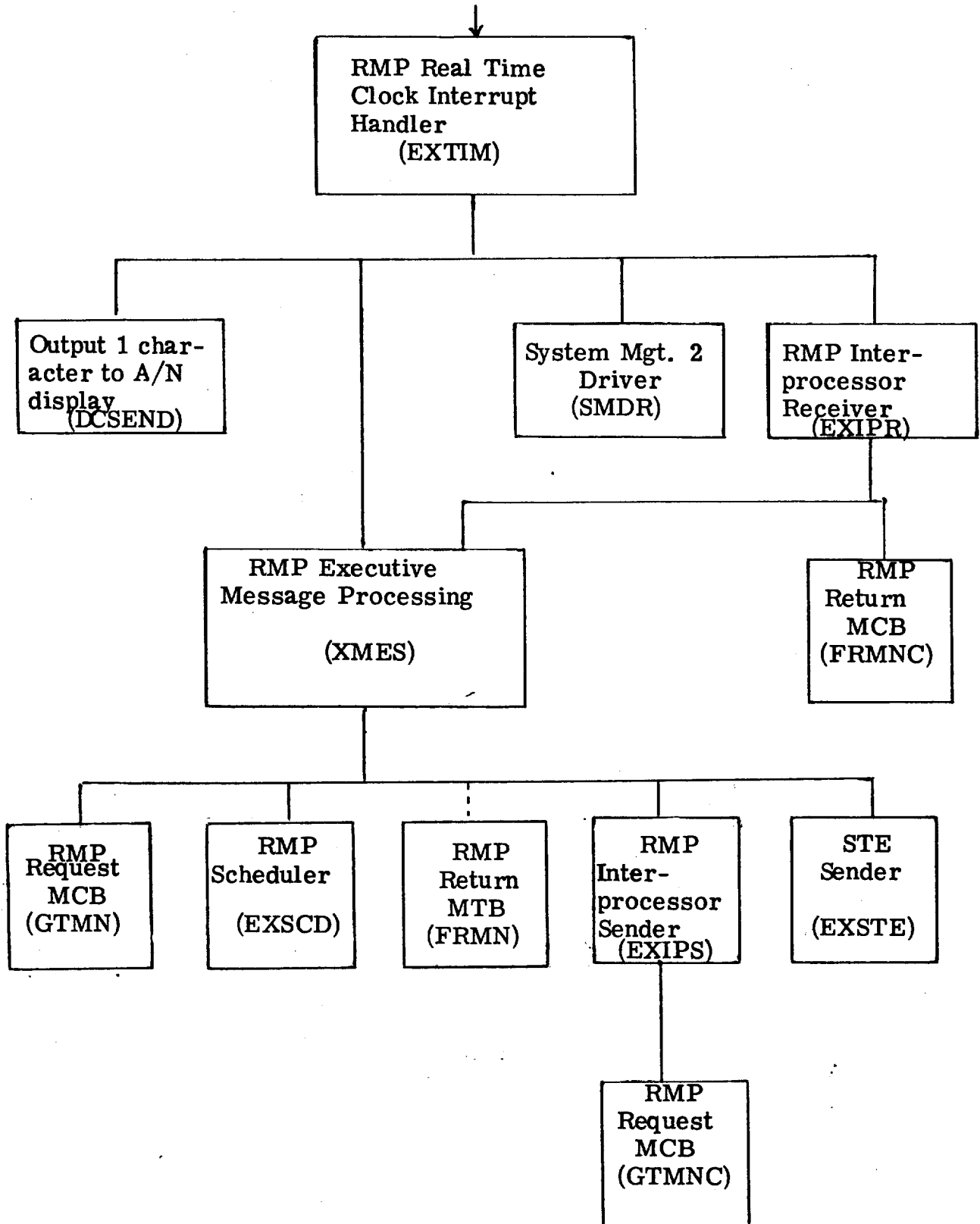
Interface Description (RMP Executive with RMP Interrupts)
