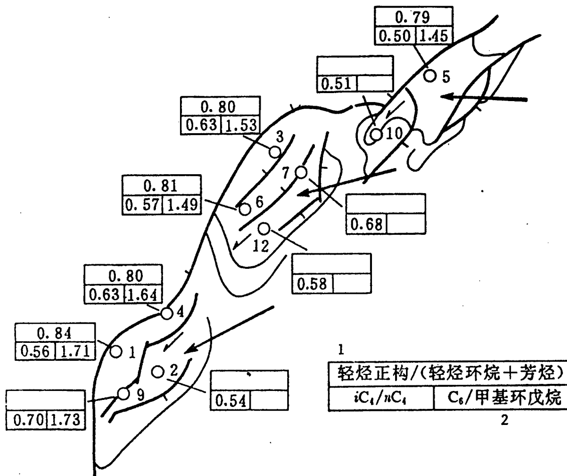
Figure 2. Direction of Natural Gas Migration in Jingchuan 20-2 Gas Field (According to the Bohai Sea Petroleum Company Research Academy)
