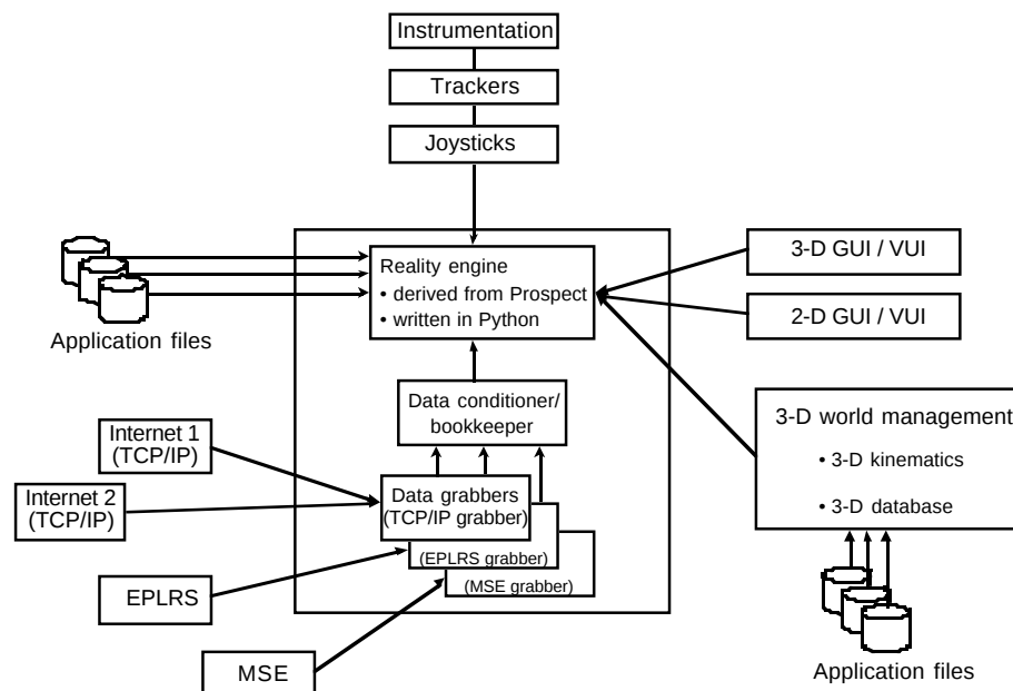
Figure 1. Program architecture.
