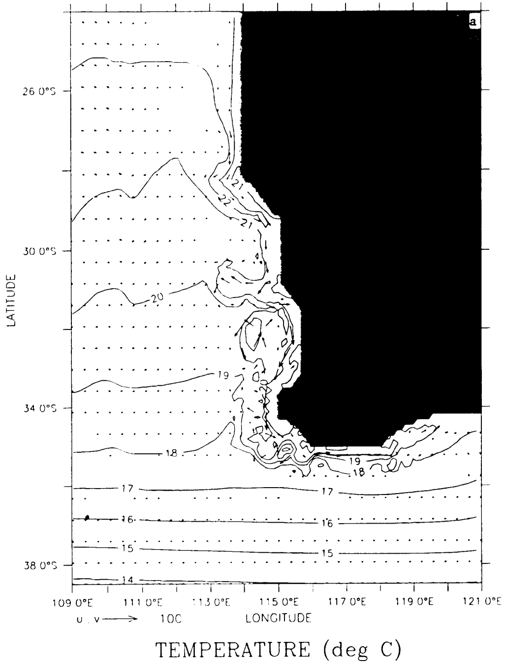
Figure 15. Temperature contours and velocity vectors at 10 m depth at days (a) 45, (b) 180, and (c) 360 of Experiment 3. Contour interval is 1°C; maximum velocity vector is 100 cm/s.
