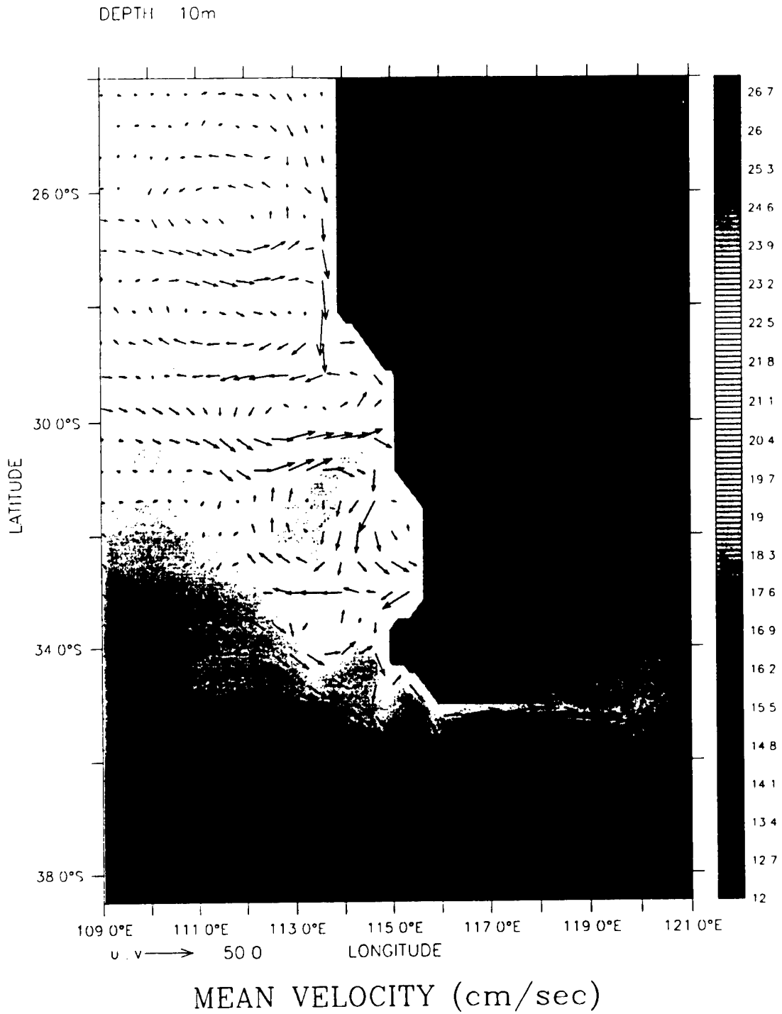
Figure 7. Mean temperature and velocity vectors at 10 m depth averaged for days 90 to 270 of Experiment I. Contour interval is 0.1°C with colder waters in the south end of model domain; maximum velocity vector is 50 cm/s.
