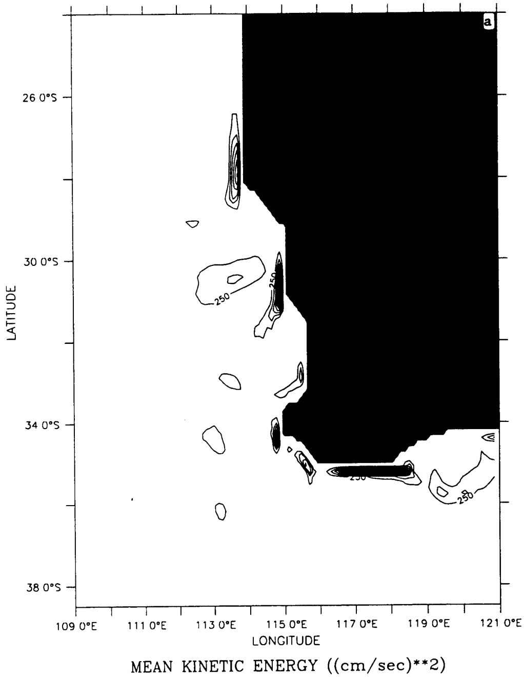
Figure 8. Horizontal maps at 10 m depth of (a) mean kinetic energy (MKE) and (b) eddy kinetic energy (EKE) averaged for days 90 to 270 of Experiment 1. Contour interval is 250 \text{ cm}^2/\text{s}^2 .
