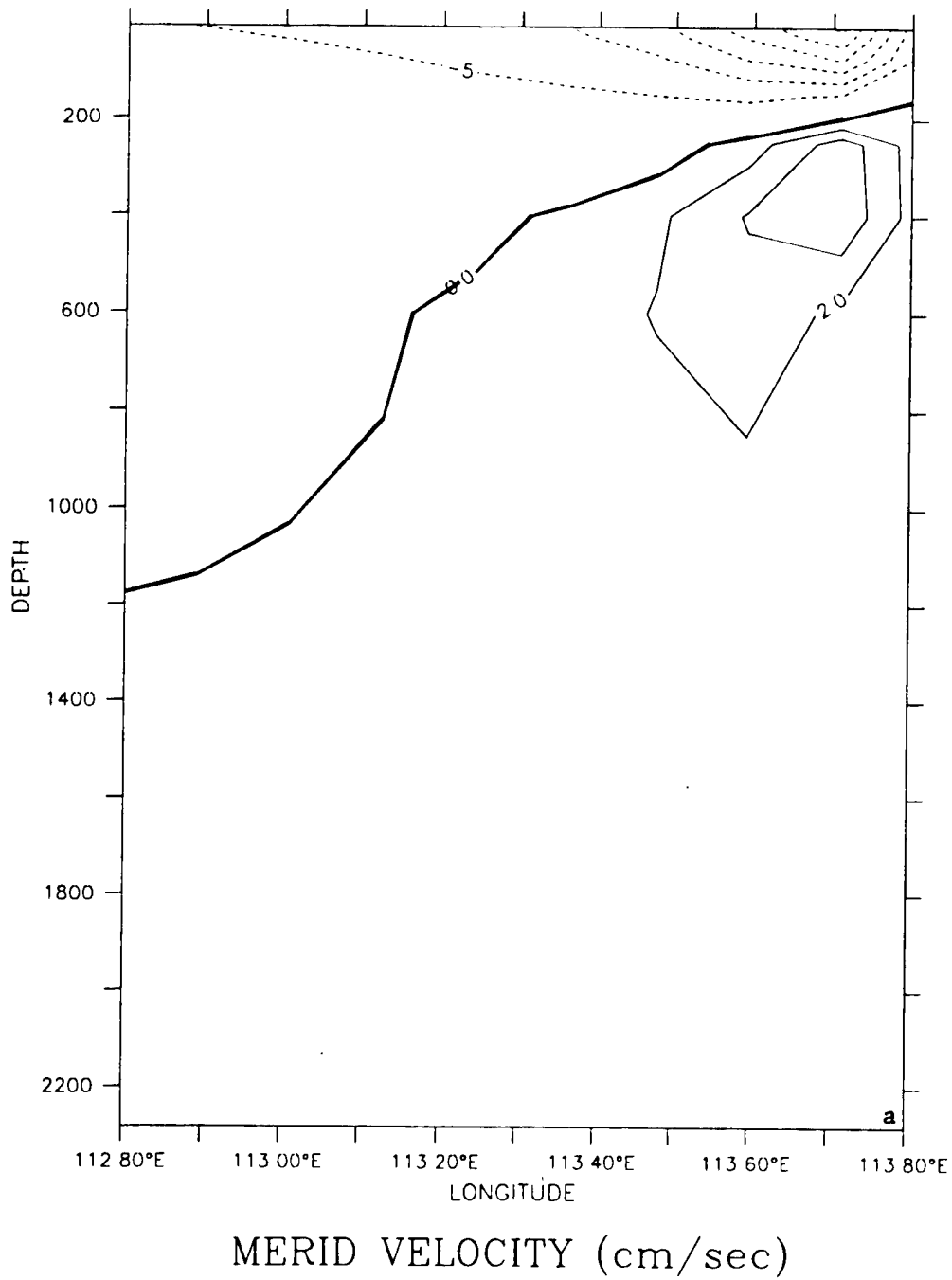
Figure 30. Cross-shore section of meridional velocity ( v ) for day 9 at (a) \sim 26^\circ S, and (b) 32^\circ S of Experiment 6. The contour interval is 5.0 cm/s for poleward (dashed line) flow and 2.0 cm/s for equatorward (solid line) flow.
