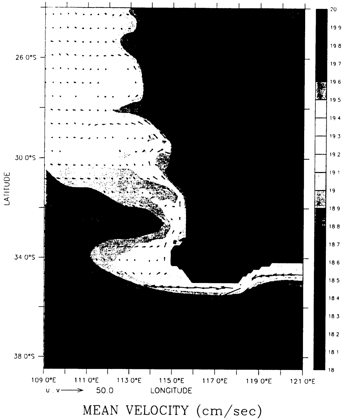
Figure 13. Mean temperature and velocity vectors at 10 m depth averaged for days 90 to 270 of Experiment 2. Contour interval is 0.1°C with colder waters in the coastal region of model domain; maximum velocity vector is 50 cm/s
