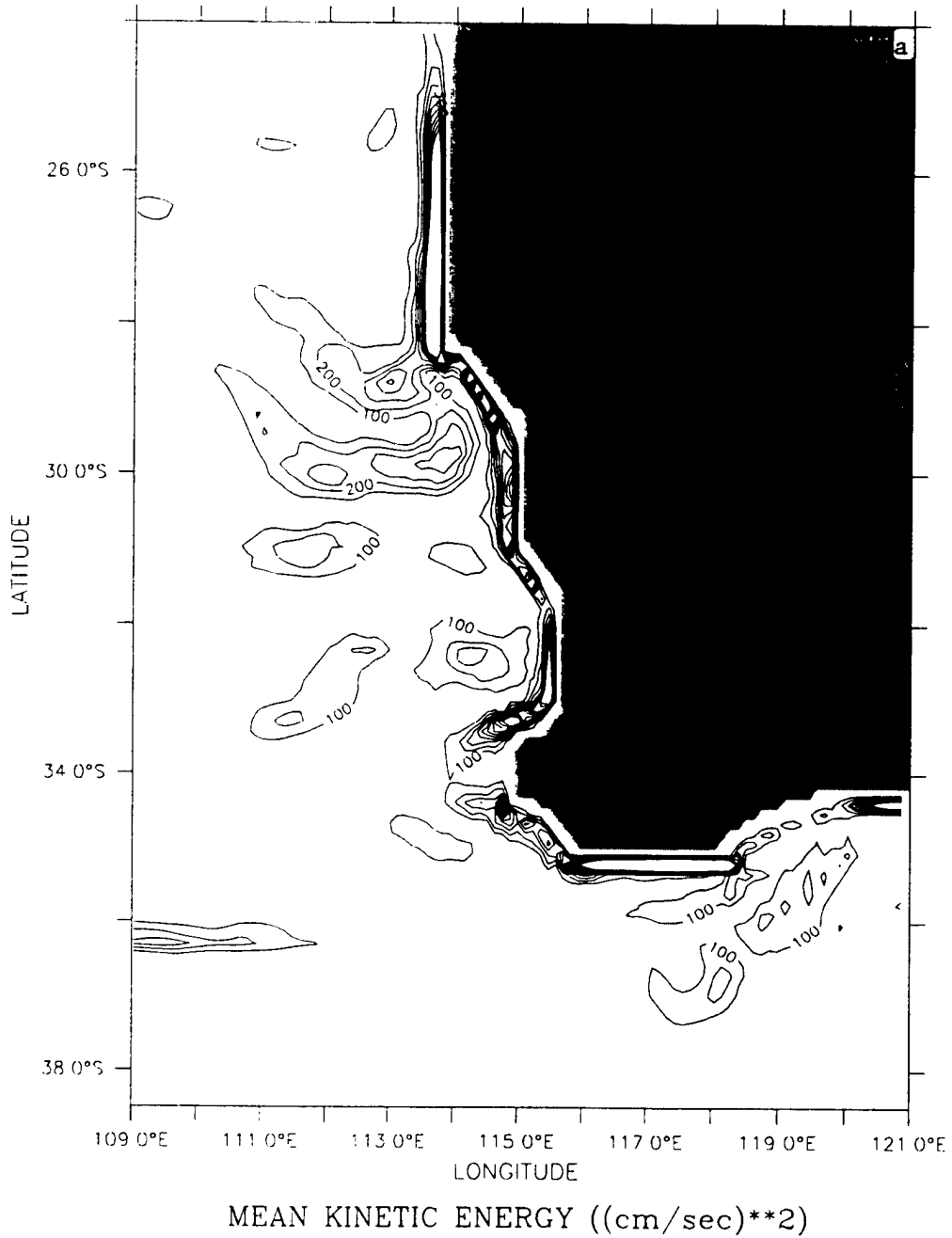
Figure 27. Horizontal maps at 10 m depth of (a) mean kinetic energy (MKE) and (b) eddy kinetic energy (EKE) averaged for days 90 to 270 of Experiment 5. Contour interval is 100 \text{ cm}^2/\text{s}^2 in (a) and 250 \text{ cm}^2/\text{s}^2 in (b).
