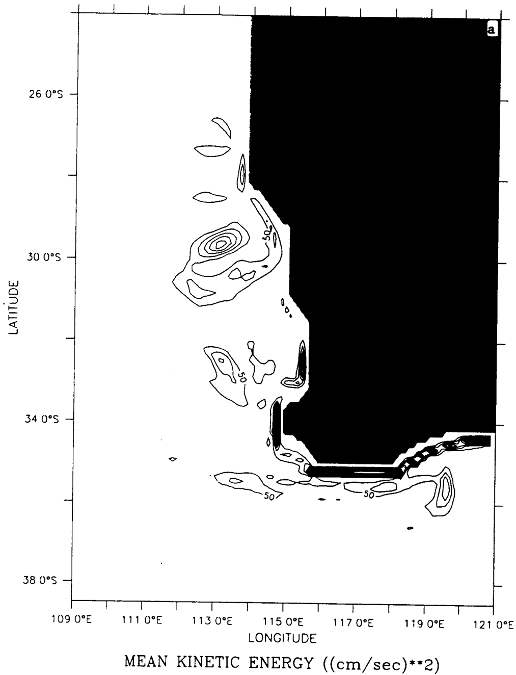
Figure 18. Horizontal maps at 10 m depth of (a) mean kinetic energy (MKE) and (b) eddy kinetic energy (EKE) averaged for days 90 to 270 of Experiment 3. Contour interval is 50 \text{ cm}^2/\text{s}^2 in (a) and 100 \text{ cm}^2/\text{s}^2 in (b).
