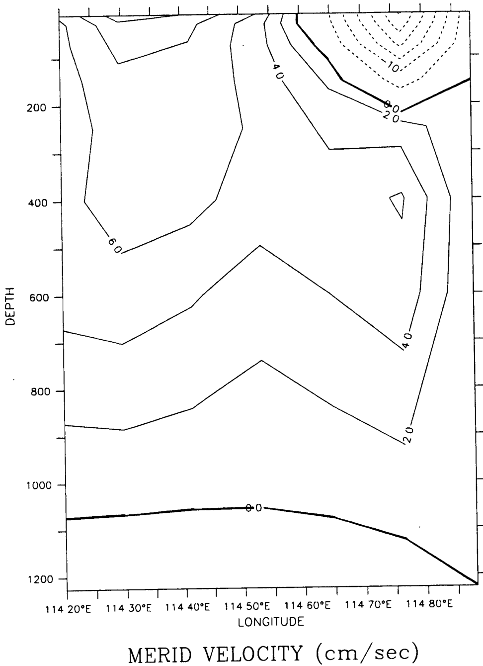
Figure 16. Cross-shore section of meridional velocity ( v ) at 34^{\circ} S (off Cape Leeuwin), for day 180 of Experiment 3. The contour interval is 5.0 cm/s for poleward (dashed line) flow and 2.0 cm/s for equatorward (solid line) flow.
