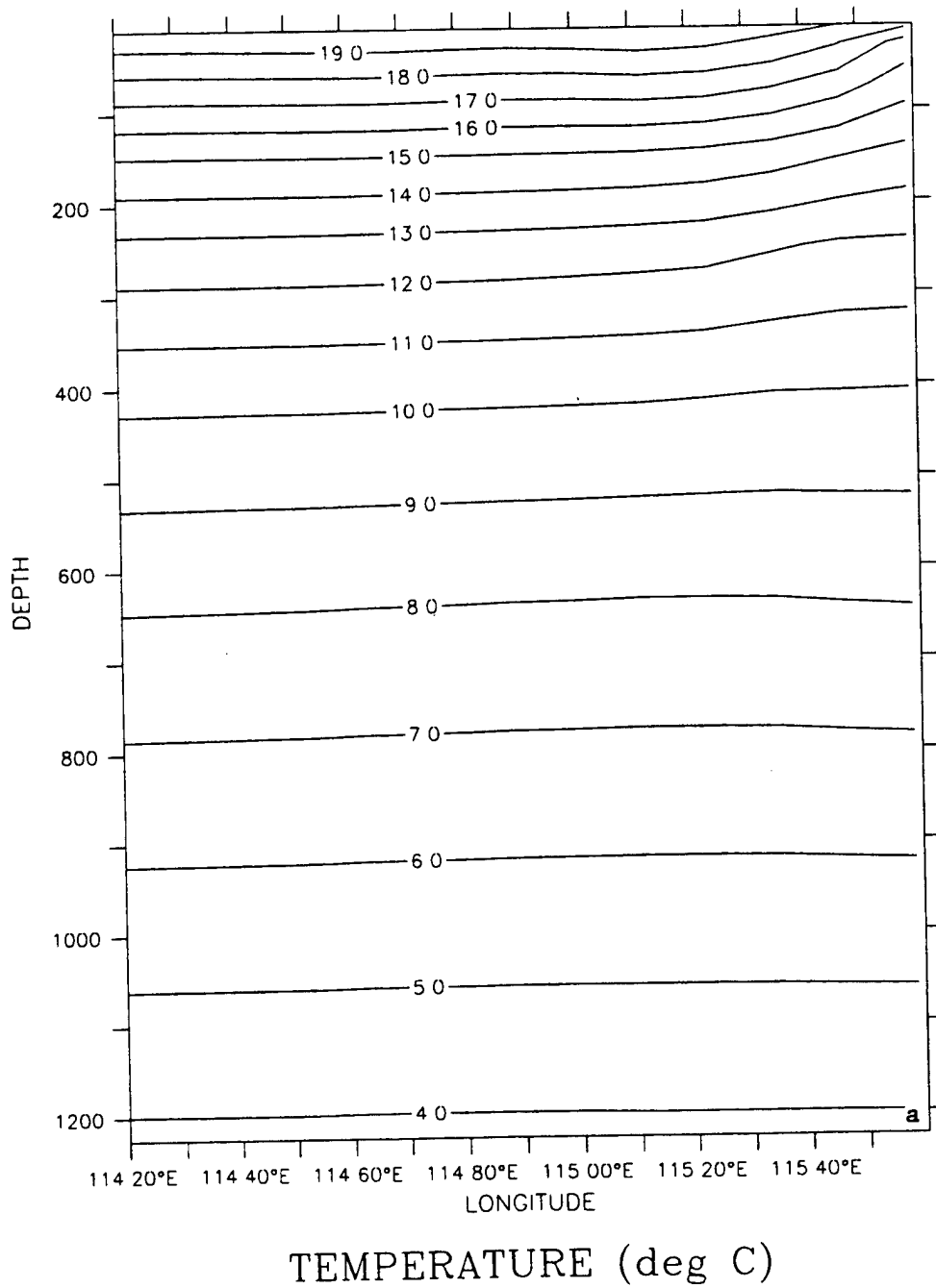
Figure 11. Cross-shore sections of temperature at ~ 32°S (near Fremantle) at days (a) 90, (b) 180, (c) 360 of Experiment 2. Contour interval is 1°C.
