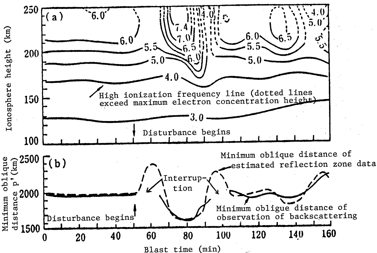
Figure 2. Changes in minimum oblique distance of backscattered echoes (b) and their disturbance of reflection zone ionosphere (a)
