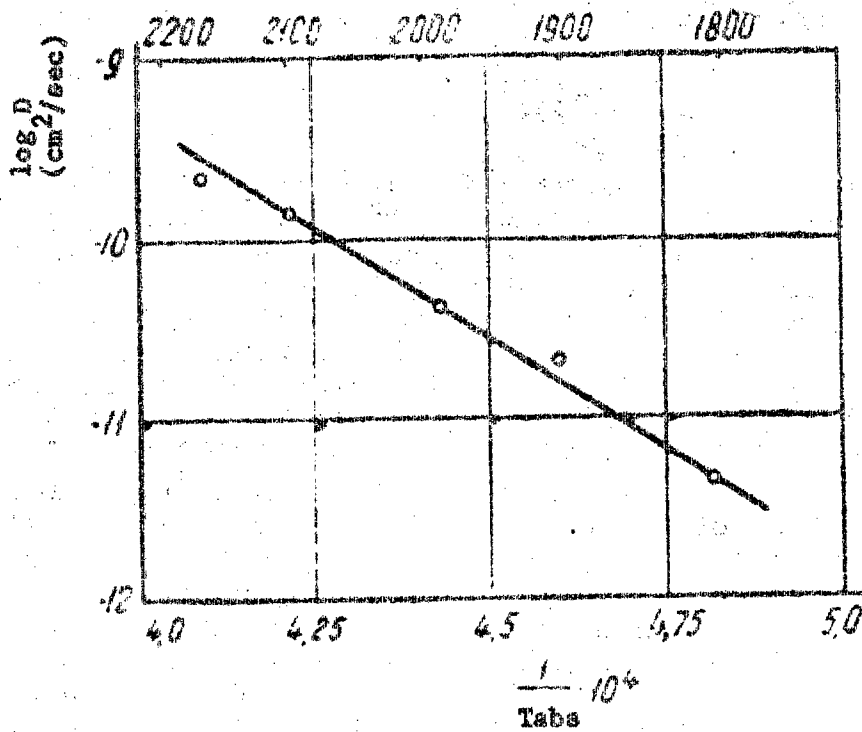
Fig. 1. Self-diffusion coefficients of melted molybdenum vs temperature.
