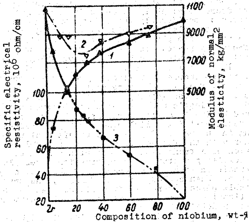
Fig. 3. Elastic modulus and specific electrical resistivity of hardened zirconium alloys with niobium: 1- alloys hardened in water from 1100^\circ\text{C} ; 2 - alloys annealed for 80 hours at 525^\circ\text{C} ; 3 - specific electrical resistivity.
